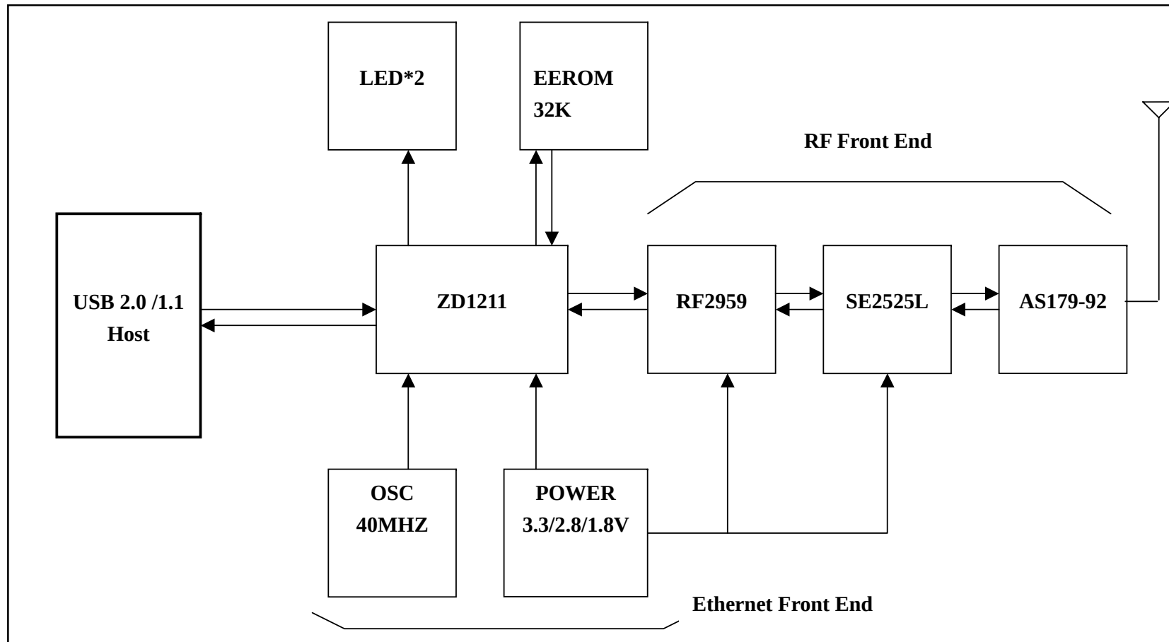
WN4320Z Functional Block Diagram
