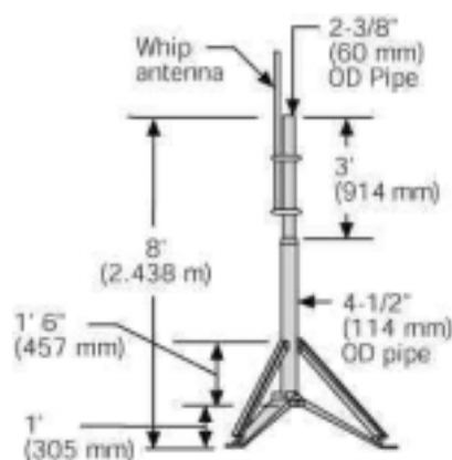
Tripod Mount
