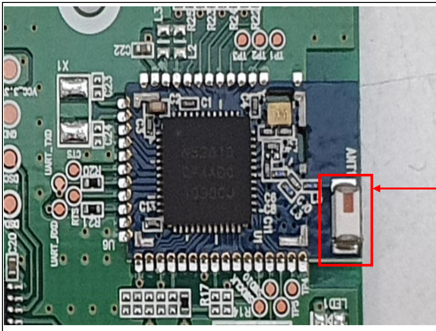
Chip Antenna
