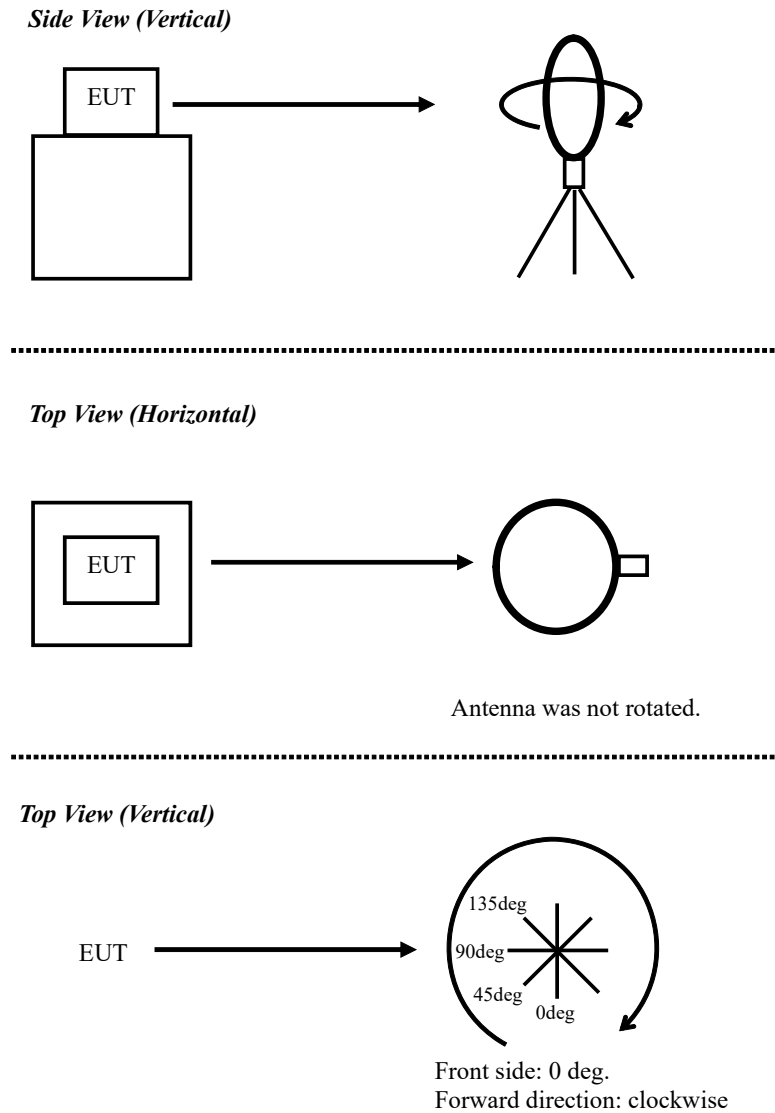
Figure 1: Direction of the Loop Antenna
