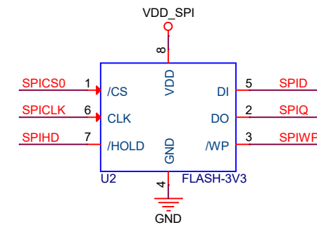
ESP32-S3-WROOM-1(pin-out)
