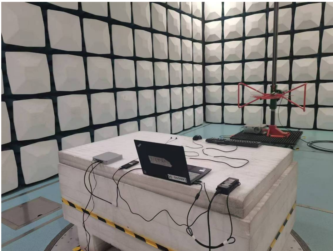
Radiated Emission 30M-1GHz Rear View
