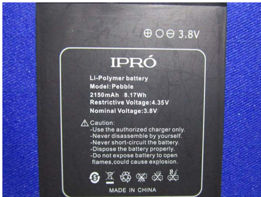
EUT –Battery Top Label View
