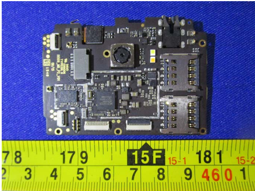
EUT –Main Board Bottom Ushield View
