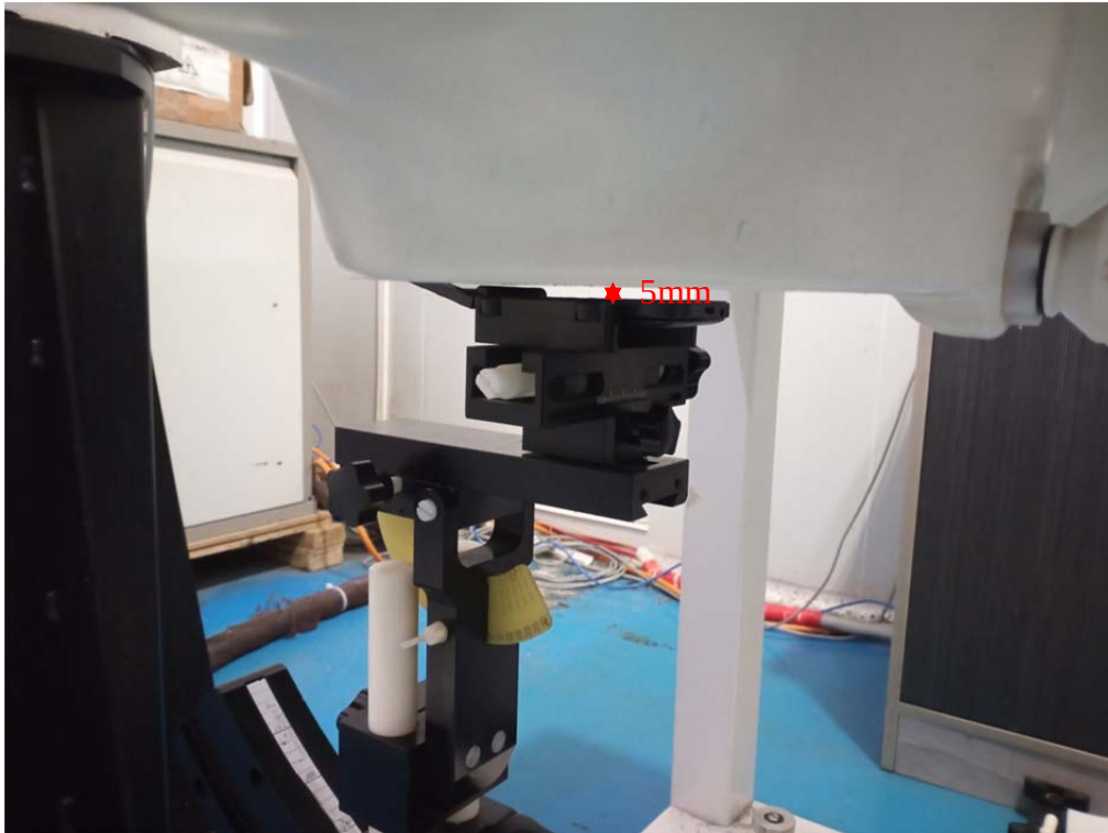
Body Front (closed-cover) Setup Photo(5mm)
