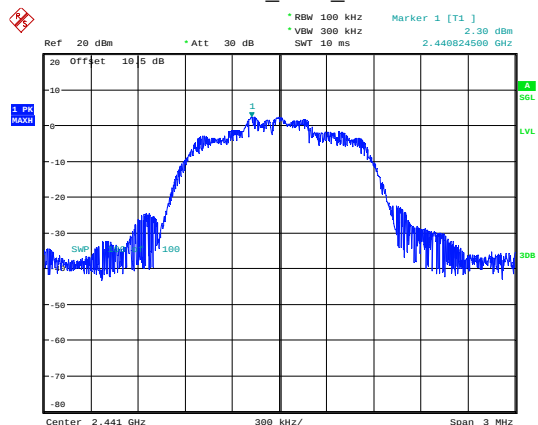
3EDR_DH1_Middle
