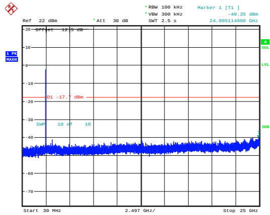
3EDR_DH1_Middle
