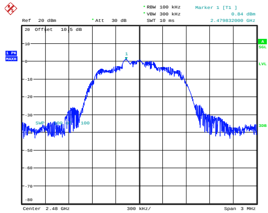
3EDR_DH1_High
