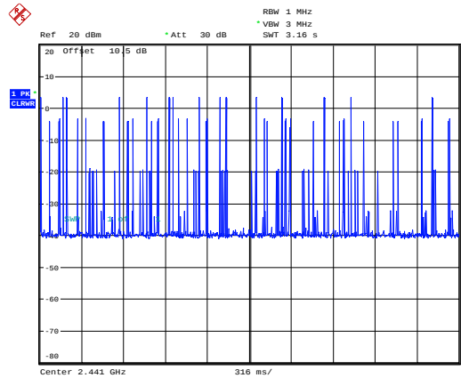
BDR_DH3_Hopping
