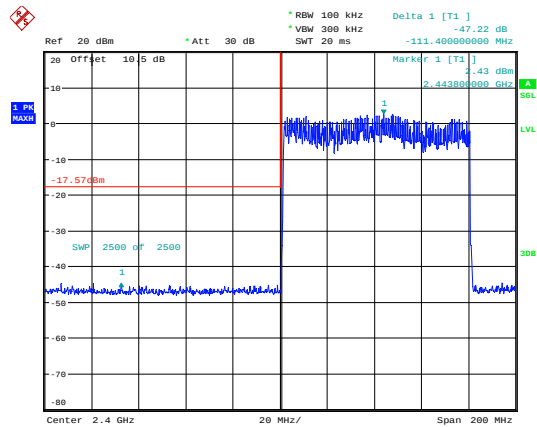
3EDR_DH1_Hopping_Lower
