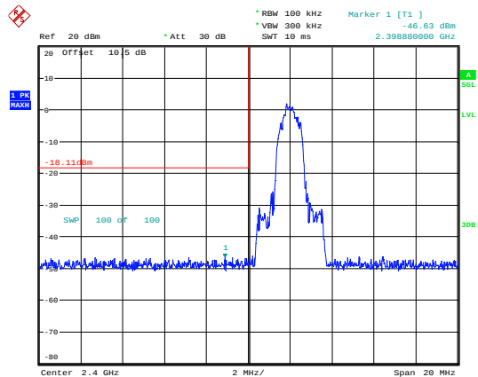
3EDR_DH1_Low
