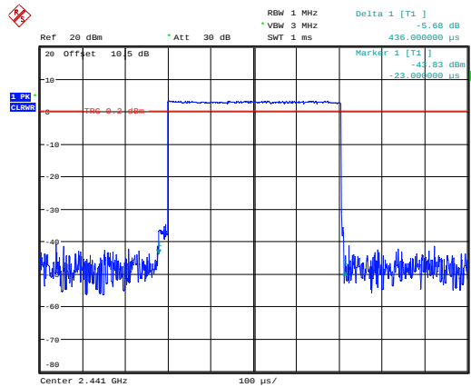
BDR_DH1_Hopping
