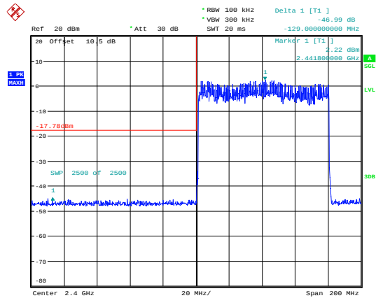
2EDR_DH1_Hopping_Lower
