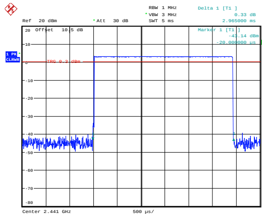
BDR_DH5_Hopping
