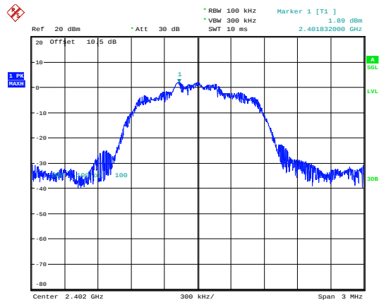
3EDR_DH1_Low
