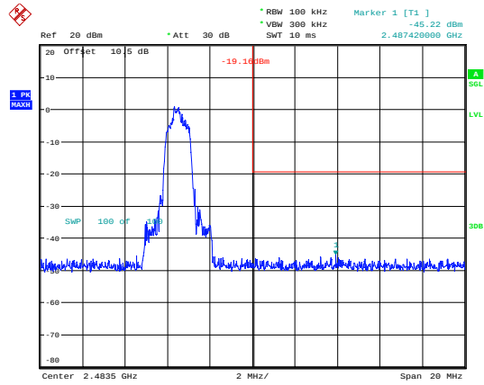
3EDR_DH1_High
