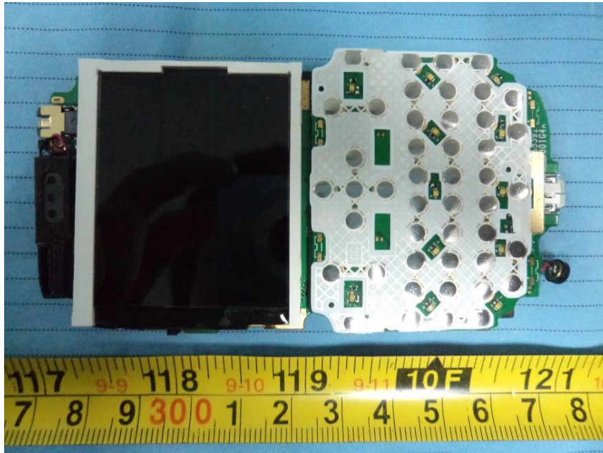
EUT – Main Board Top with LCD&Keyboard View
