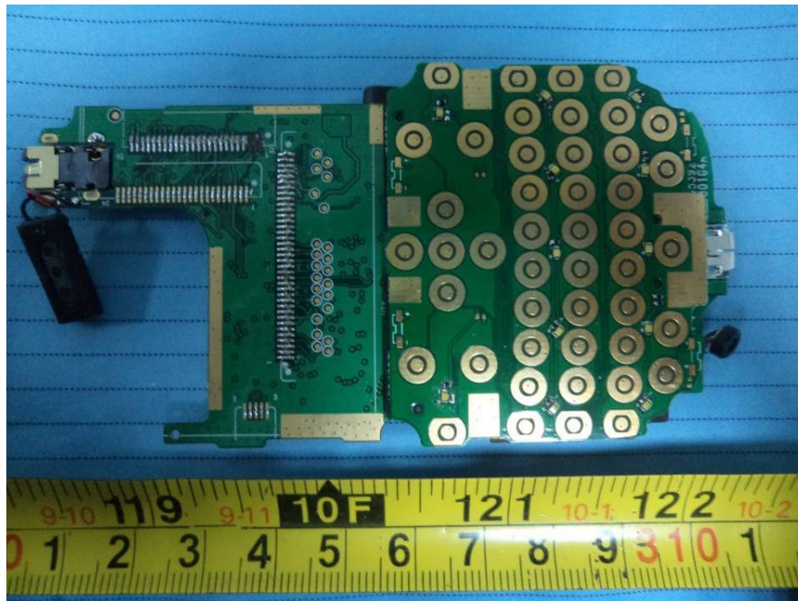
EUT – Main Board Top with Keyboard View 2
