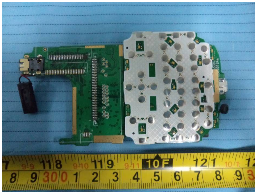
EUT – Main Board Top with Keyboard View 1
