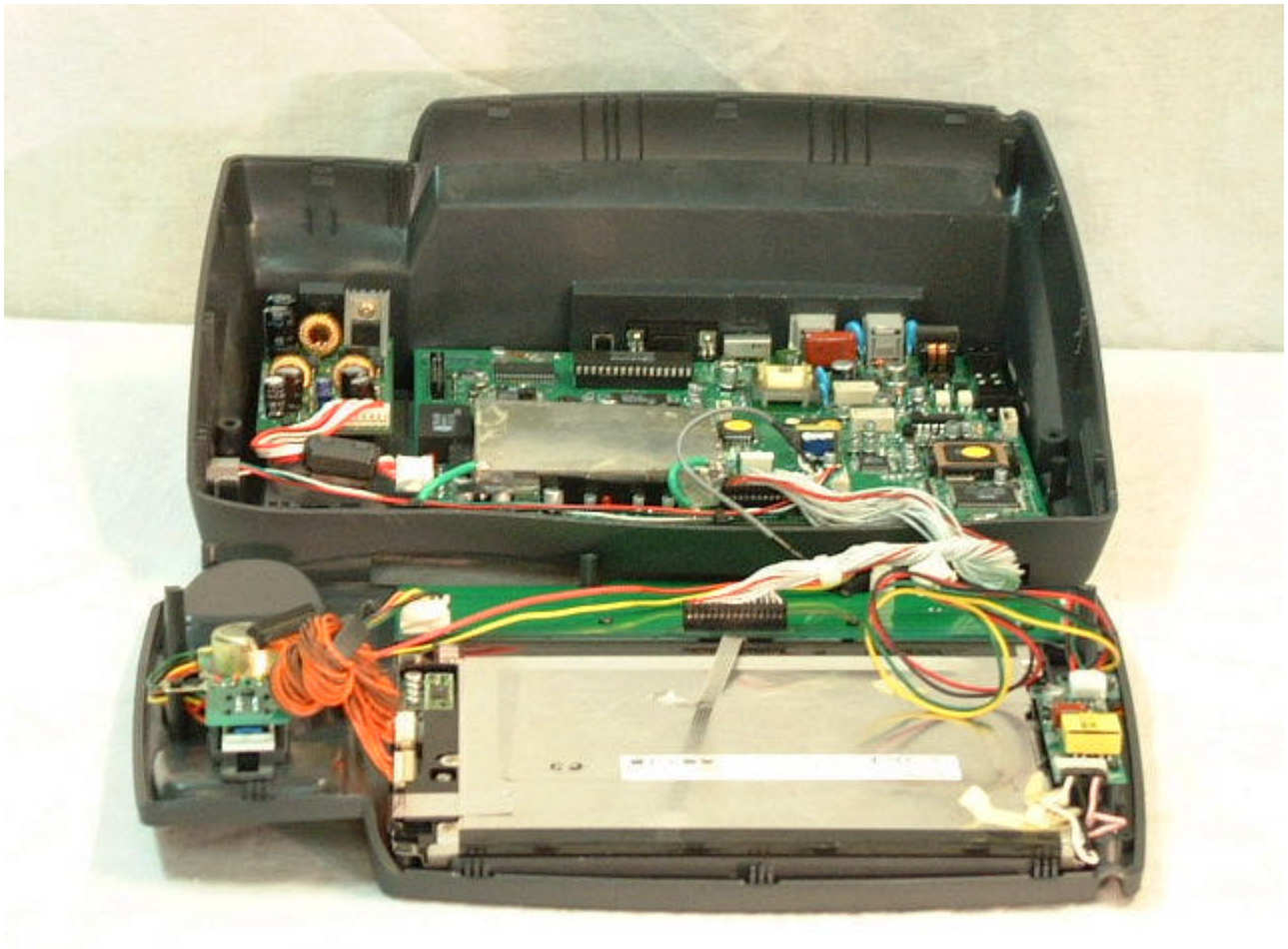
<INTERNAL VIEW OF E.U.T>
