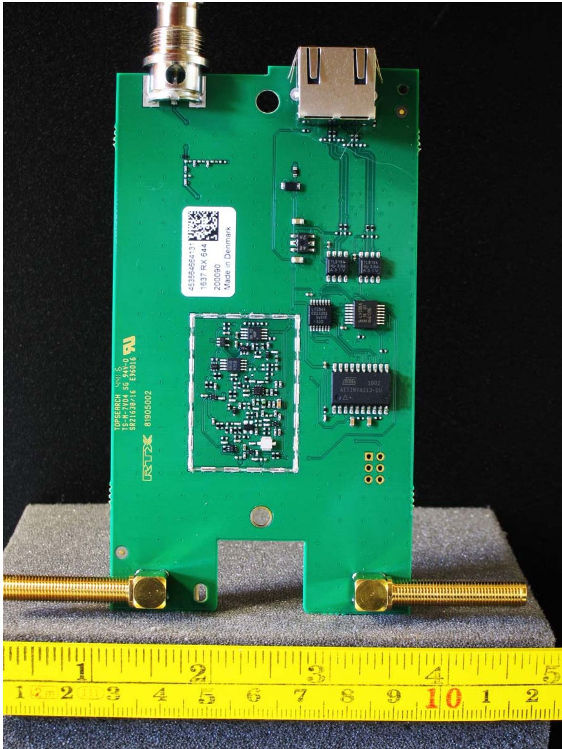
PCB Front Shield Removed
