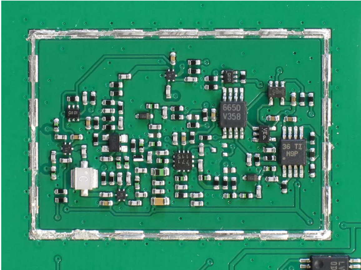
Transmitter Section close up
