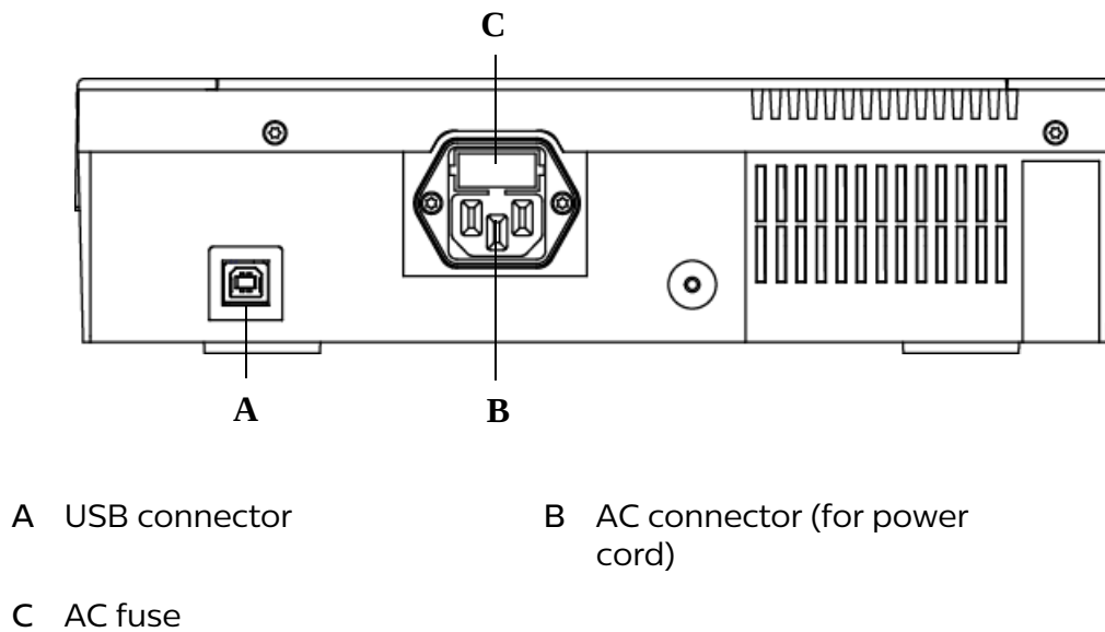
Figure C-4 ST80i Thermal Printer Rear Panel
