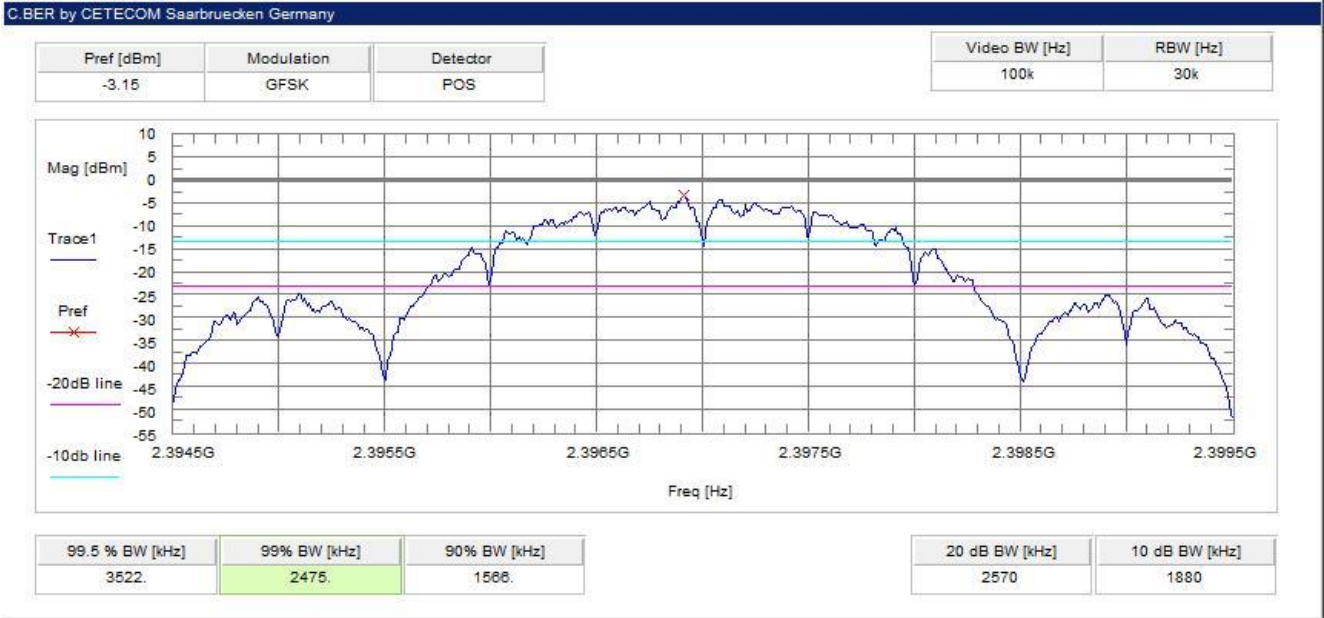
Plot 5: highest channel, upper band
