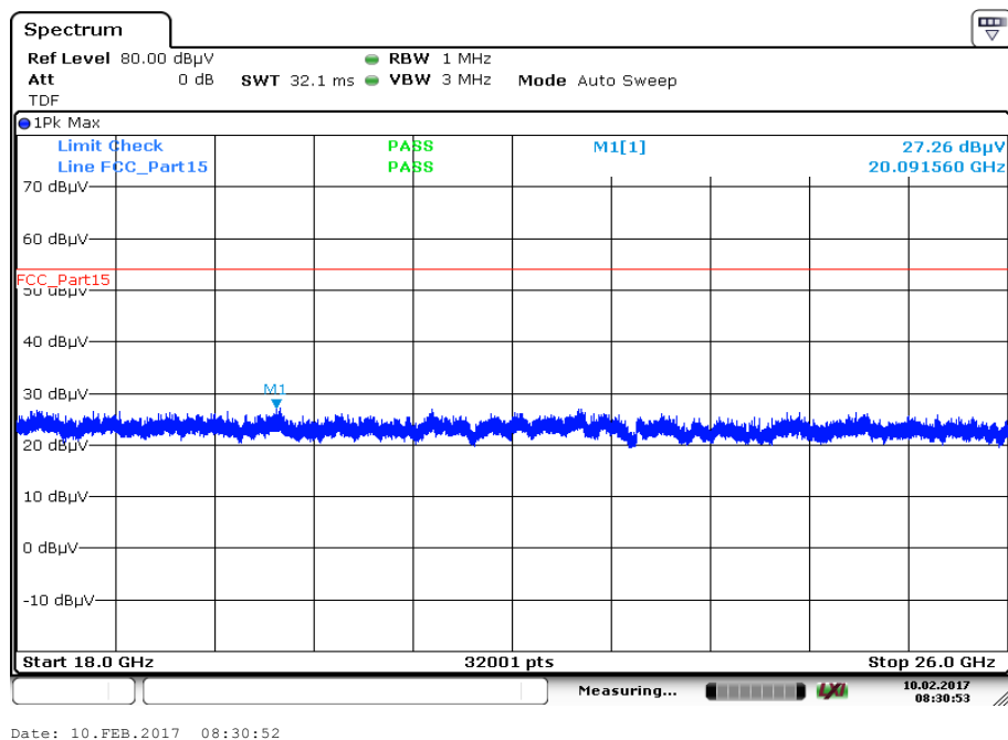
Plot 5: 18 GHz – 26 GHz, antenna horizontal/vertical
