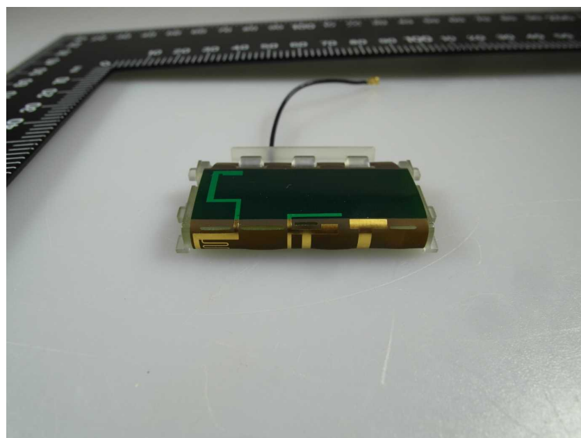
Photo 14: Antenna Apollo
