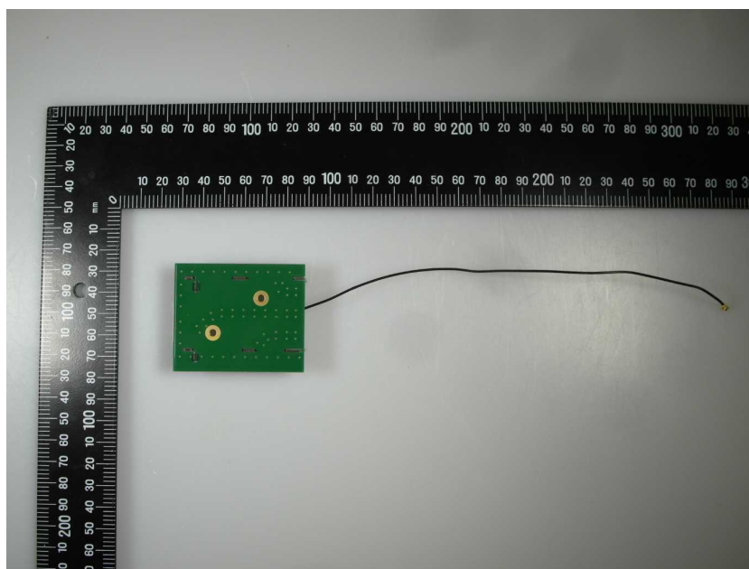
Photo 18: Antenna Delphi
