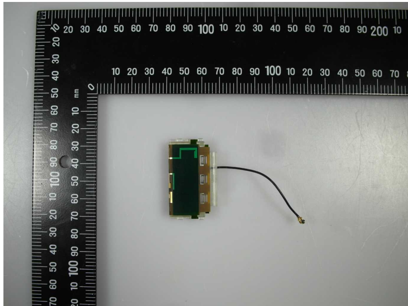
Photo 11: Antenna Apollo
