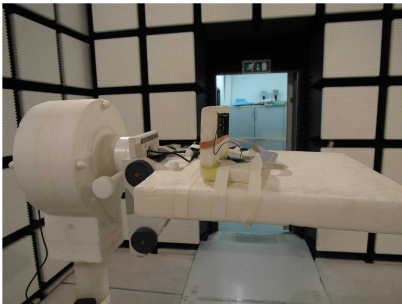
Photo 14: Setup Delphi
