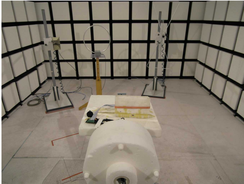
Photo 3: Setup Apollo
