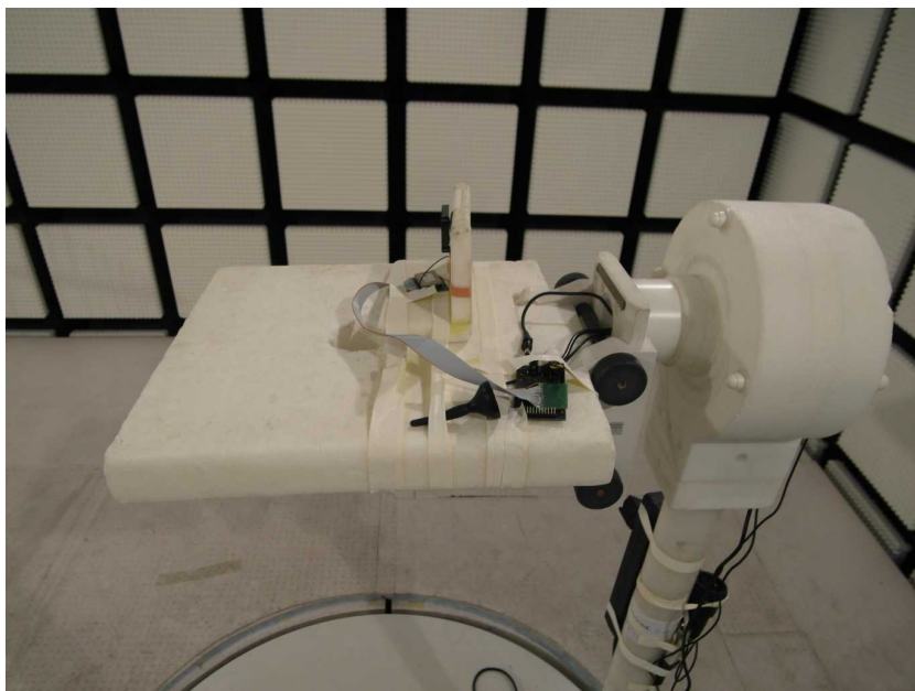
Photo 12: Setup Delphi
