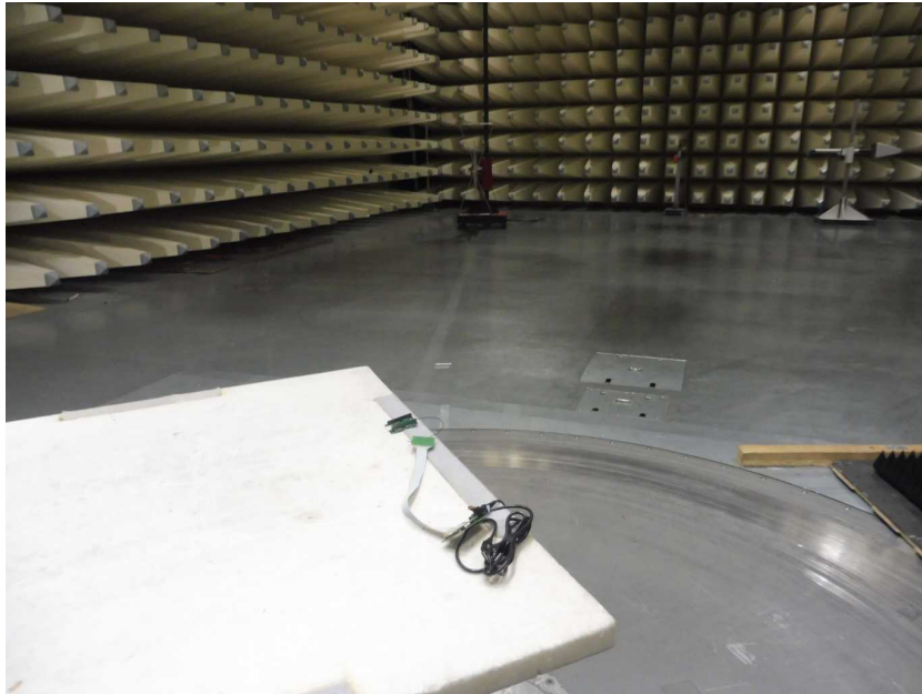
Photo 21: Setup Delphi
