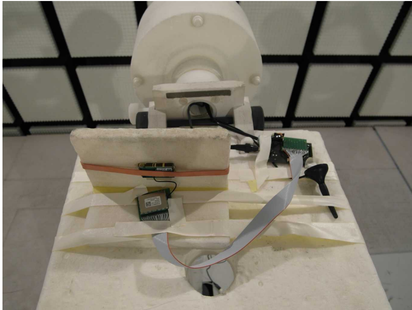
Photo 5: Setup Apollo
