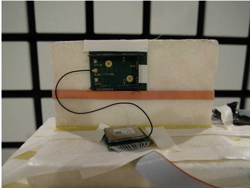
Photo 15: Setup Delphi
