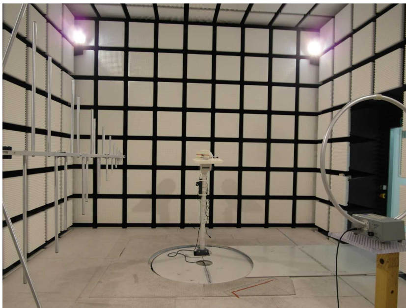
Photo 8: Setup Apollo
