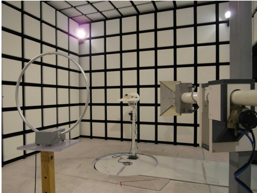
Photo 17: Setup Delphi
