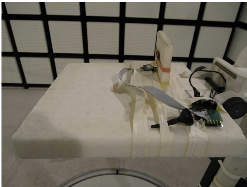
Photo 2: Setup Apollo
