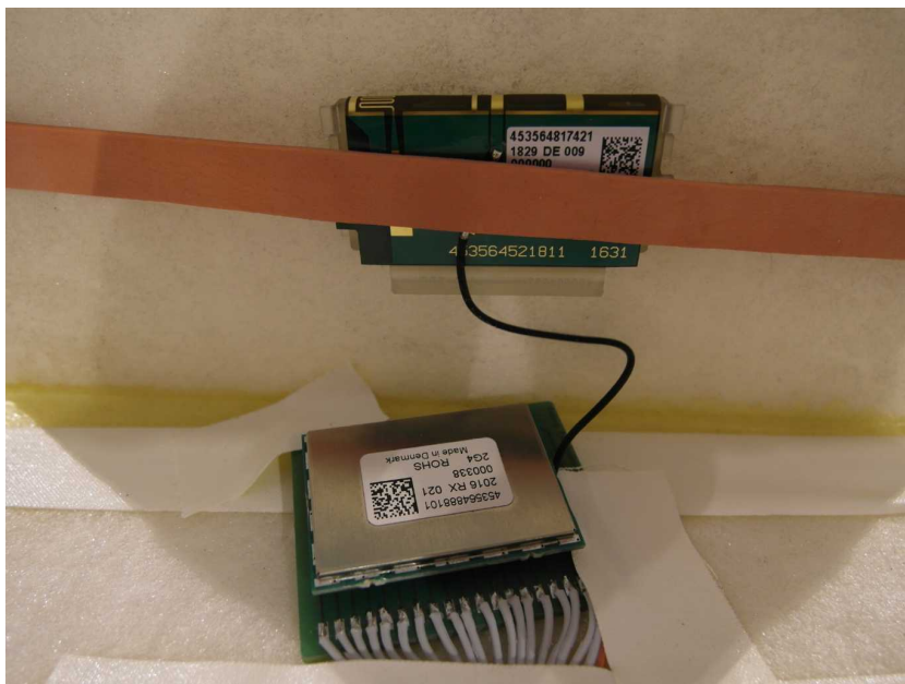
Photo 6: Setup Apollo
