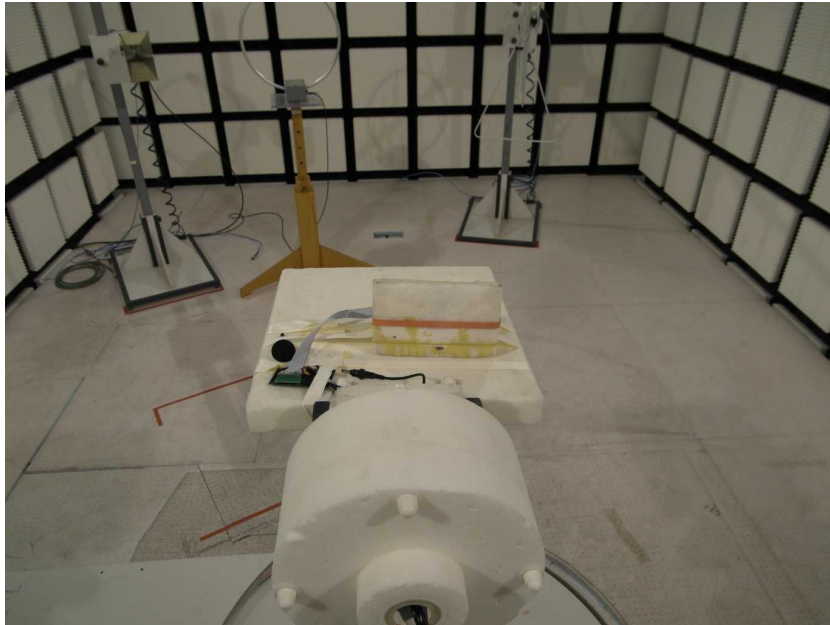
Photo 13: Setup Delphi
