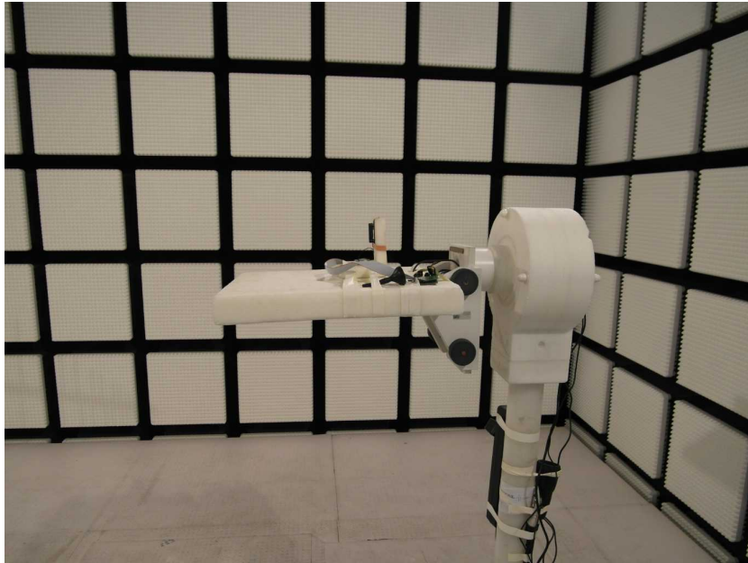
Photo 11: Setup Delphi
