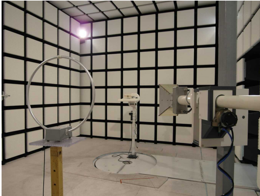
Photo 9: Setup Apollo
