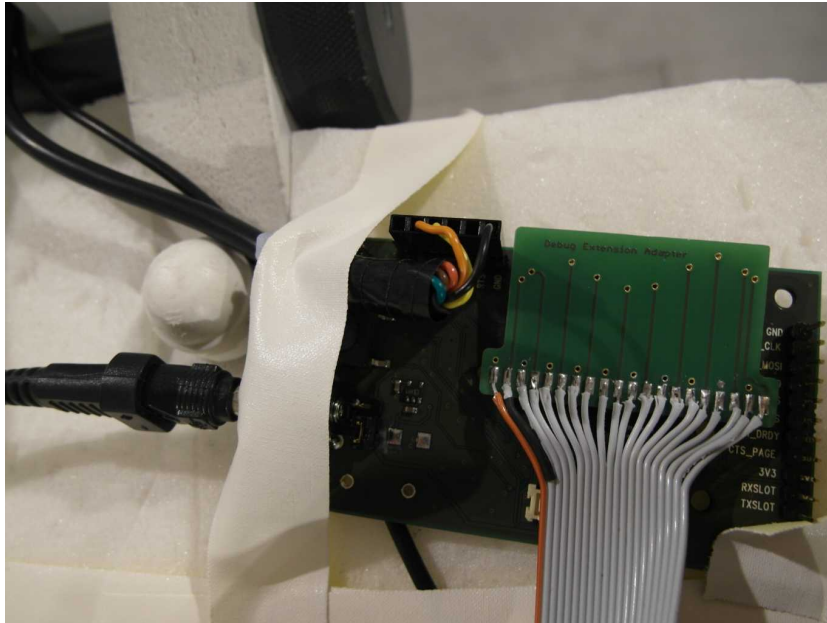
Photo 7: Setup Apollo
