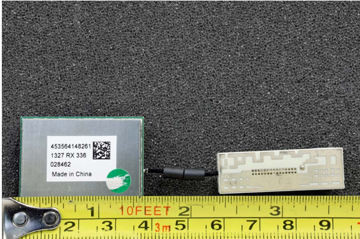
Transmitter module with antenna attached – Front
