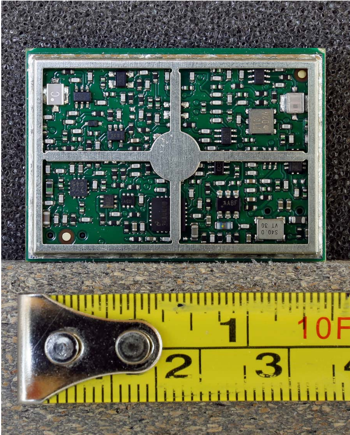
Transmitter module Front with cover removed
