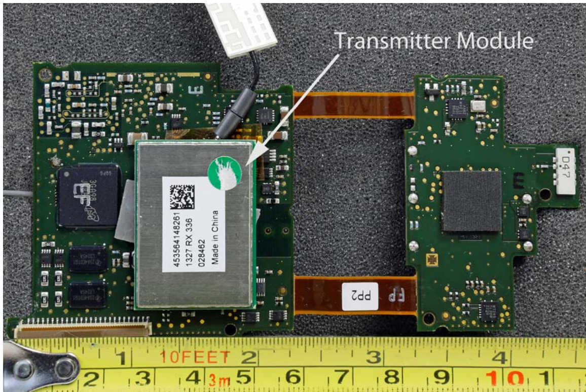
Main Board – Rear with antenna attached
