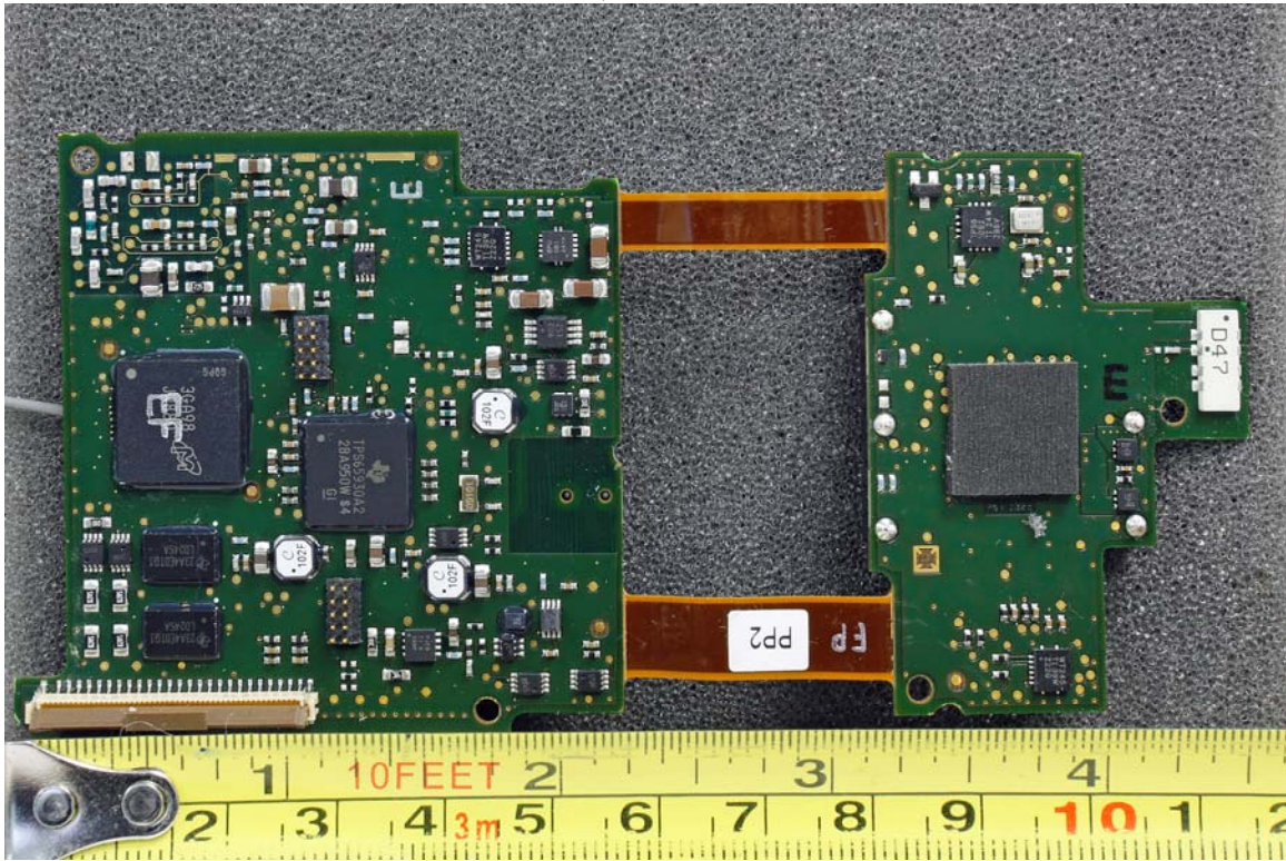
Main board – Rear with Antenna attached, transmitter removed
