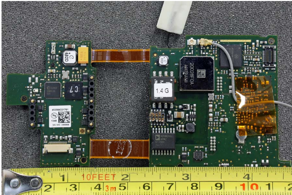
Main board – Front with antenna attached
