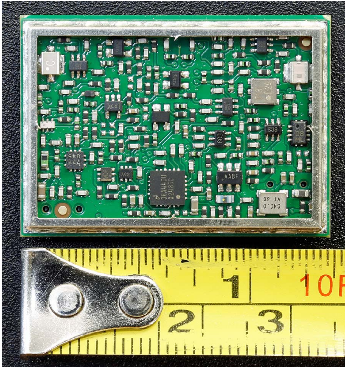
Transmitter module Front with cover removed and shield frame cross member removed
