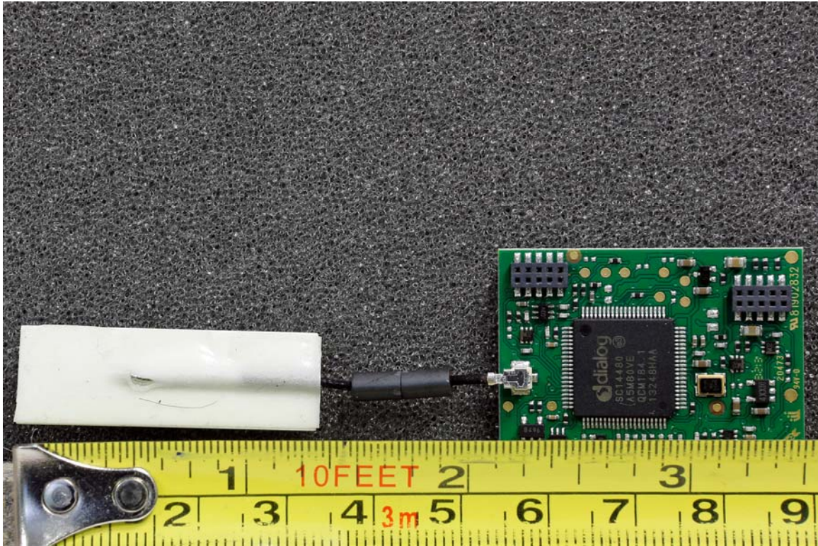
Transmitter module with antenna attached – Rear
