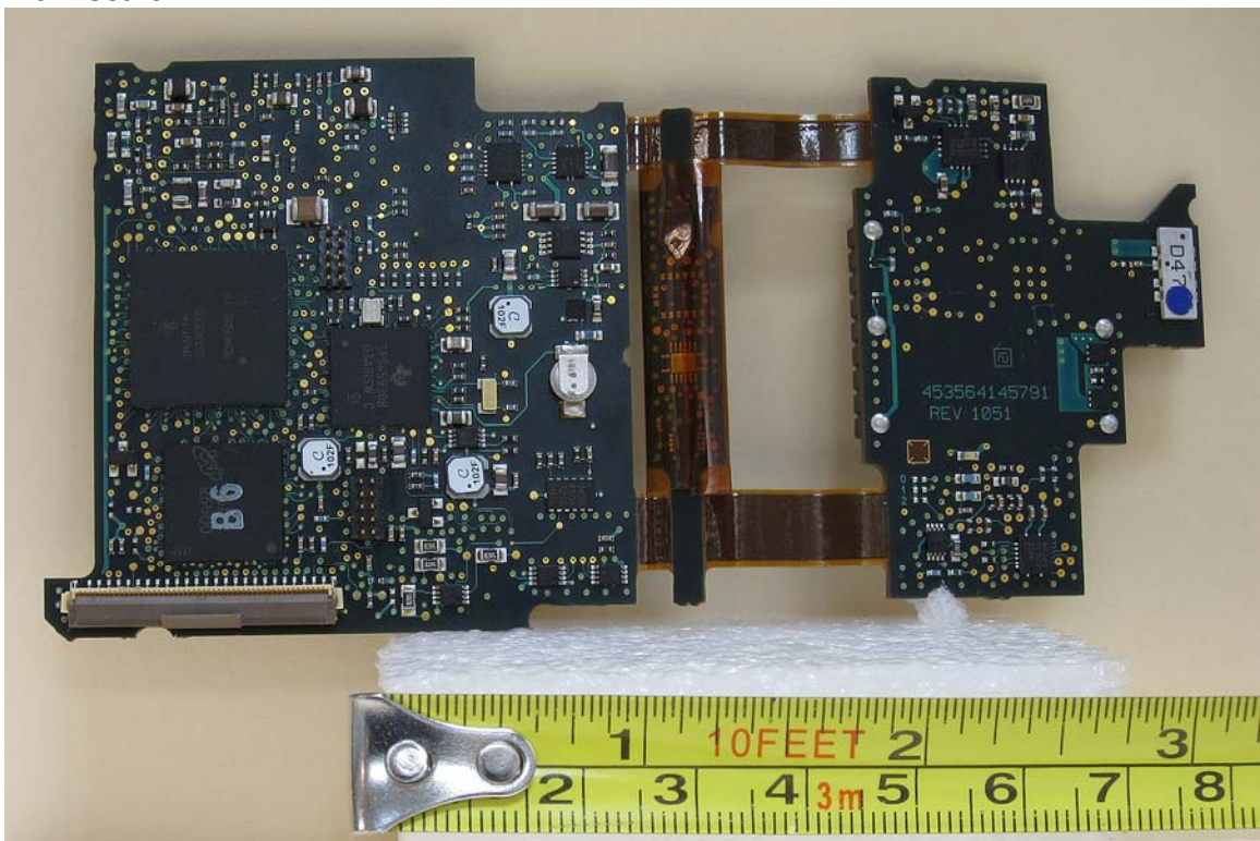
Main board
