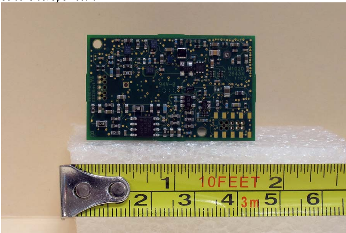
Solder Side: SpO2 board
