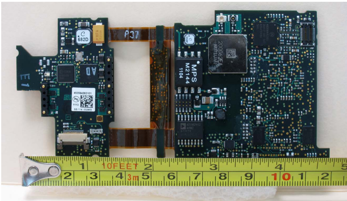
Main board
