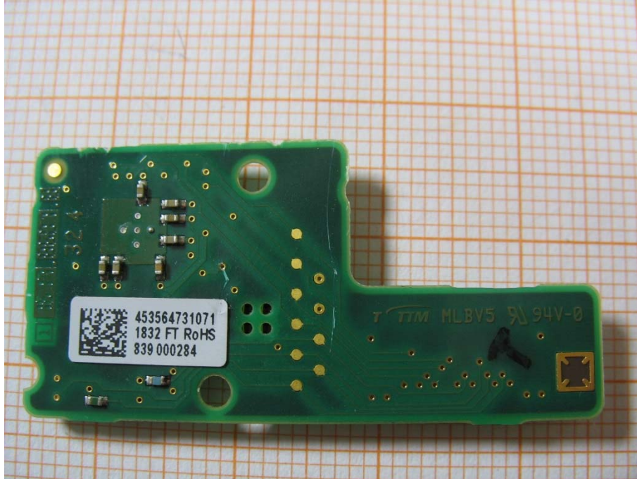
Photo 7: EUT
