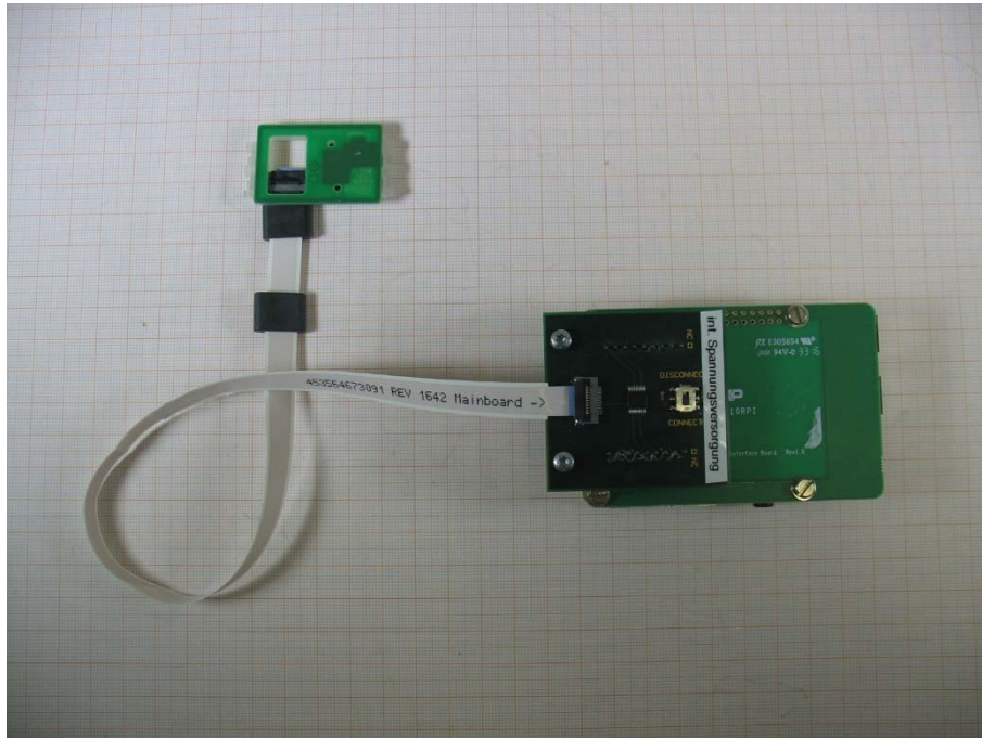
Photo 1: Test setup
