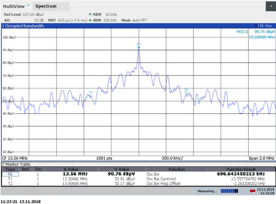
Plot 1: 99 % emission bandwidth, EUT without tag
