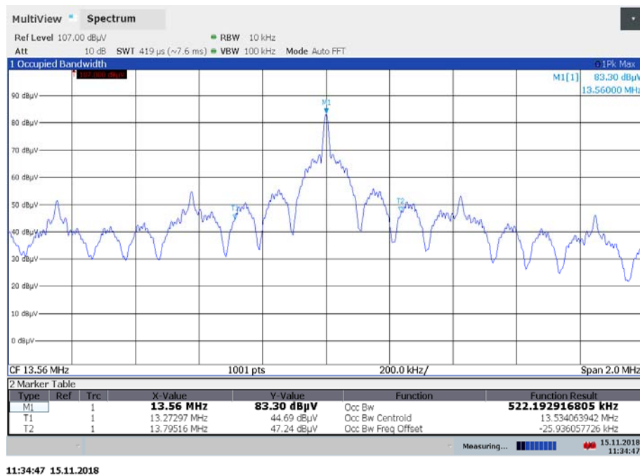
Plot 6: 99 % emission bandwidth, EUT with tag type 5
