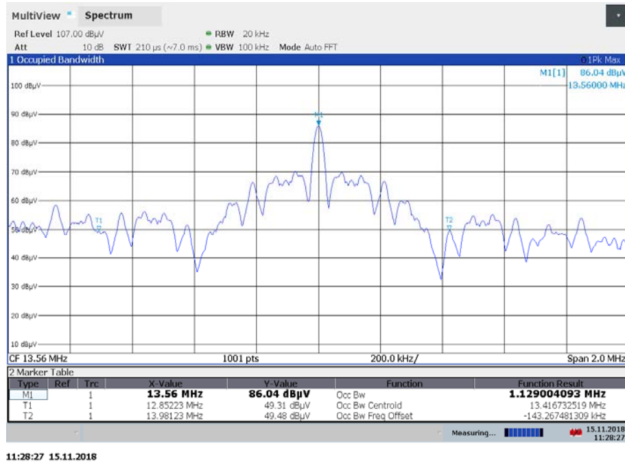
Plot 4: 99 % emission bandwidth, EUT with tag type 3
