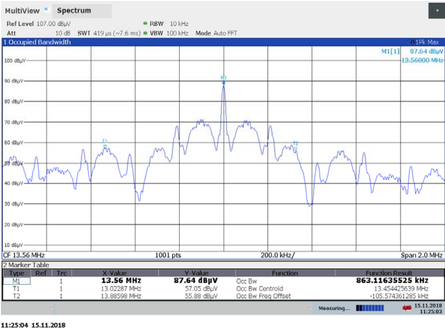
Plot 2: 99 % emission bandwidth, EUT with tag type 1
