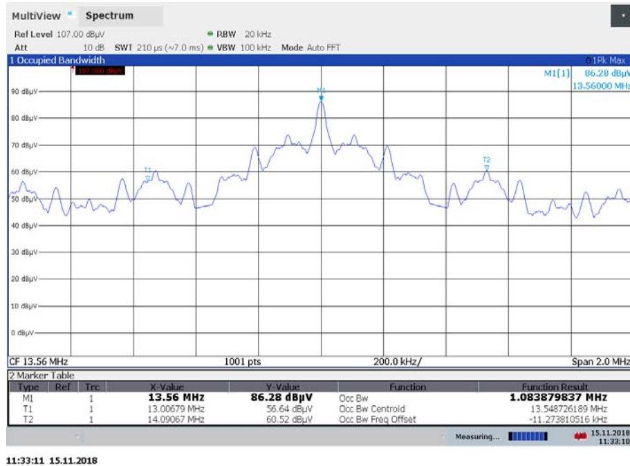
Plot 5: 99 % emission bandwidth, EUT with tag type 4
