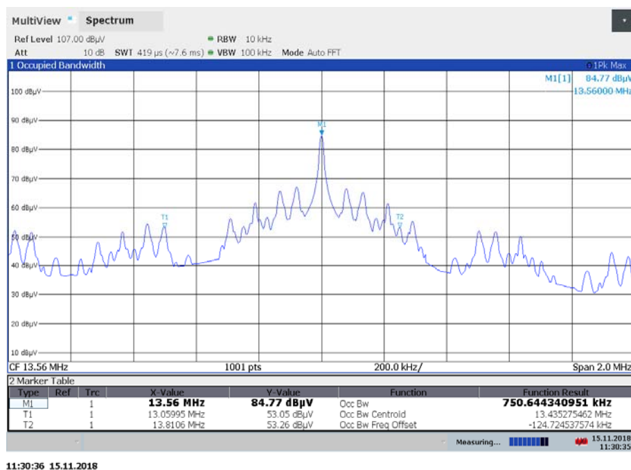
Plot 4: 99 % emission bandwidth, EUT with tag type 3
