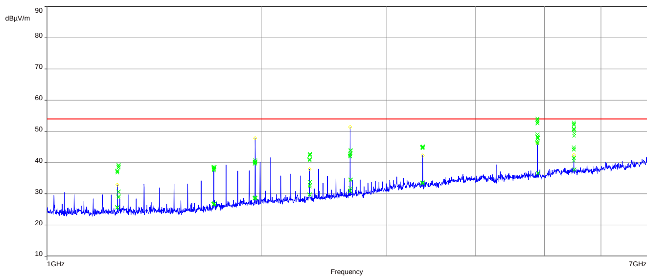
Plot 6: 1 GHz – 7 GHz, middle channel
