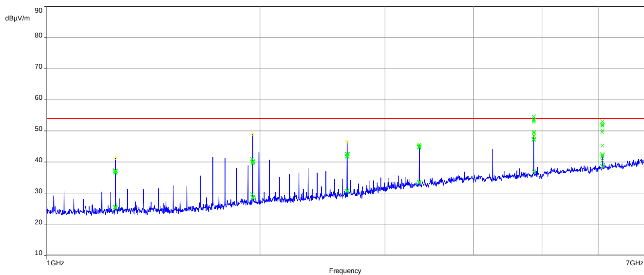
Plot 3: 1 GHz – 7 GHz, low channel
