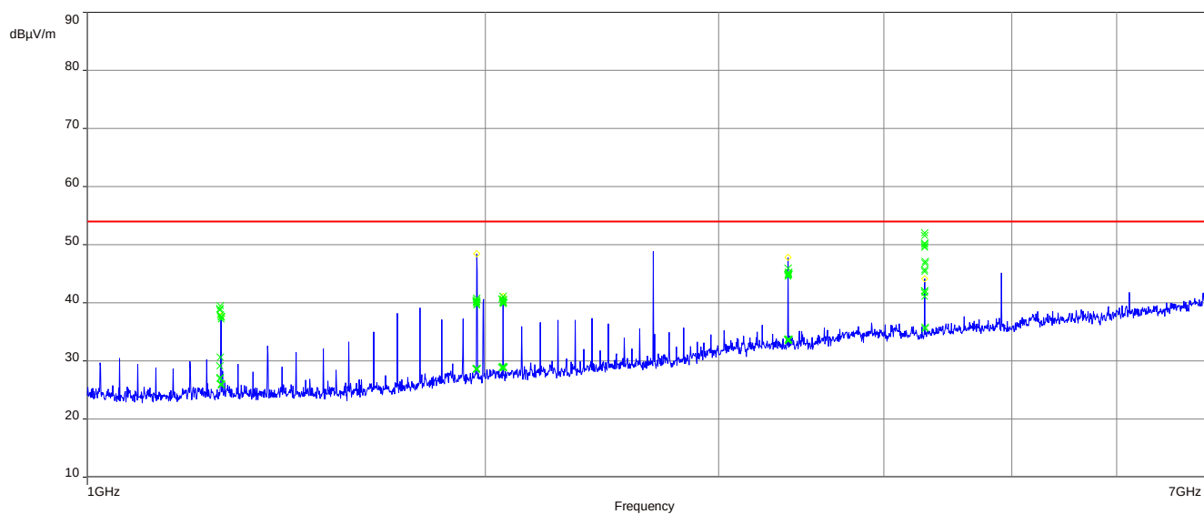
Plot 9: 1 GHz – 7 GHz, high channel
