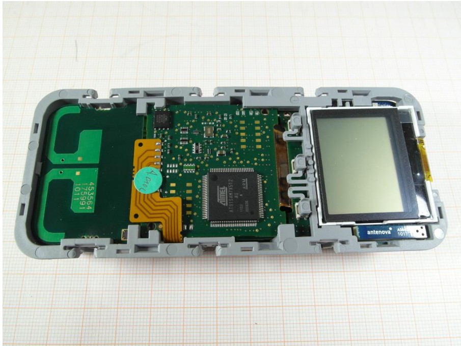
Photo 1: EUT opened (front side view)
