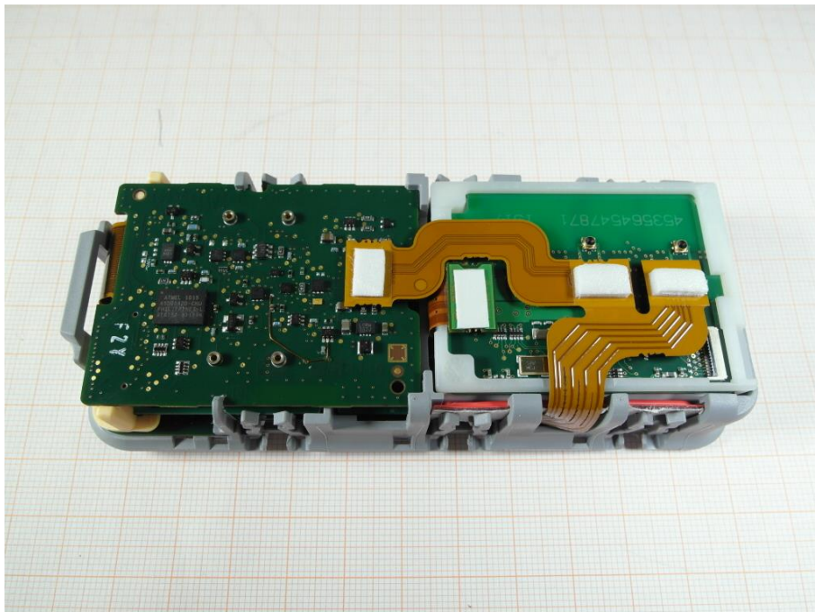
Photo 2: EUT opened (back side view)
