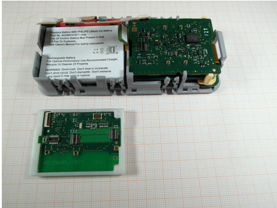
Photo 3: PCB 1 removed
