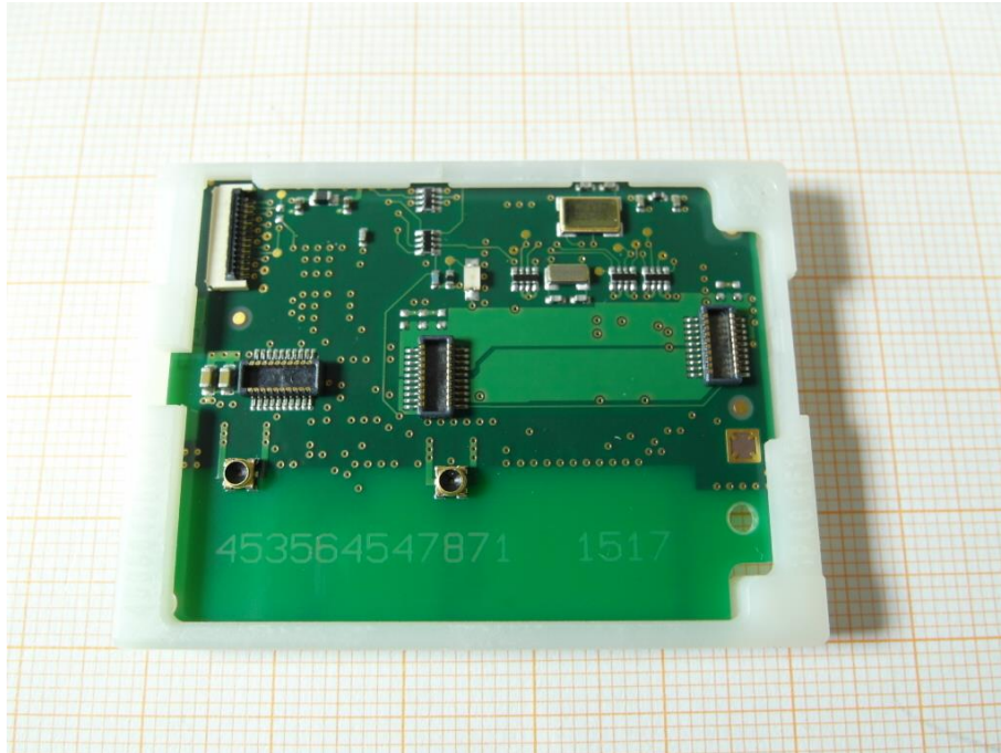
Photo 5: PCB 1 front side view
