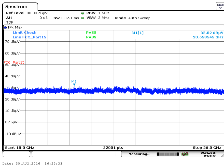
Plot 30: 18 GHz – 26 GHz, antenna horizontal/vertical, channel high, upper band
