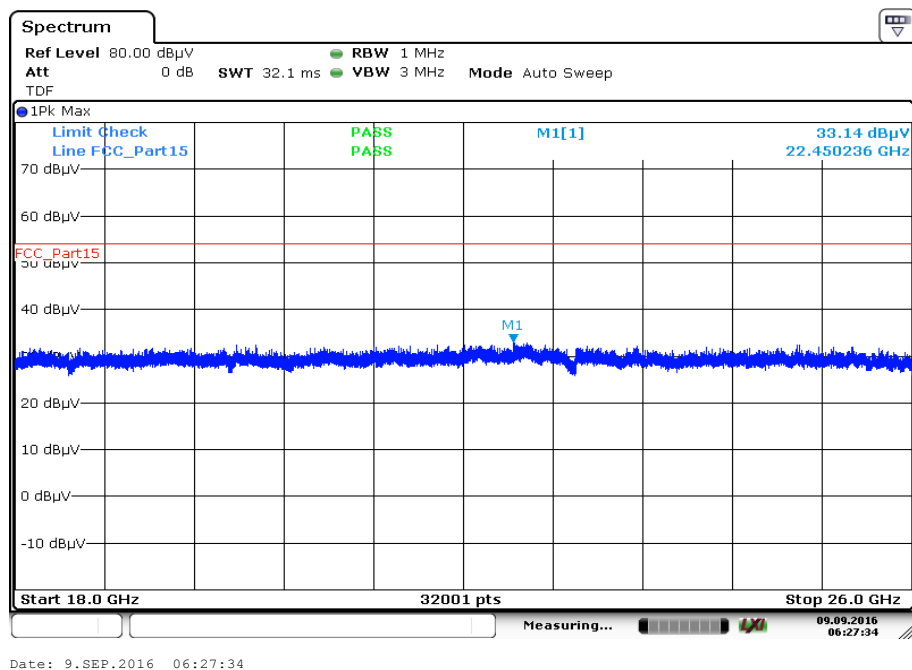
Plot 18: 18 GHz – 26 GHz, antenna horizontal/vertical, channel high, lower band
