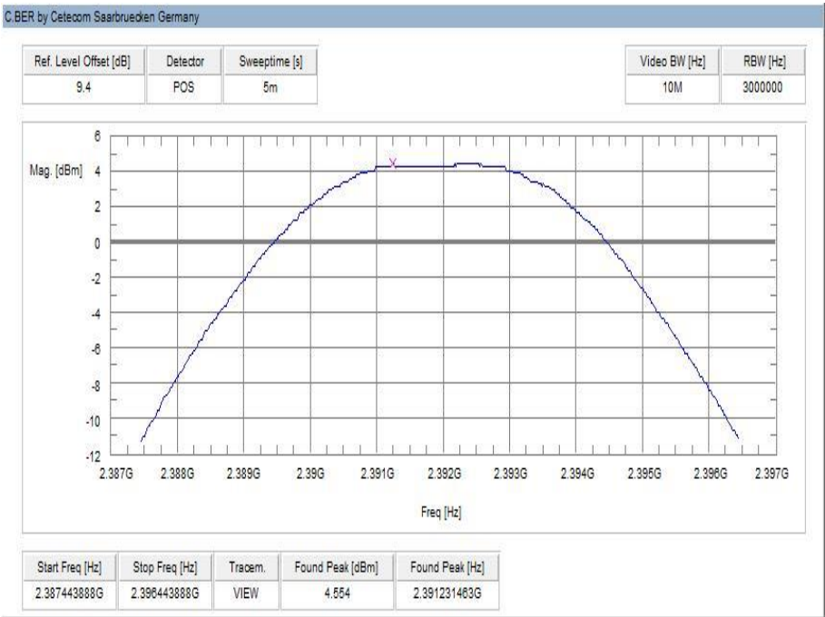
Plot 4: lower channel, upper band
