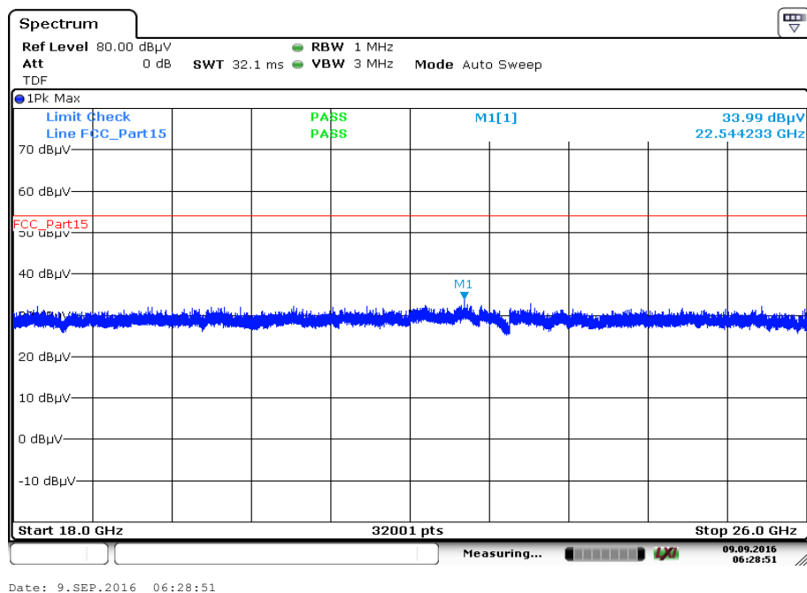
Plot 24: 18 GHz – 26 GHz, antenna horizontal/vertical, channel low, upper band
