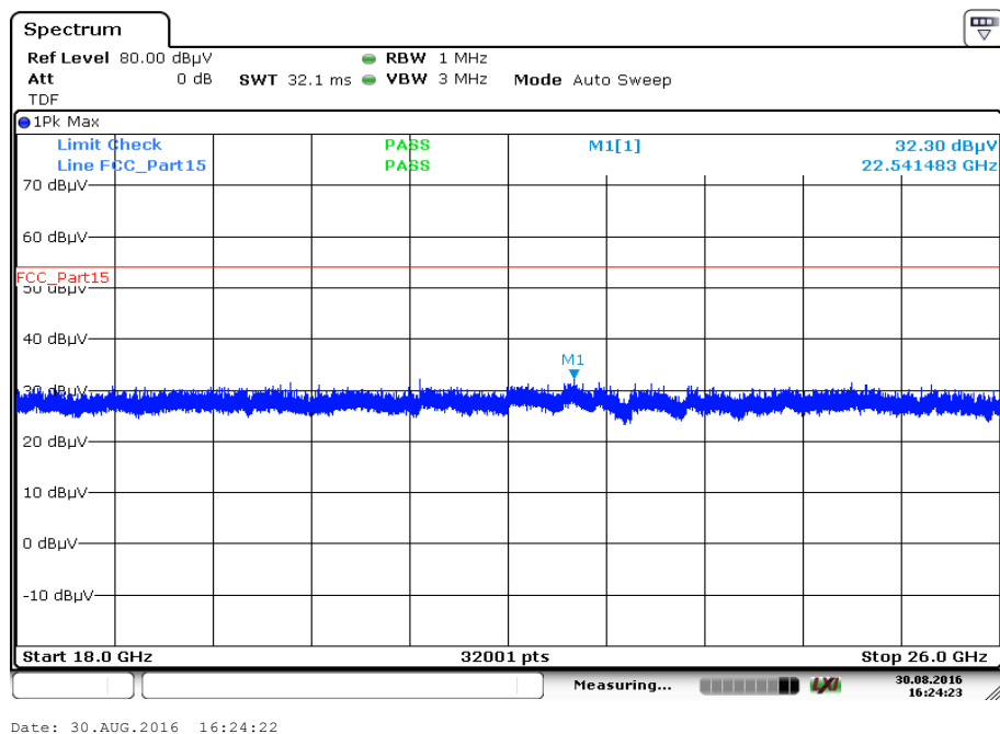
Plot 6: 18 GHz – 26 GHz, antenna horizontal/vertical, channel low, lower band
