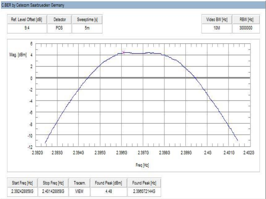
Plot 5: highest channel, upper band
