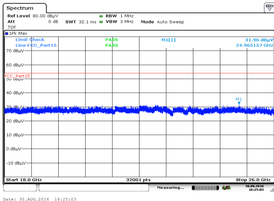
Plot 12: 18 GHz – 26 GHz, antenna horizontal/vertical, channel mid, lower band
