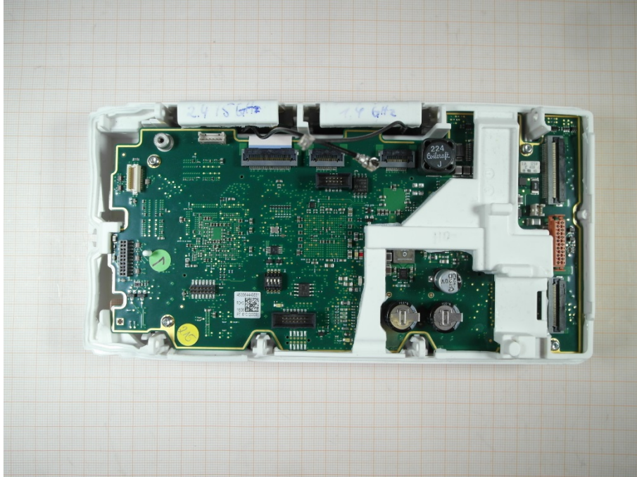
Photo 1: Antenna module - IV2 TRNS Antenna WLAN IIT 1.4
