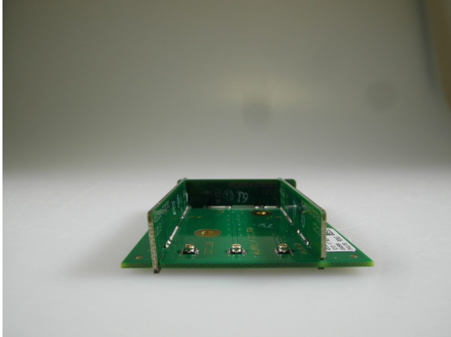
Photo 15: Antenna Ant 453564271931
