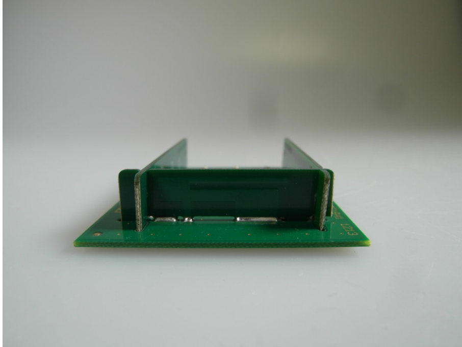
Photo 17: Antenna Ant 453564271931
