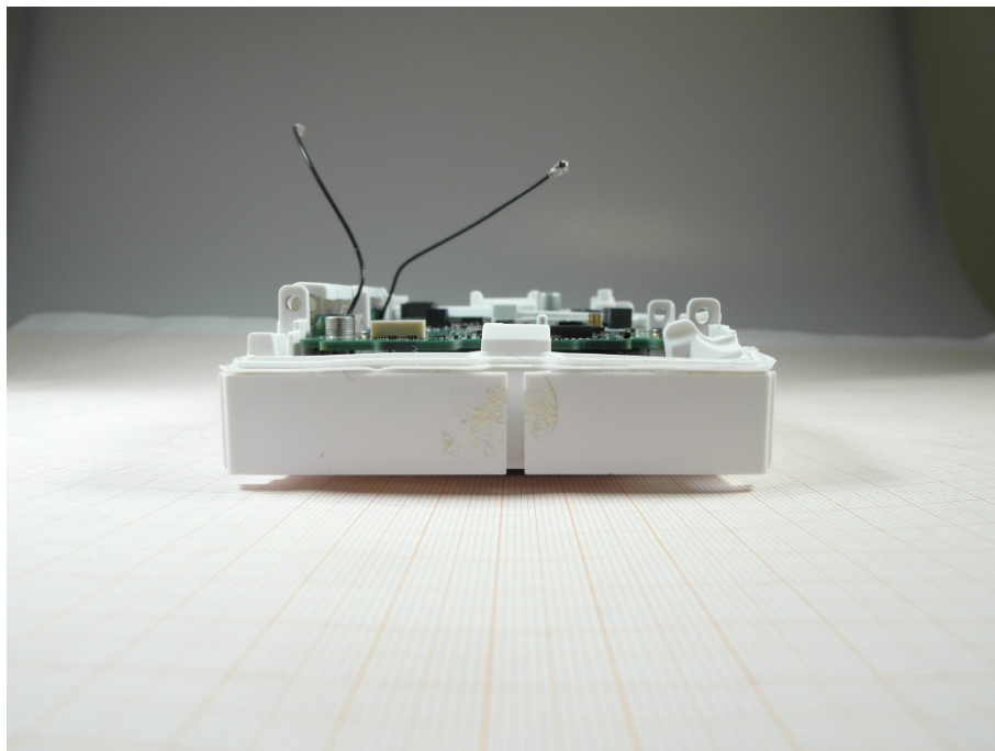
Photo 4: Antenna module - IV2 TRNS Antenna WLAN IIT 1.4
