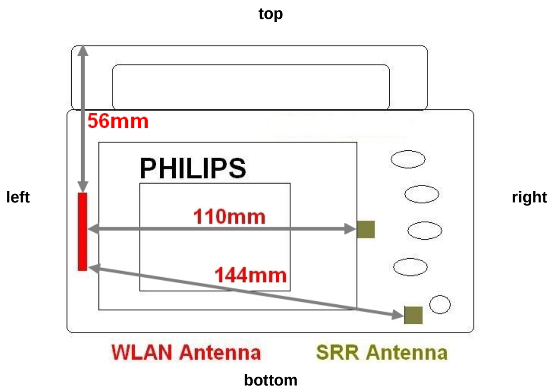
Antenna dimensions and separation distances
