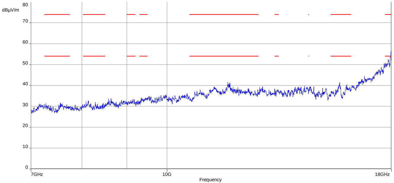
Plot 9: Highest channel, 7 GHz to 18 GHz, vertical & horizontal polarization
