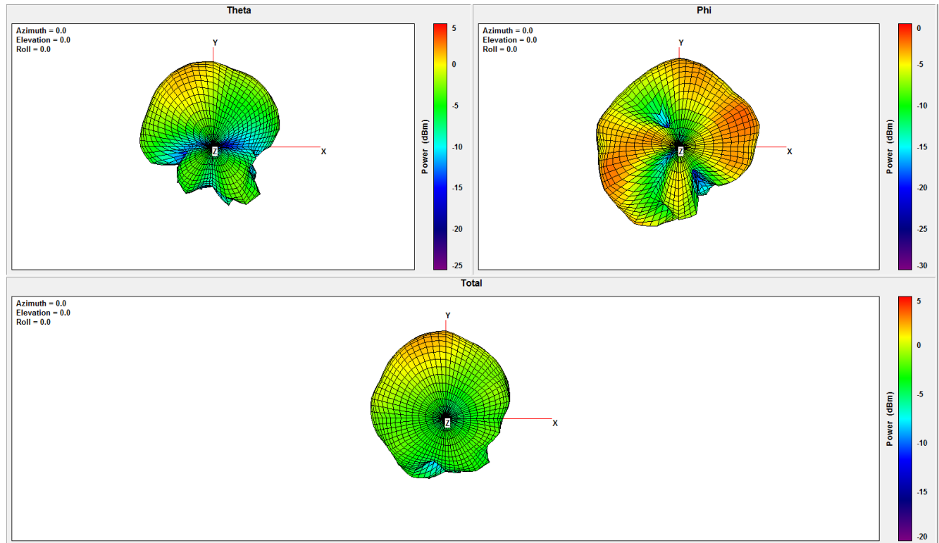
Plot 5: Highest channel, antenna diagram
