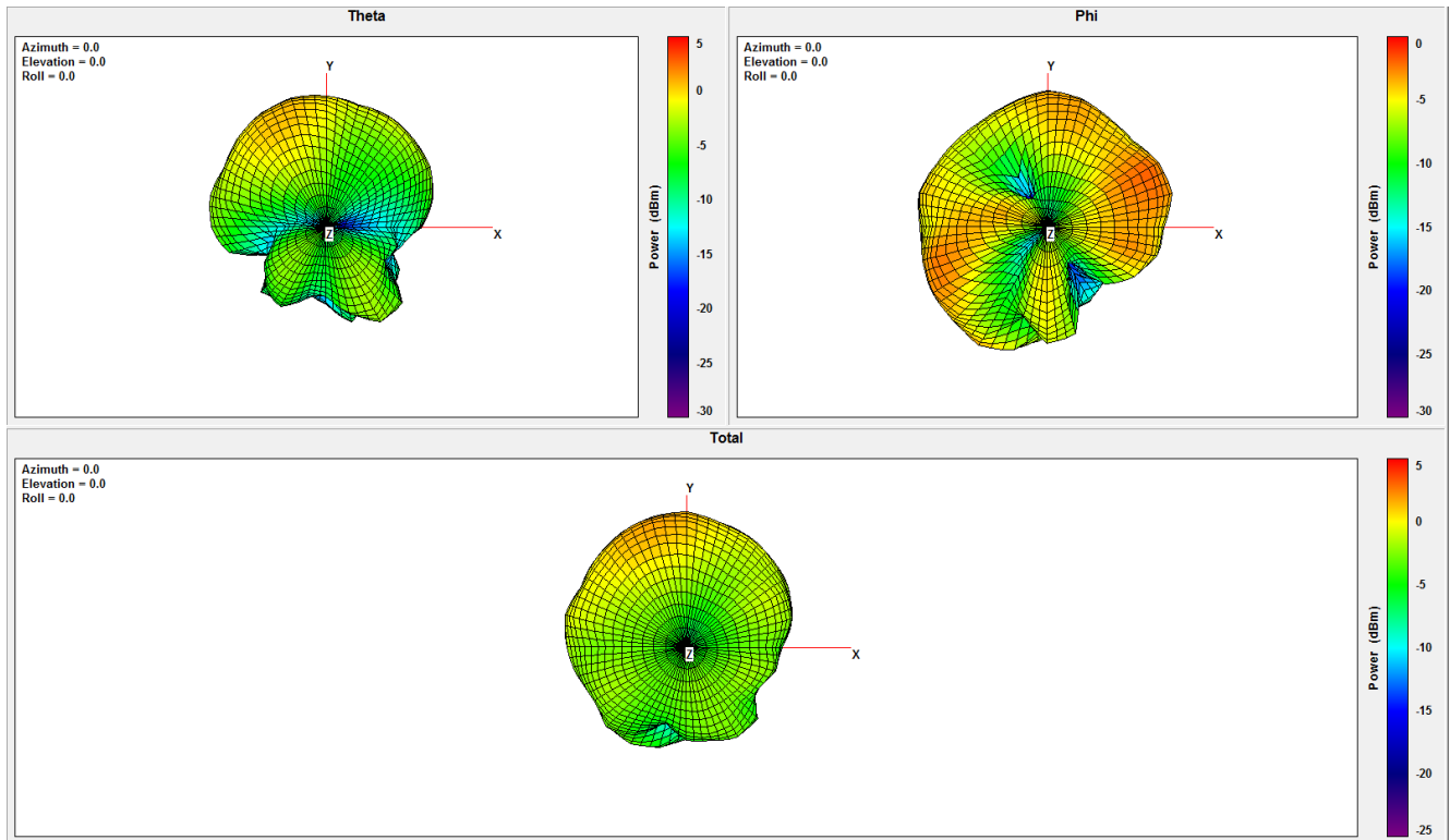
Plot 3: Mid channel, antenna diagram
