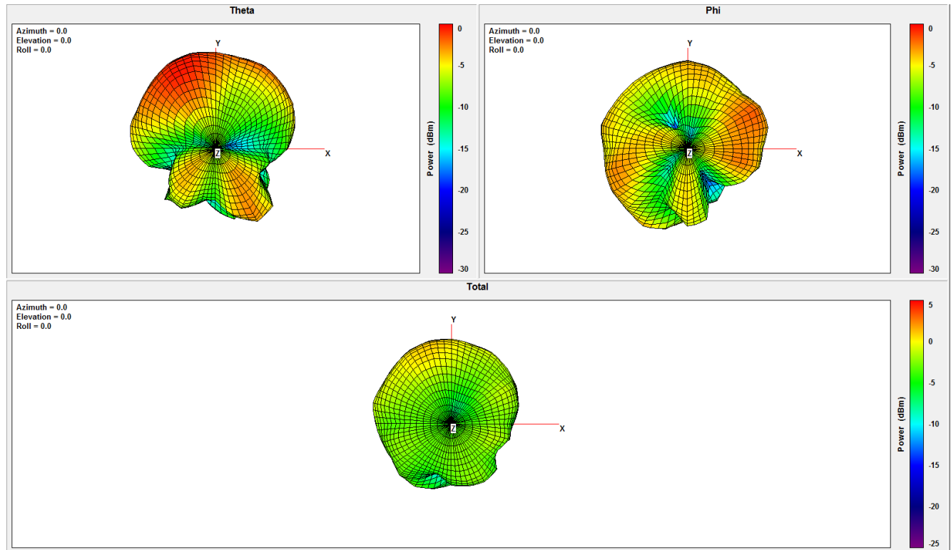
Plot 1: Lowest channel, antenna diagram
