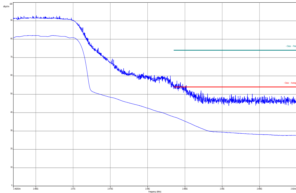
Plot 2: TX mode, upper band edge, vertical & horizontal polarization
