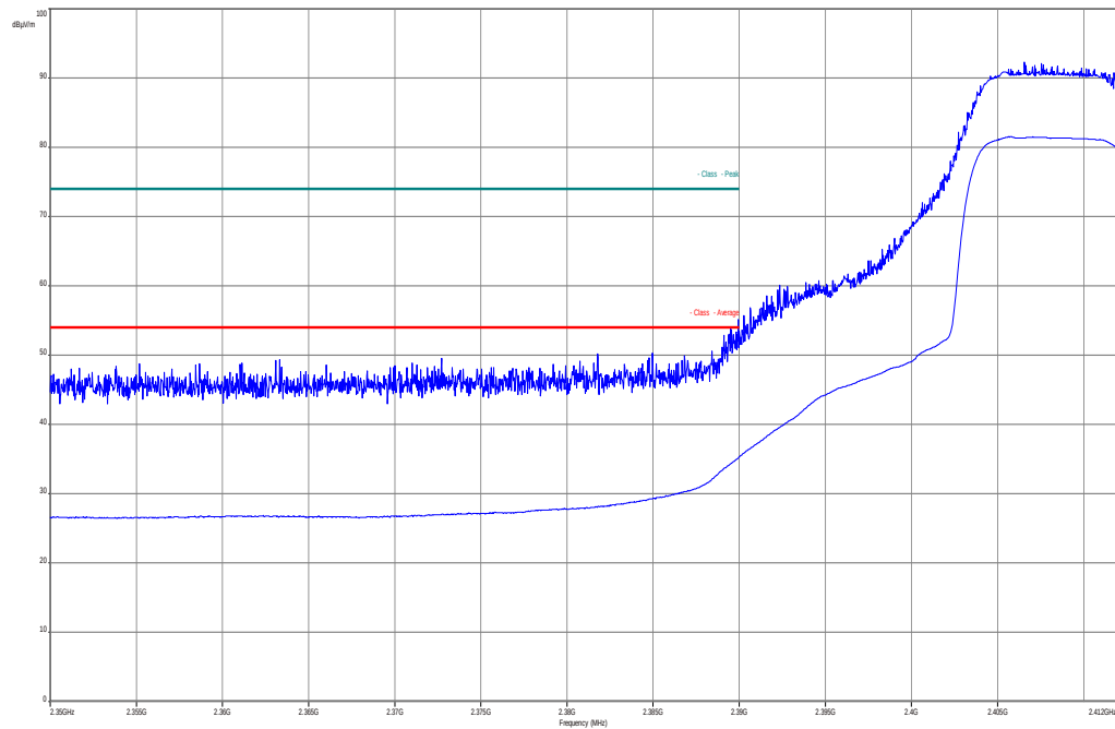
Plot 1: TX mode, lower band edge, vertical & horizontal polarization
