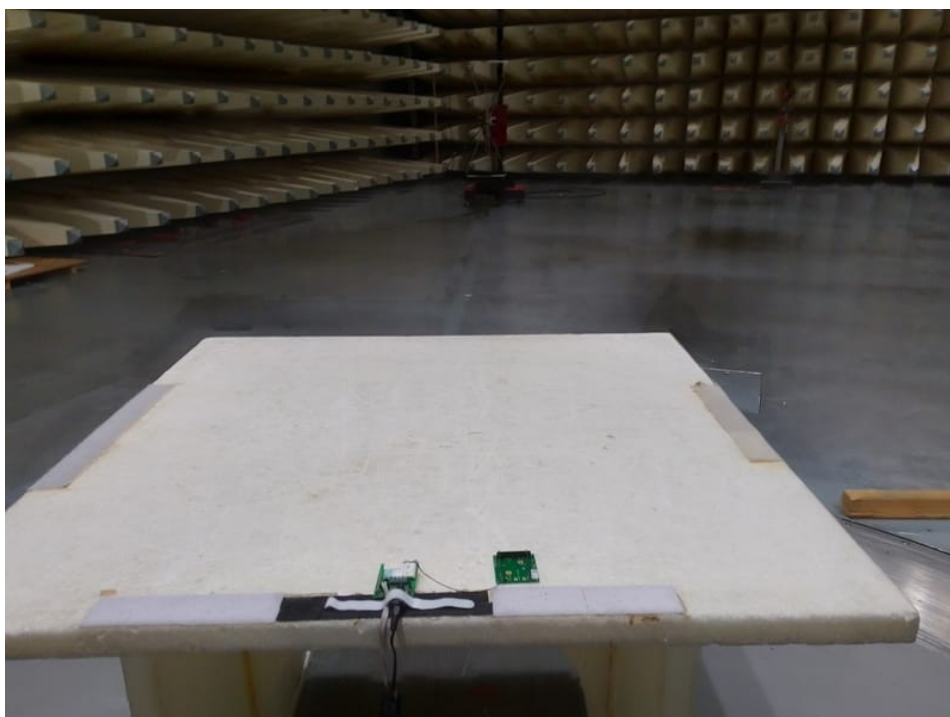
Photo 10: Tests with 453564271931 antenna
