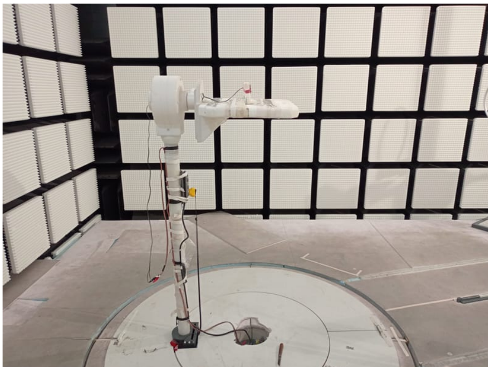
Photo 13: Tests with 453564682551 antenna
