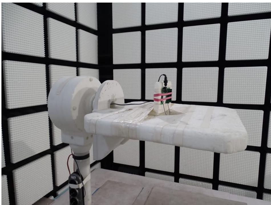
Photo 2: Tests with 453564271931 antenna
