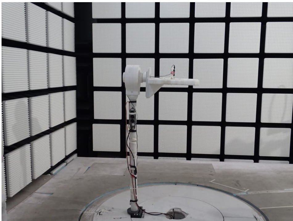
Photo 1: Tests with 453564271931 antenna
