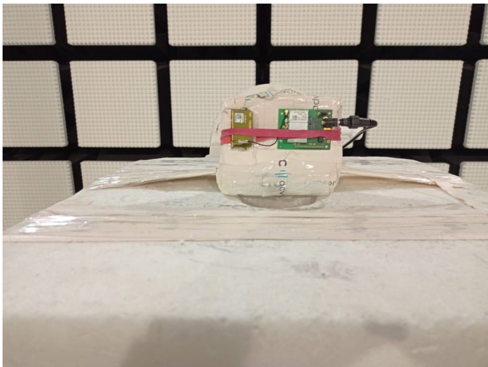
Photo 17: Tests with 453564682551 antenna
