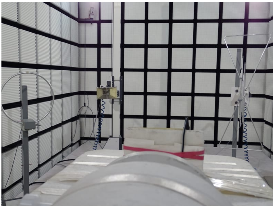
Photo 5: Tests with 453564271931 antenna
