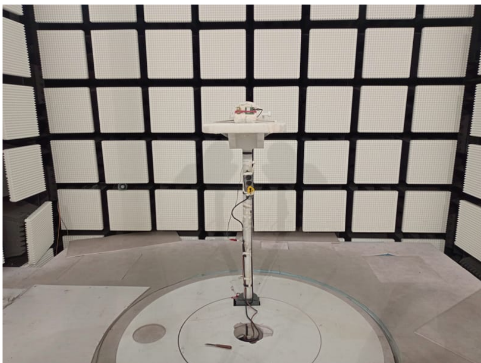
Photo 16: Tests with 453564682551 antenna
