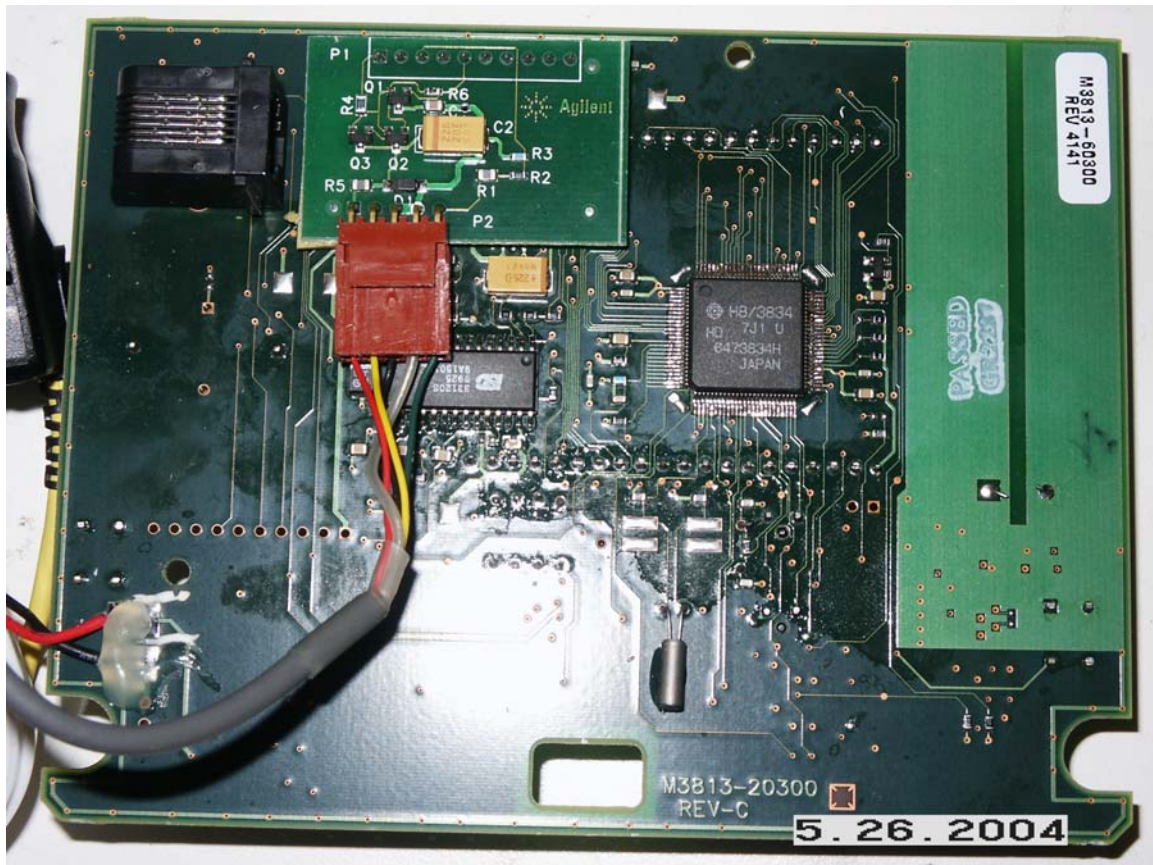
Rear of PCB removed from EUT housing
