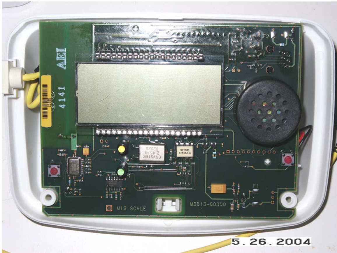
Board and display with cover removed
