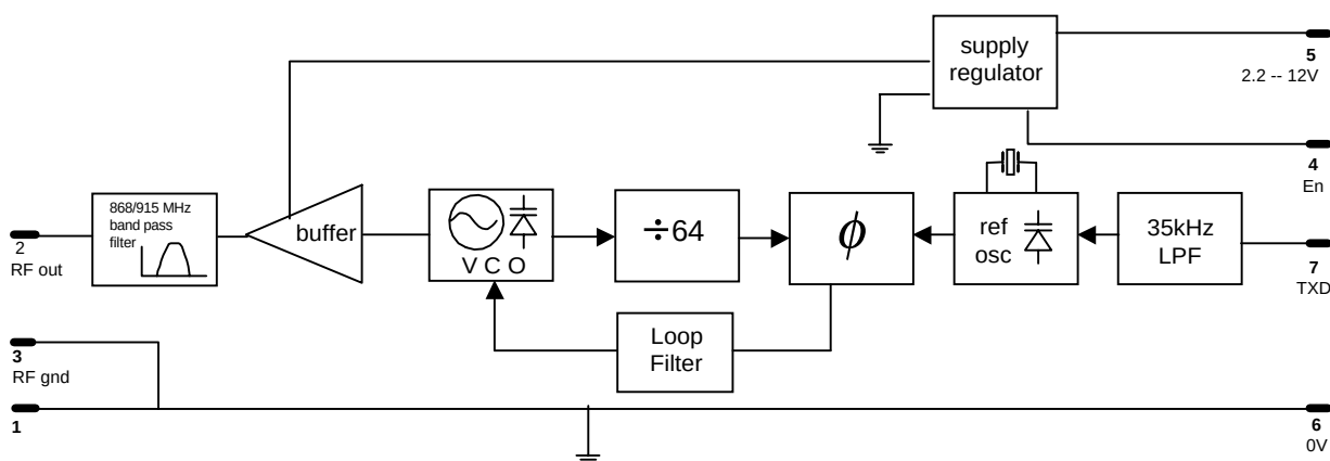
Fig 1 :TX3A block diagram
