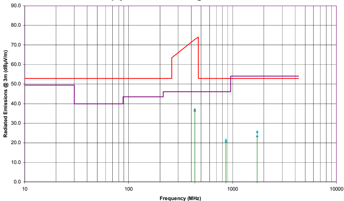
Radiated Emissions Measurements @ 3m OFTS FCC Section 15.231(e) Lyngsoe Exciter, Model EX21 @ 433.92 MHz
