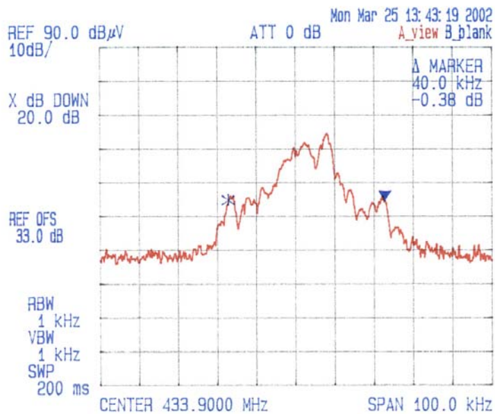
20 dB Emission Bandwidth
