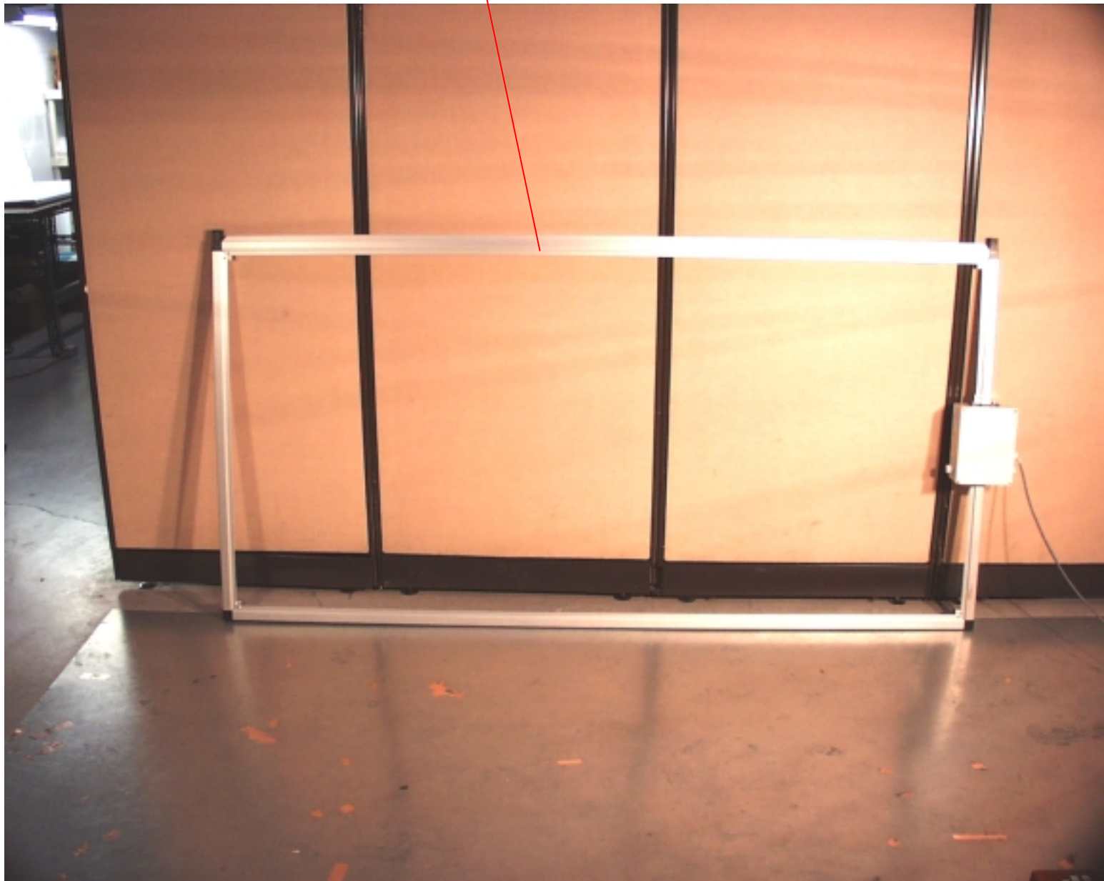
125 kHz Loop Antenna
