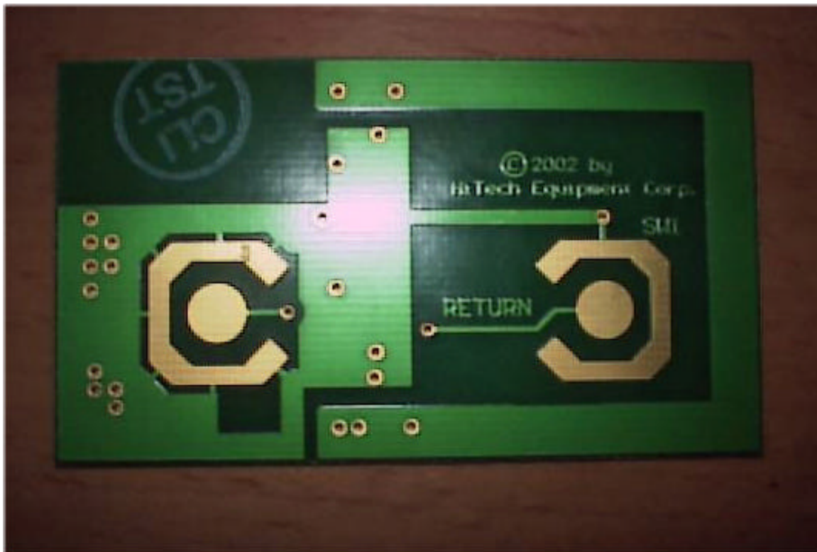
BOARD TOP
