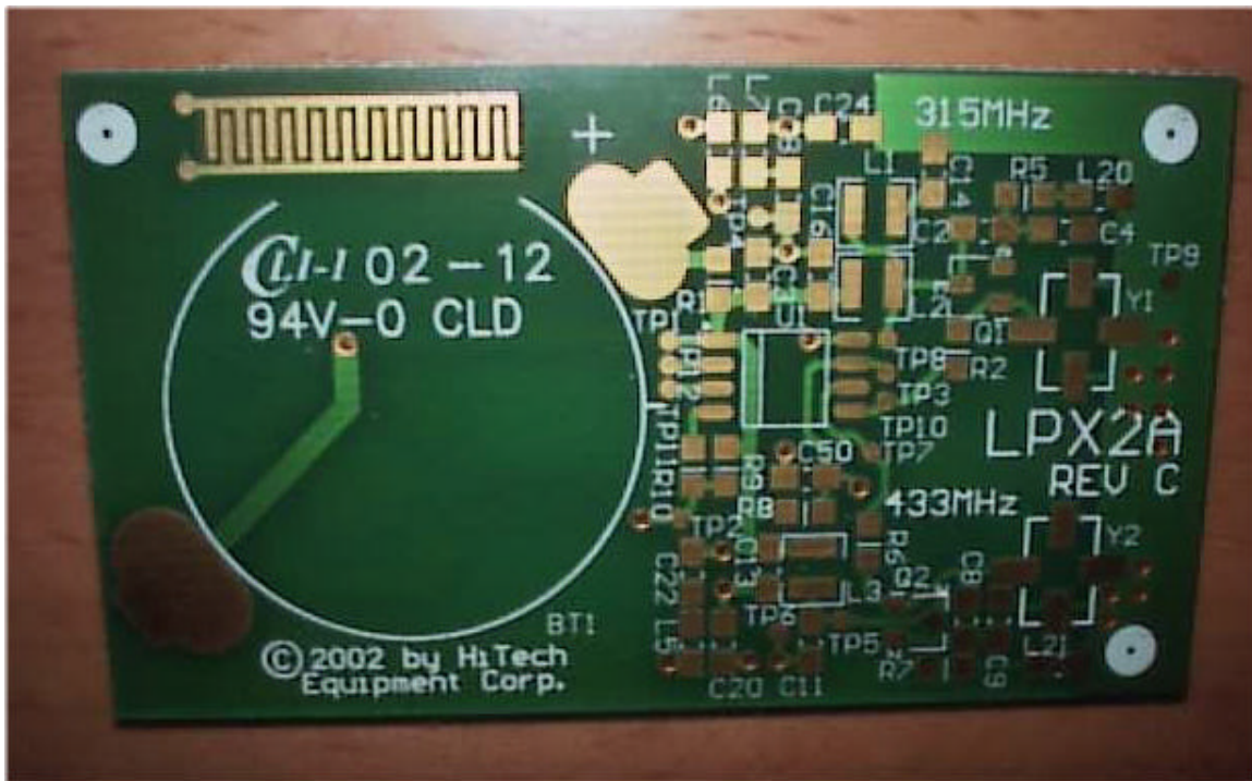
BOARD BOTTOM
