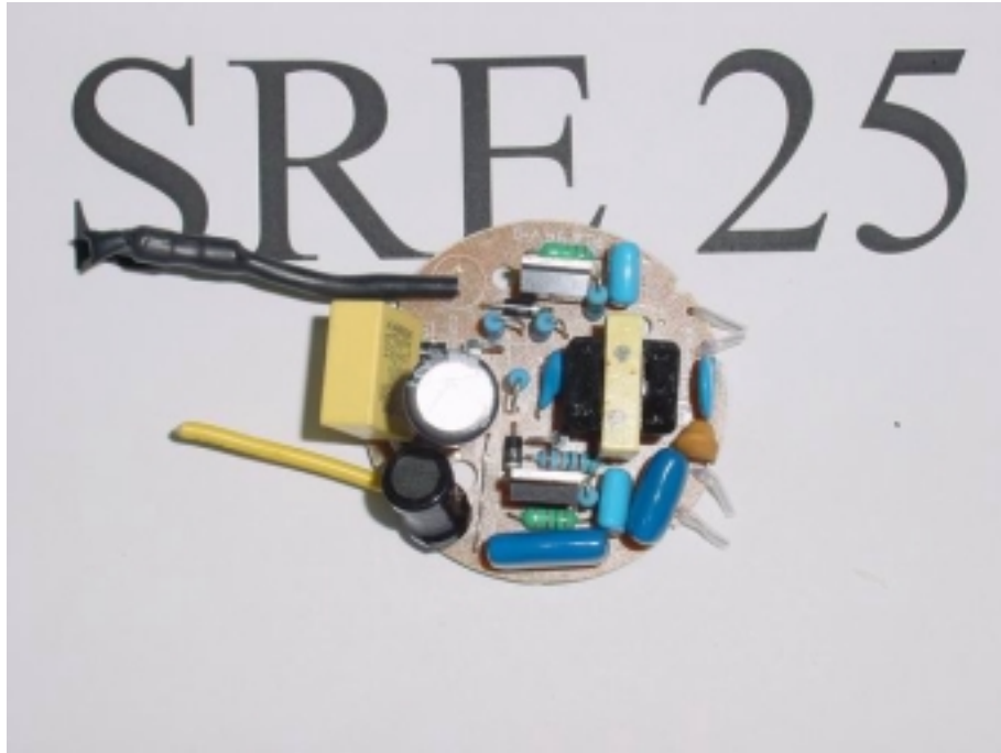
Figure 30 Main Board, Component Side
