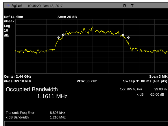
Plot 6. 20 dB Bandwidth, 20 dB BW, 3DH1, mid
