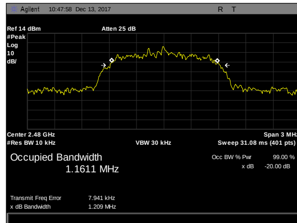
Plot 4. 20 dB Bandwidth, 20 dB BW, 3DH1, high
