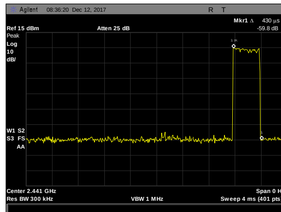
Plot 14. Dwell Time, Dwell Time 3DH1
