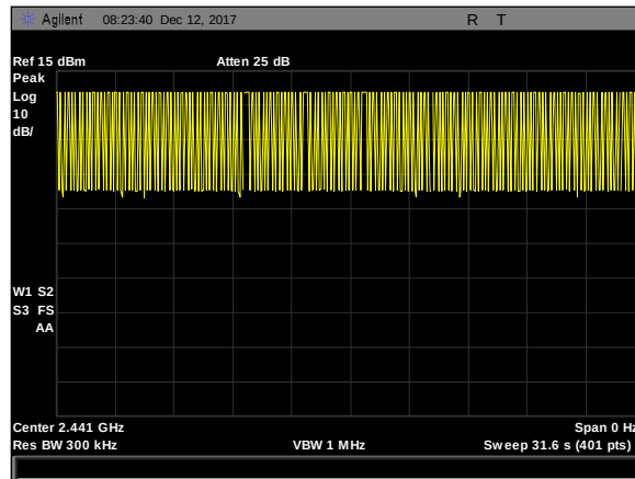
Plot 12. Dwell Time, burst DM1
