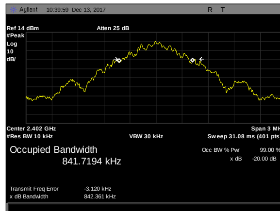
Plot 8. 20 dB Bandwidth, 20 dB BW, DM1, low
