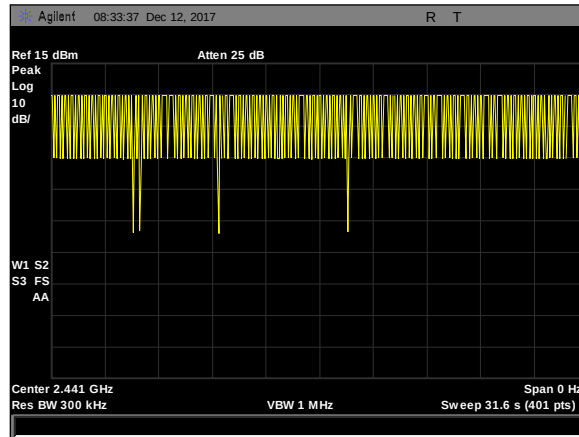
Plot 10. Dwell Time, burst 2DH1
