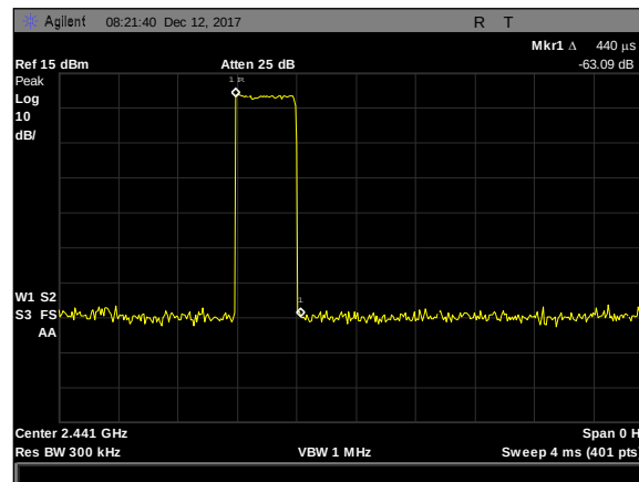
Plot 15. Dwell Time, Dwell Time DM1
