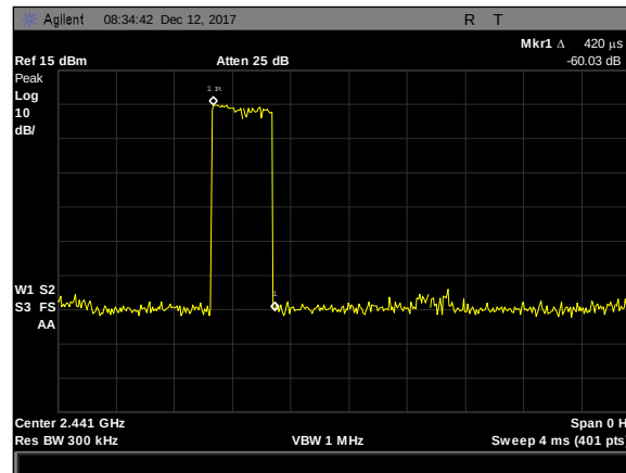
Plot 13. Dwell Time, Dwell Time 2DH1
