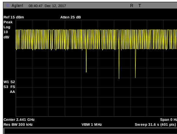
Plot 11. Dwell Time, burst 3DH1
