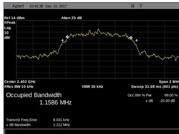
Plot 5. 20 dB Bandwidth, 20 dB BW, 3DH1, low
