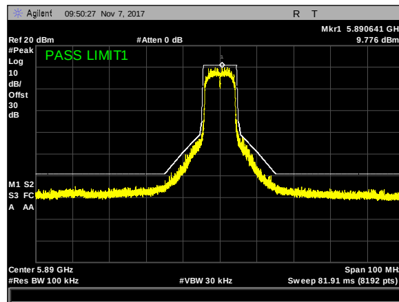
Plot 9. Transmit Spectrum Mask, Class C, 5890, ANT1
