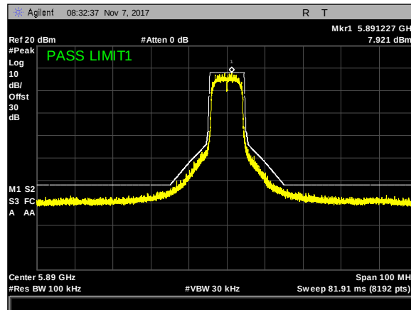
Plot 10. Transmit Spectrum Mask, Class C, 5890, ANT2
