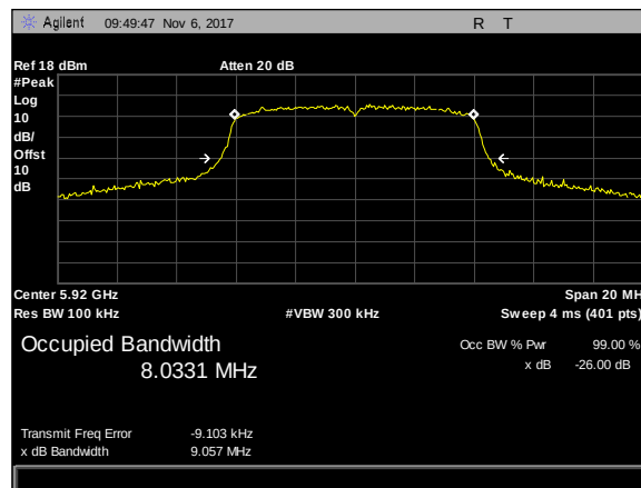
Plot 13. Emissions Bandwidth, 26dB BW, high channel, 5920M, ANT2
