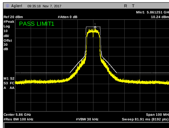
Plot 7. Transmit Spectrum Mask, Class C, 5860, ANT1
