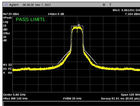
Plot 8. Transmit Spectrum Mask, Class C, 5860, ANT2
