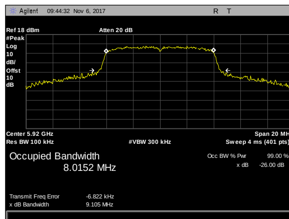
Plot 14. Emissions Bandwidth, 26dB BW, high channel, 5920M, ANT1
