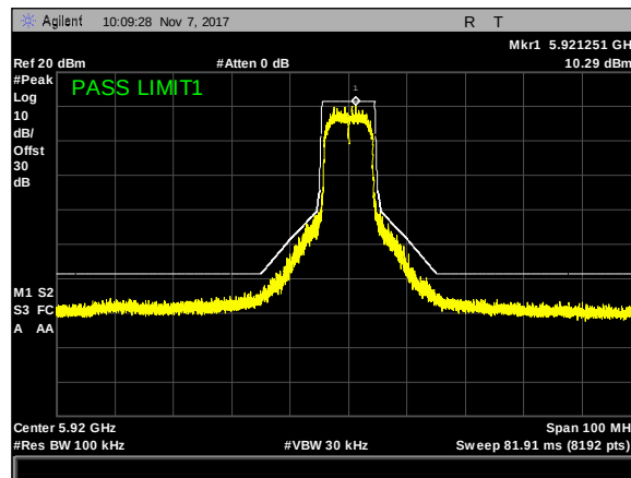
Plot 11. Transmit Spectrum Mask, Class C, 5920, ANT1
