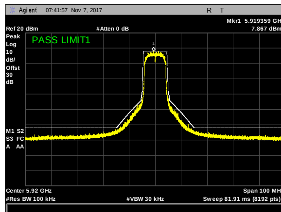
Plot 12. Transmit Spectrum Mask, Class C, 5920, ANT2
