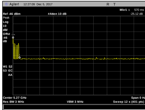
Plot 19. Channel Move Time
