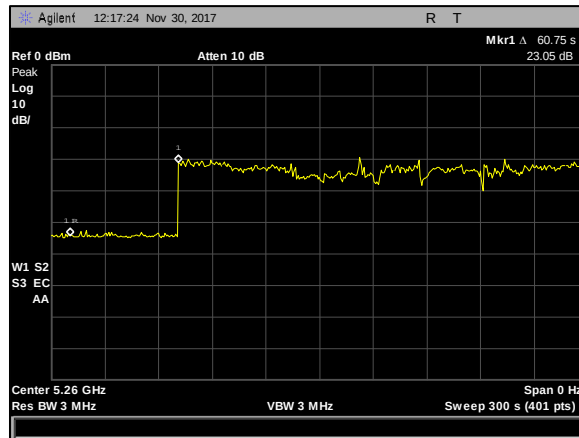
Plot 15. CAC Time
