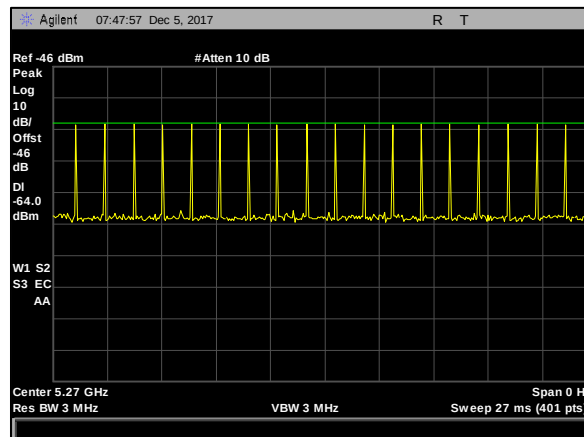
Plot 8. Radar Waveform Calibration, 5270 MHz, Type 0, 40 MHz
