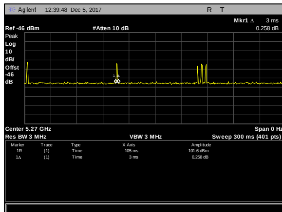
Plot 18. Channel Close Time
