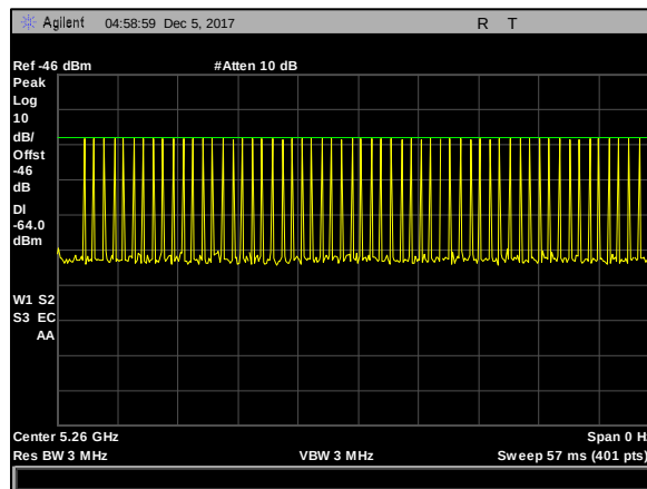
Plot 2. Radar Waveform Calibration, 5260 MHz, Type 1, 20 MHz
