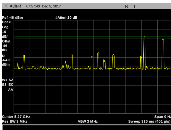
Plot 14. Radar Waveform Calibration, 5270 MHz, Type 6, 40 MHz
