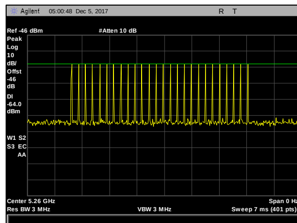
Plot 3. Radar Waveform Calibration, 5260 MHz, Type 2, 20 MHz
