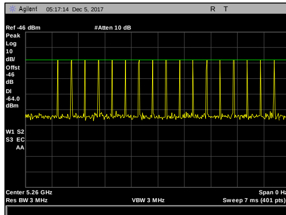
Plot 4. Radar Waveform Calibration, 5260 MHz, Type 3, 20 MHz
