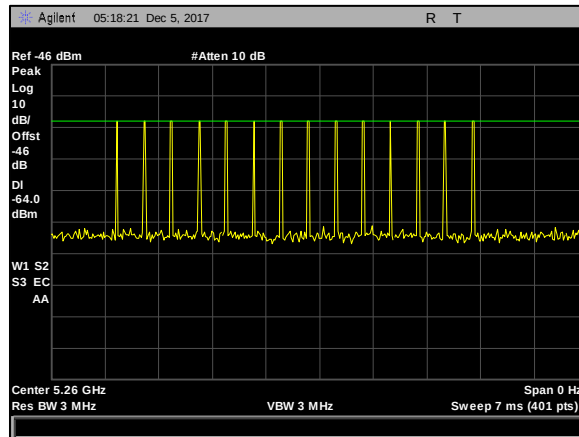
Plot 5. Radar Waveform Calibration, 5260 MHz, Type 4, 20 MHz
