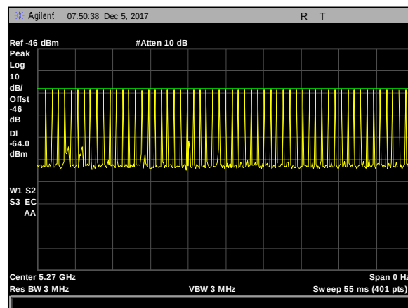
Plot 9. Radar Waveform Calibration, 5270 MHz, Type 1, 40 MHz
