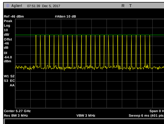
Plot 10. Radar Waveform Calibration, 5270 MHz, Type 2, 40 MHz
