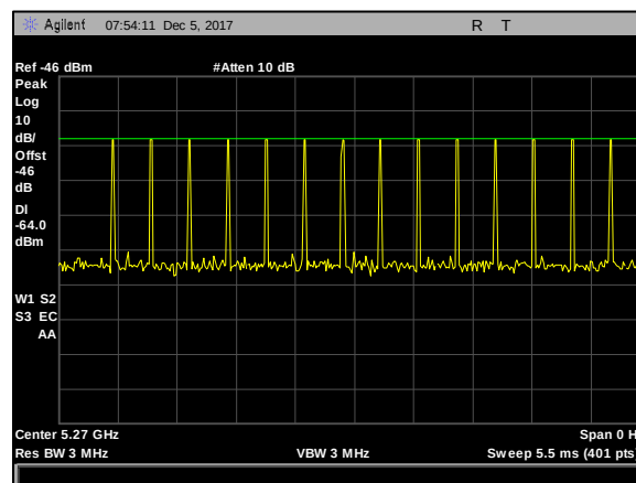
Plot 12. Radar Waveform Calibration, 5270 MHz, Type 4, 40 MHz
