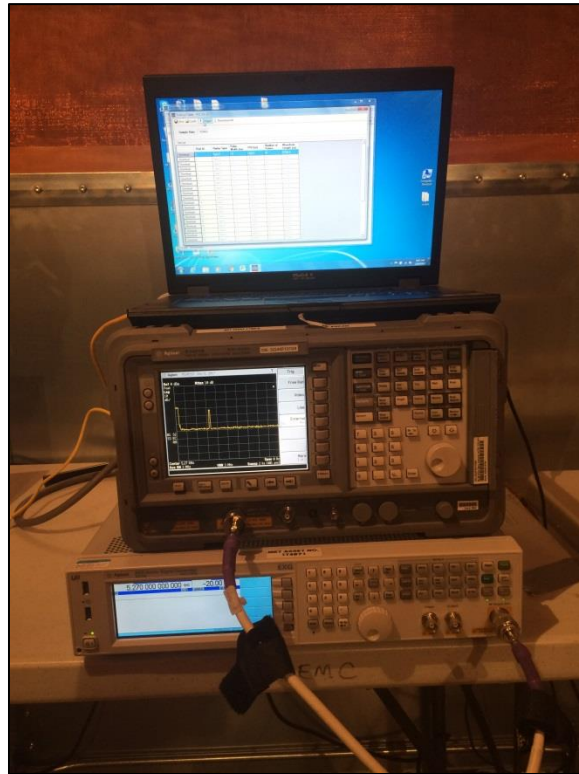
Photograph 2. DFS Test Calibration Setup
