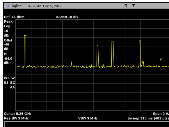
Plot 7. Radar Waveform Calibration, 5260 MHz, Type 6, 20 MHz
