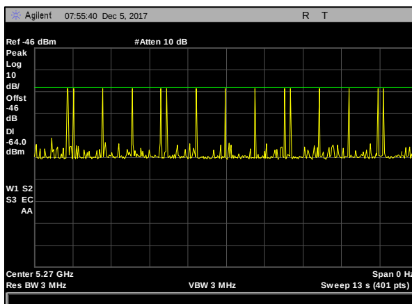
Plot 13. Radar Waveform Calibration, 5270 MHz, Type 5, 40 MHz
