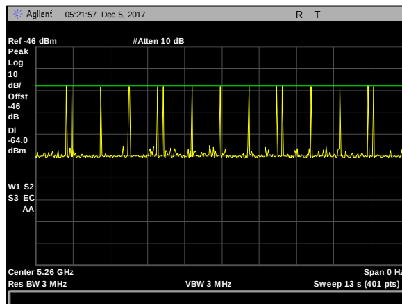
Plot 6. Radar Waveform Calibration, 5260 MHz, Type 5, 20 MHz
