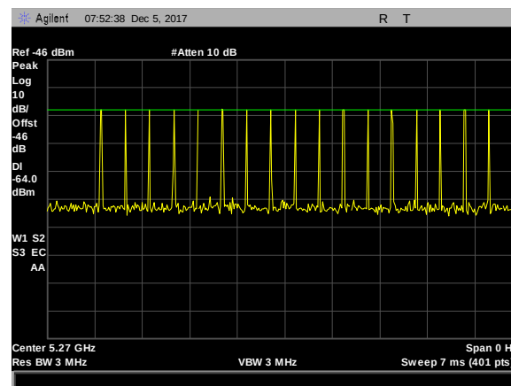
Plot 11. Radar Waveform Calibration, 5270 MHz, Type 3, 40 MHz
