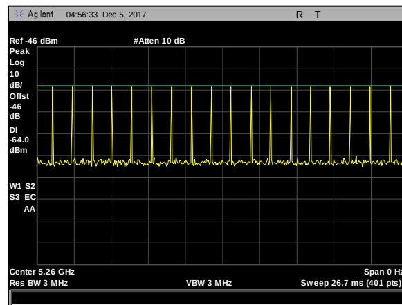
Plot 1. Radar Waveform Calibration, 5260 MHz, Type 0, 20 MHz
