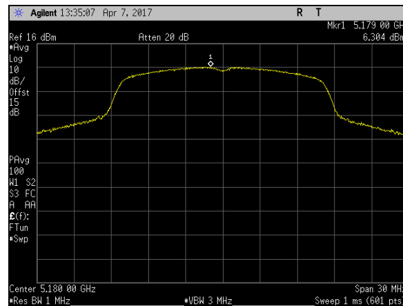
Plot 34. Power Spectral Density, BW 20 M, Ch. 5180 MHz, A mode, Port 1
