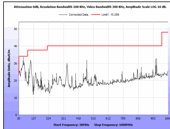
Plot 91. Undesirable Emissions, 30 MHz - 1 GHz 5200 MHz A Mode 20 MHz Port 1
