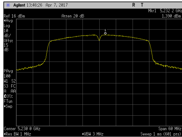
Plot 48. Power Spectral Density, BW 40 M, Ch. 5230 MHz, N mode, Port 1
