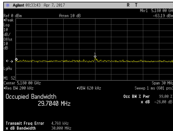
Plot 1. 26 dB Occupied Bandwidth, 26 dB, BW 20 M, Ch. 5180 MHz, A mode, Port 1, Noise Floor
