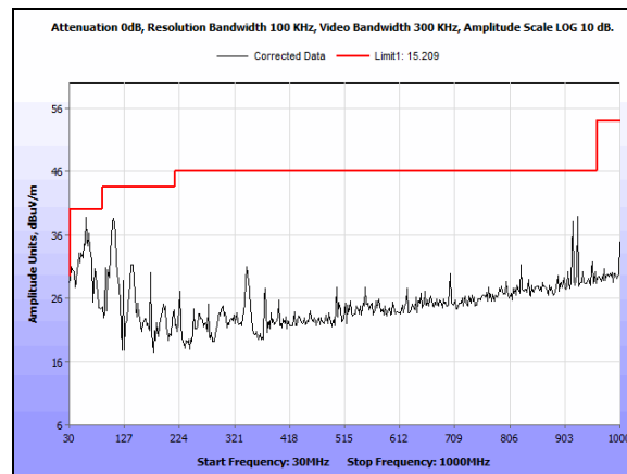
Plot 92. Undesirable Emissions, 30 MHz - 1 GHz 5200 MHz A Mode 20 MHz Port 2
