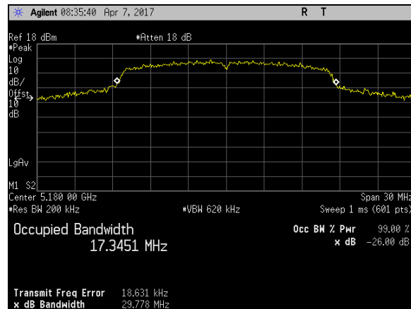
Plot 2. 26 dB Occupied Bandwidth, 26 dB, BW 20 M, Ch. 5180 MHz, A mode, Port 1
