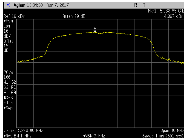
Plot 45. Power Spectral Density, BW 20 M, Ch. 5240 MHz, N mode, Port 2
