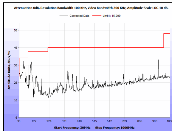
Plot 93. Undesirable Emissions, 30 MHz - 1 GHz 5200 MHz N Mode 20 MHz Port 1
