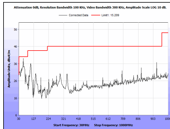
Plot 86. Undesirable Emissions, 30 MHz - 1 GHz 5180 MHz A Mode 20 MHz Port 2
