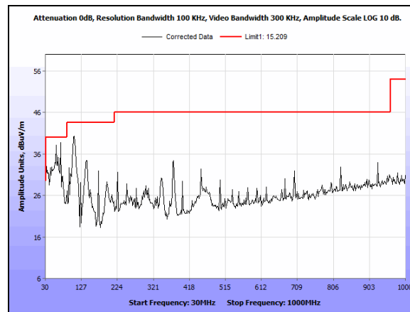
Plot 89. Undesirable Emissions, 30 MHz - 1 GHz 5190 MHz N Mode 40 MHz Port 1
