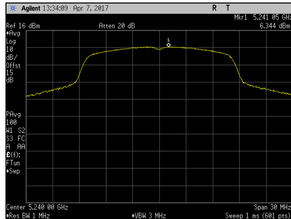
Plot 42. Power Spectral Density, BW 20 M, Ch. 5240 MHz, A mode, Port 1
