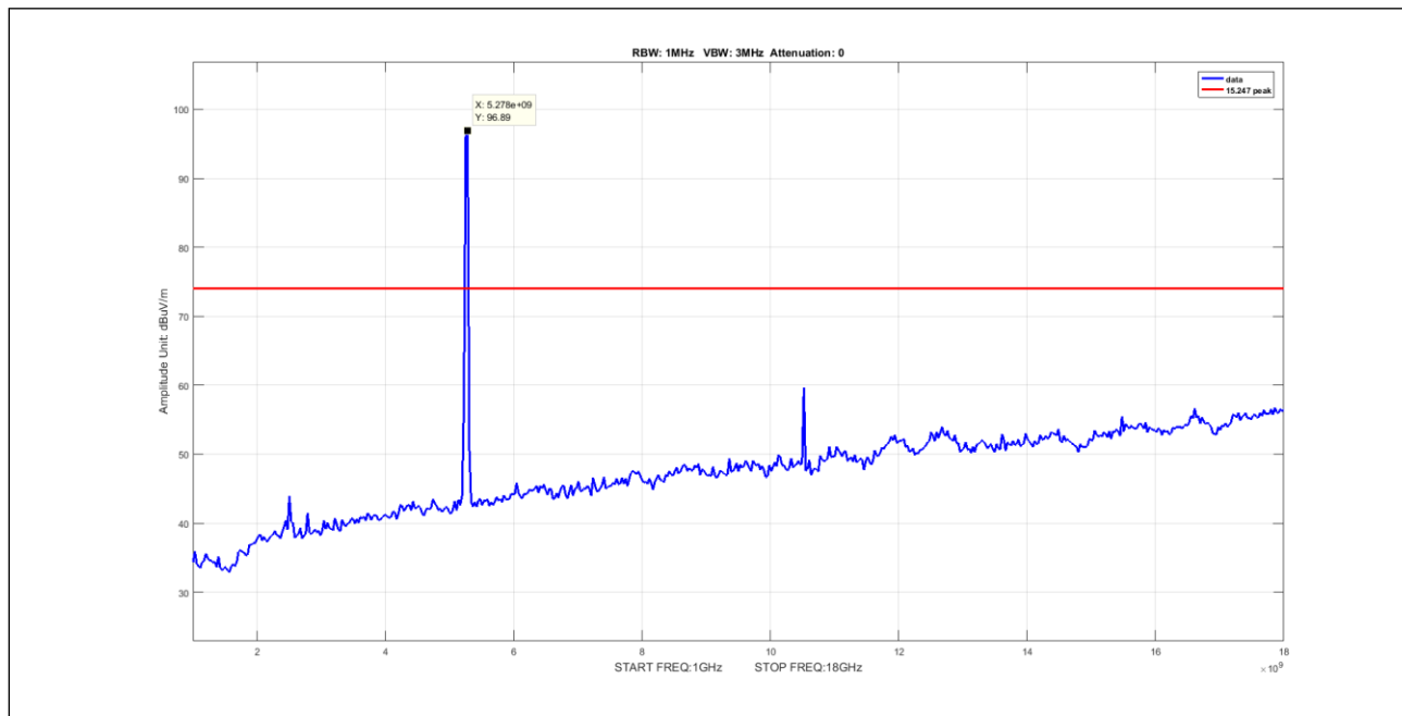
Plot 182. Undesirable Emissions, Peak Spurious Emission 1-18GHz, BW 20M, Ch 5260M, N Mode Port 1
