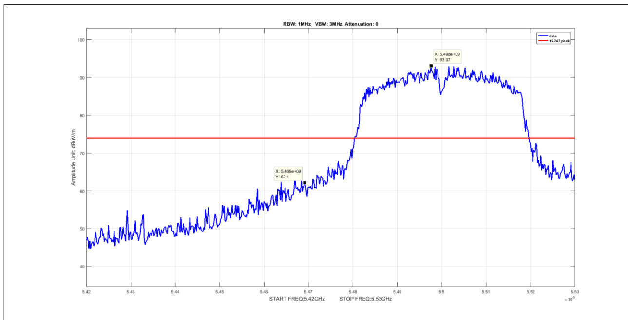
Plot 136. Undesirable Emissions, Peak Band Edge Spurious, BW 40M, Ch 5510M, N Mode Port 1
