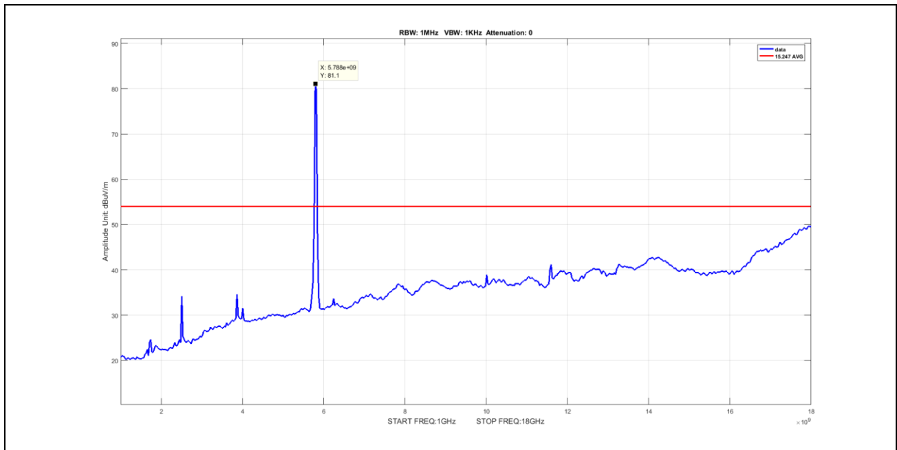
Plot 80. Undesirable Emissions, Average Spurious Emission 1-18GHz, BW 40M, Ch 5795M, N Mode Port 2
