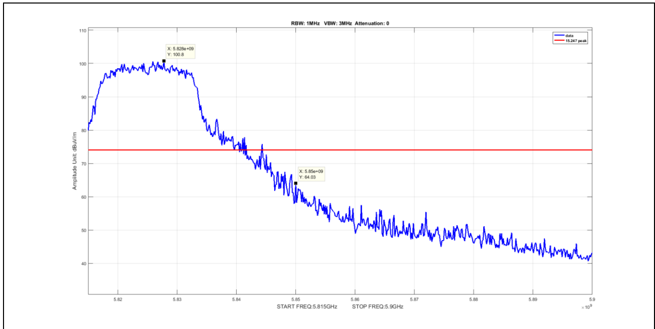
Plot 41. Undesirable Emissions, Peak Band Edge Spurious, BW 20M, Ch 5825M, A Mode Port 2
