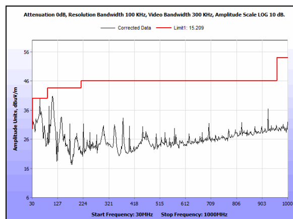
Plot 91. Undesirable Emissions, 30 MHz - 1 GHz 5745 MHz N Mode Port 1
