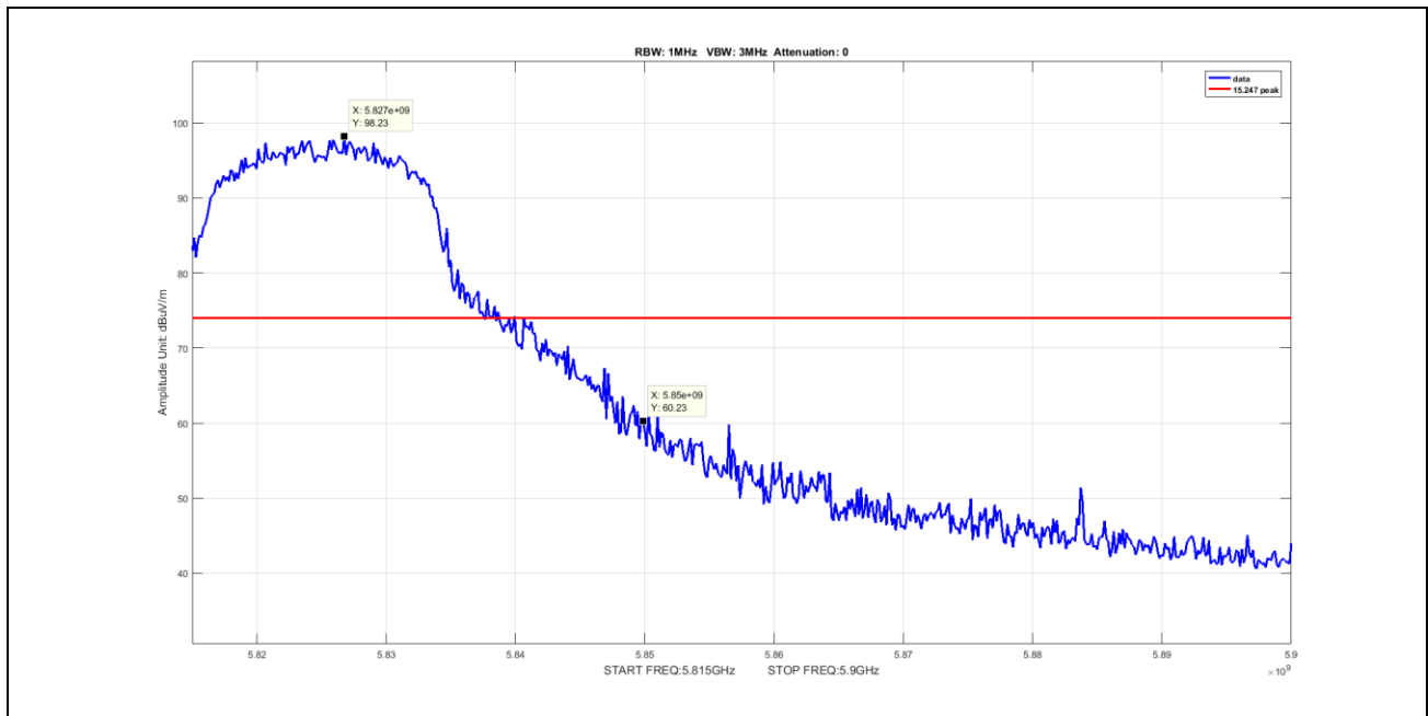
Plot 54. Undesirable Emissions, Peak Band Edge Spurious, BW 20M, Ch 5825M, N Mode
