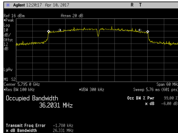
Plot 120. 6 dB Occupied Bandwidth, BW 40M, Ch 5795M, N Mode Port 2
