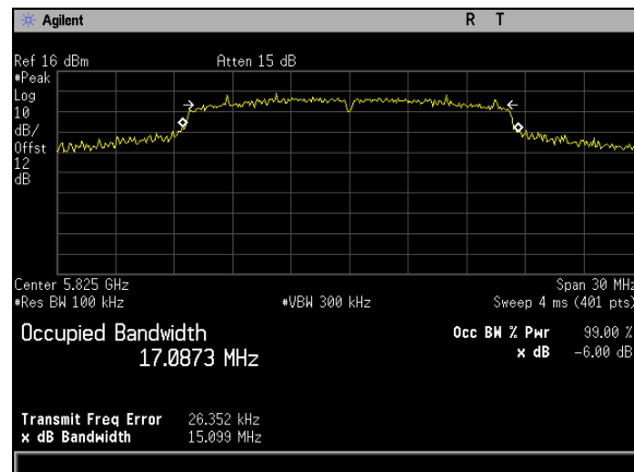
Plot 113. 6 dB Occupied Bandwidth, BW 20M, Ch 5825M, A Mode Port 1
