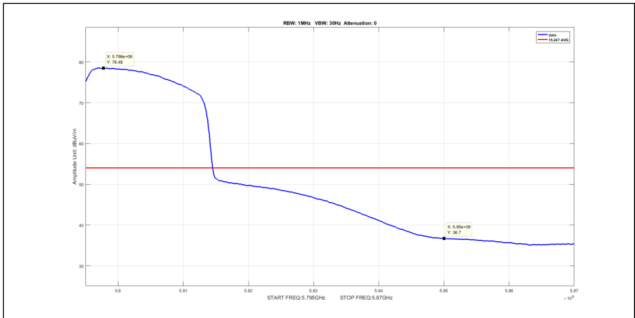
Plot 38. Undesirable Emissions, Average Band Edge Spurious, BW 40M, Ch 5795M, N Mode Port 2
