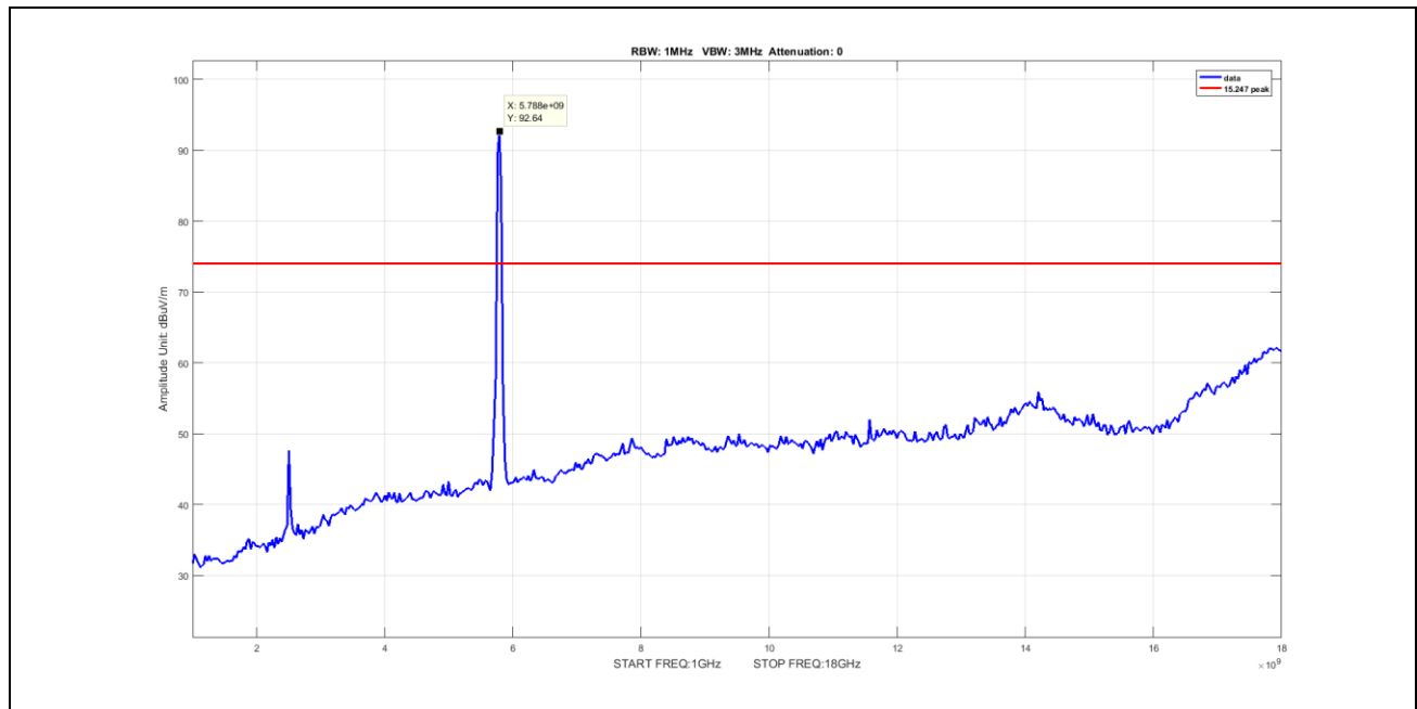
Plot 72. Undesirable Emissions, Peak Spurious Emission 1-18GHz, BW 40M, Ch 5795M, N Mode
