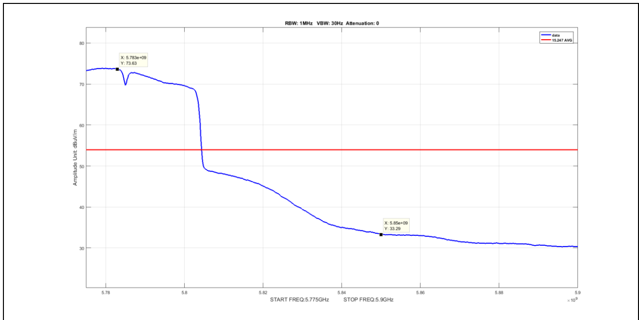
Plot 50. Undesirable Emissions, Average Band Edge Spurious, BW 40M, Ch 5795M, N Mode
