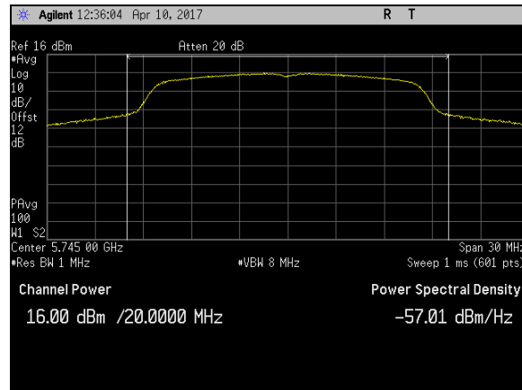
Plot 1. Maximum Conducted Output Power, BW 20M, Ch 5745M, A Mode Port 1
