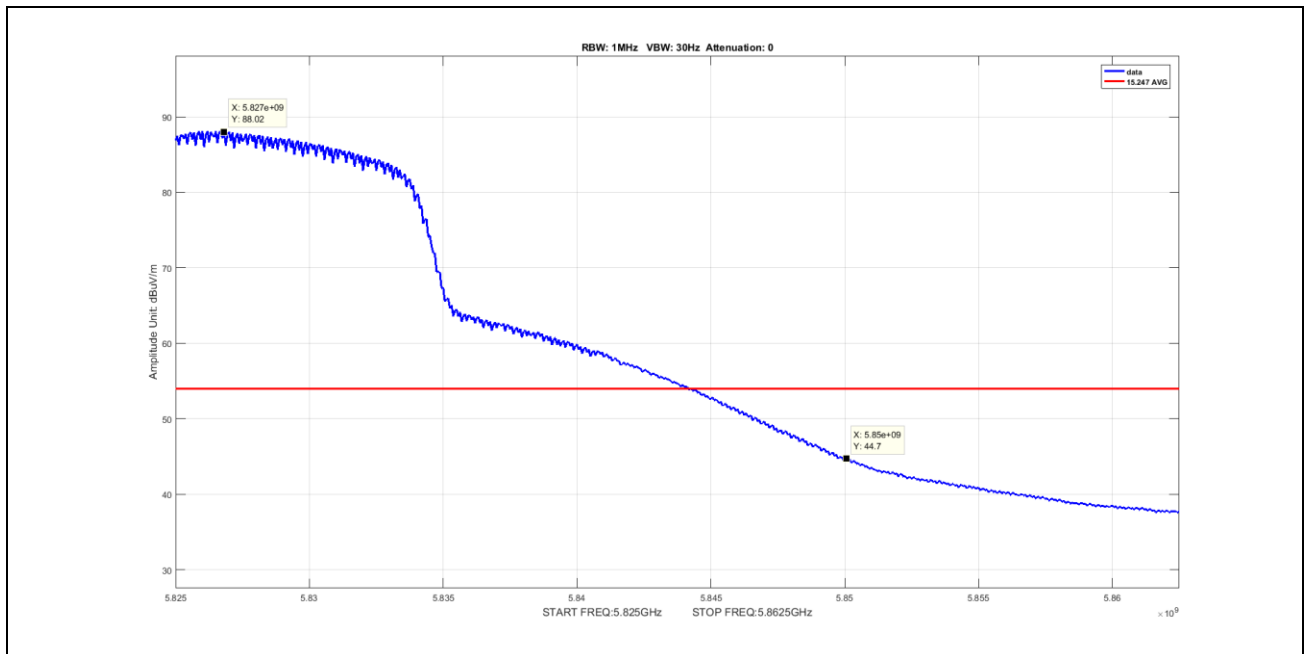
Plot 36. Undesirable Emissions, Average Band Edge Spurious, BW 20M, Ch 5825M, N Mode Port 2
