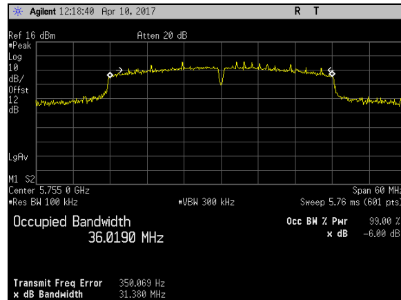
Plot 117. 6 dB Occupied Bandwidth, BW 40M, Ch 5755M, N Mode Port 1
