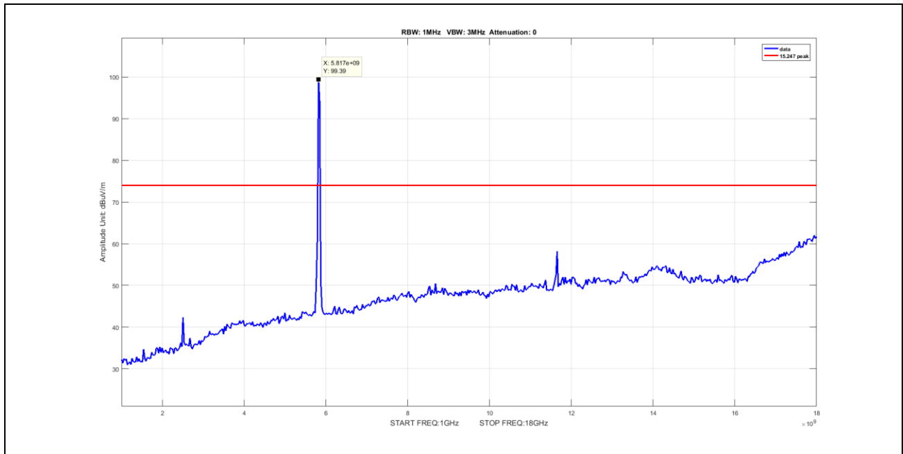
Plot 85. Undesirable Emissions, Peak Spurious Emission 1-18GHz, BW 20M, Ch 5825M, A Mode Port 2
