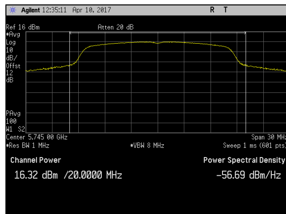
Plot 2. Maximum Conducted Output Power, BW 20M, Ch 5745M, A Mode Port 2
