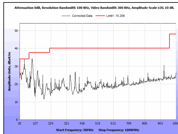
Plot 102. Undesirable Emissions, 30 MHz - 1 GHz 5825 MHz A Mode Port 2
