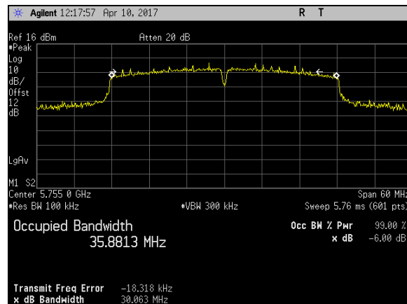
Plot 118. 6 dB Occupied Bandwidth, BW 40M, Ch 5755M, N Mode Port 2
