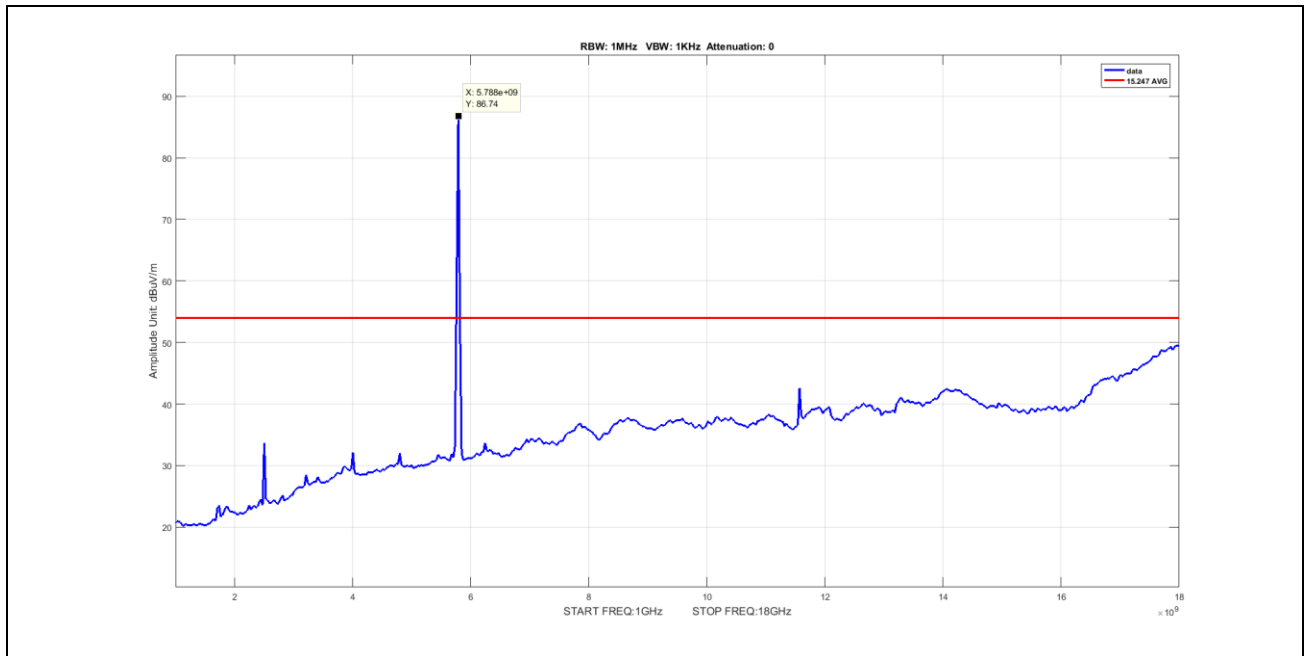
Plot 75. Undesirable Emissions, Average Spurious Emission 1-18GHz, BW 20M, Ch 5785M, A Mode Port 2
