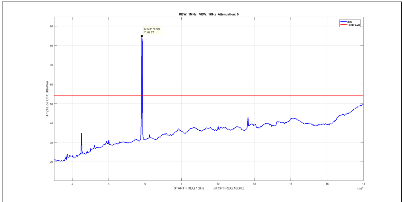
Plot 77. Undesirable Emissions, Average Spurious Emission 1-18GHz, BW 20M, Ch 5825M, A Mode Port 2
