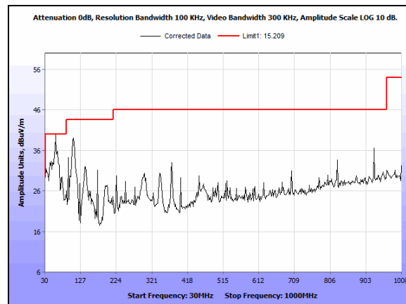
Plot 103. Undesirable Emissions, 30 MHz - 1 GHz 5825 MHz N Mode Port 1
