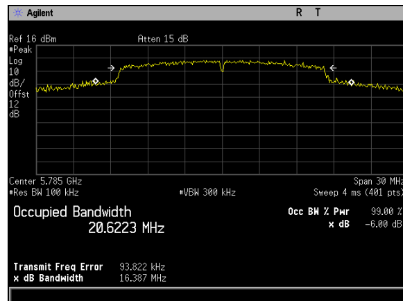
Plot 109. 6 dB Occupied Bandwidth, BW 20M, Ch 5785M, A Mode Port 1
