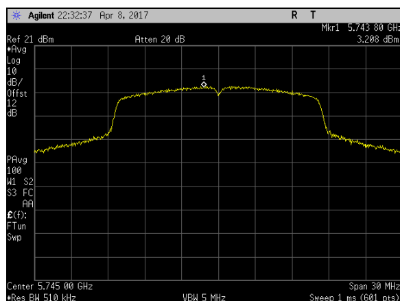
Plot 18. Power Spectral Density, BW 20M, Ch 5745M, A Mode Port 2
