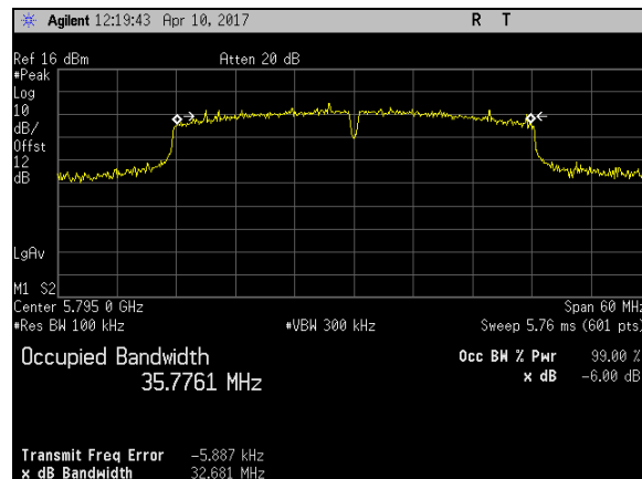
Plot 119. 6 dB Occupied Bandwidth, BW 40M, Ch 5795M, N Mode Port 1
