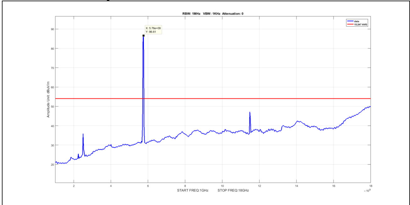
Plot 57. Undesirable Emissions, Average Spurious Emission 1-18GHz, BW 20M, Ch 5745M, A Mode
