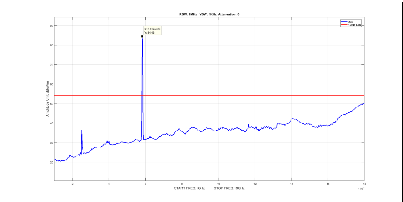
Plot 61. Undesirable Emissions, Average Spurious Emission 1-18GHz, BW 20M, Ch 5825M, A Mode
