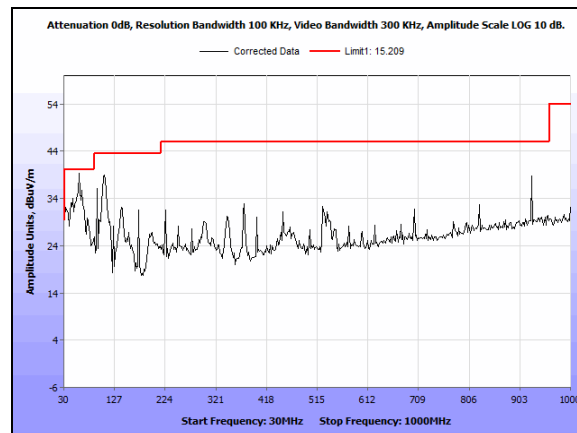
Plot 94. Undesirable Emissions, 30 MHz - 1 GHz 5755 MHz N Mode Port 2
