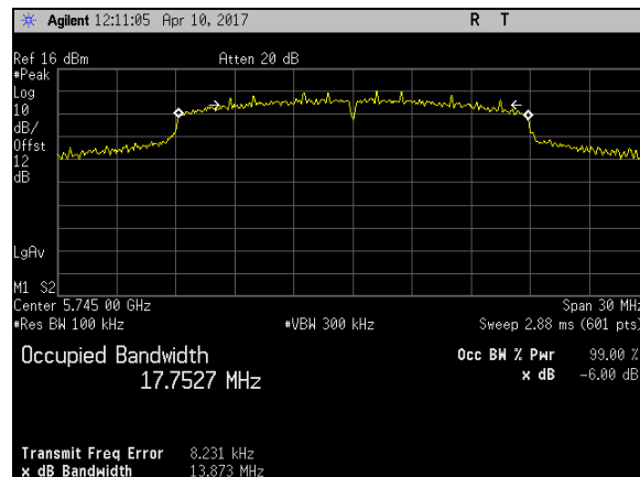
Plot 107. 6 dB Occupied Bandwidth, BW 20M, Ch 5745M, N Mode Port 1
