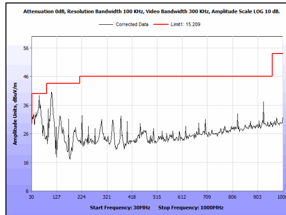
Plot 104. Undesirable Emissions, 30 MHz - 1 GHz 5825 MHz N Mode Port 2
