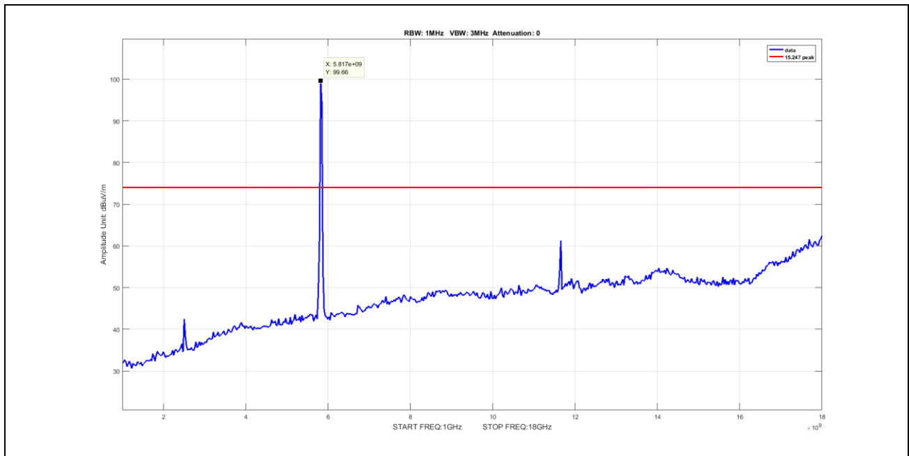
Plot 86. Undesirable Emissions, Peak Spurious Emission 1-18GHz, BW 20M, Ch 5825M, N Mode Port 2
