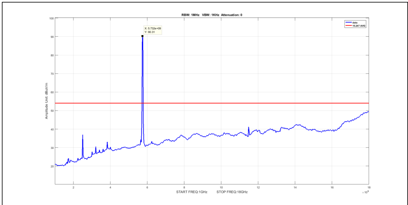
Plot 74. Undesirable Emissions, Average Spurious Emission 1-18GHz, BW 20M, Ch 5745M, N Mode Port 2
