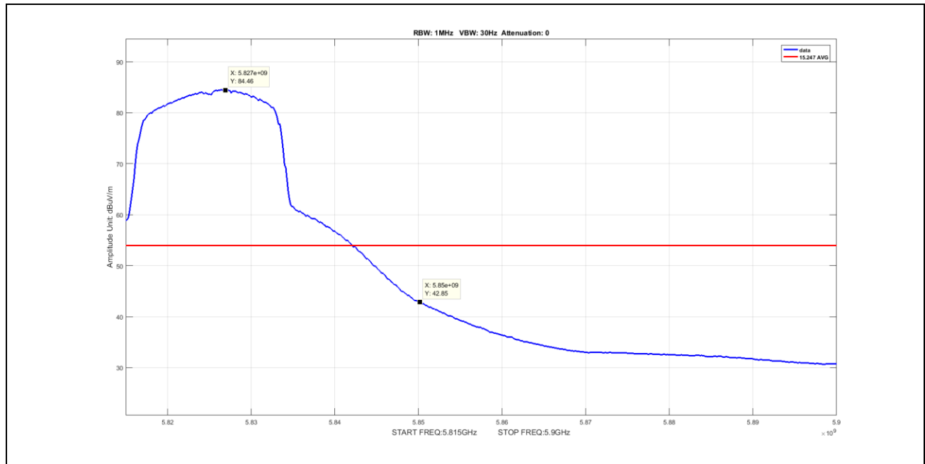
Plot 47. Undesirable Emissions, Average Band Edge Spurious, BW 20M, Ch 5825M, A Mode
