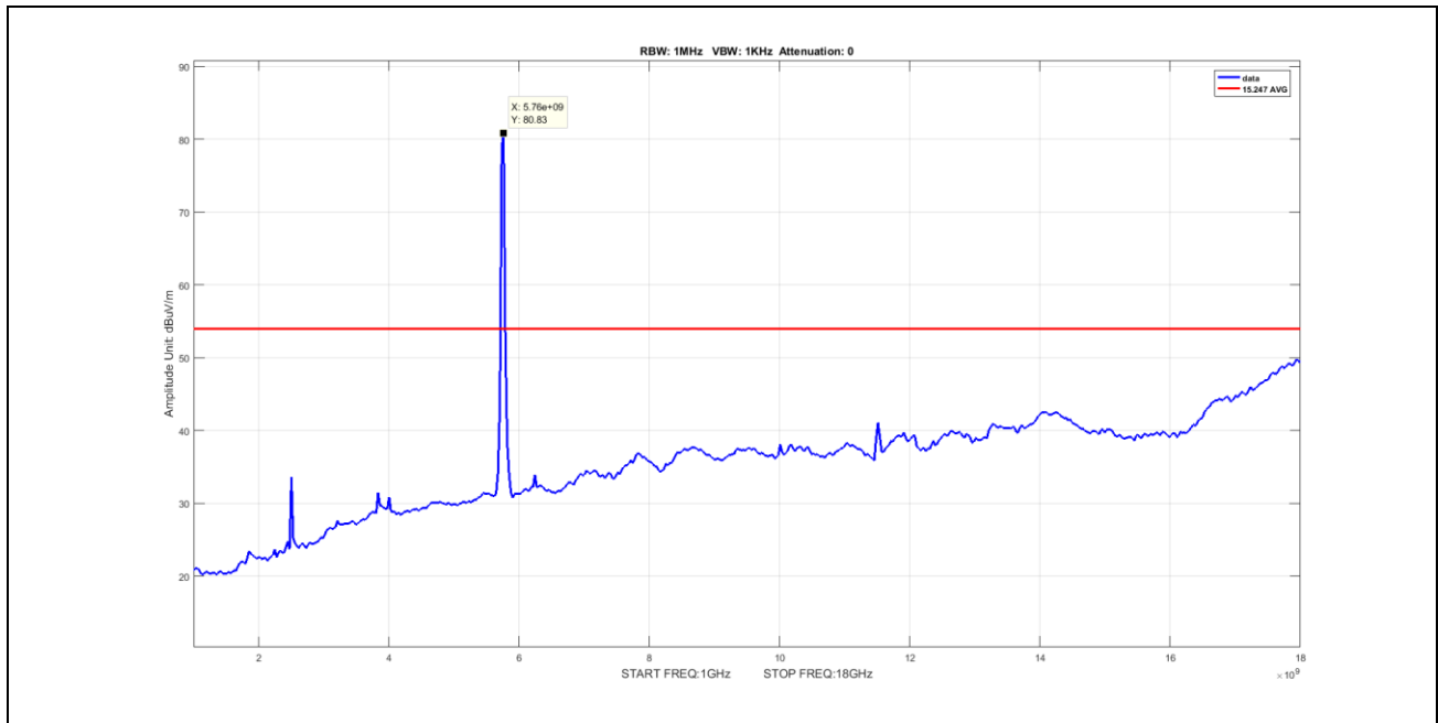
Plot 79. Undesirable Emissions, Average Spurious Emission 1-18GHz, BW 40M, Ch 5755M, N Mode Port 2
