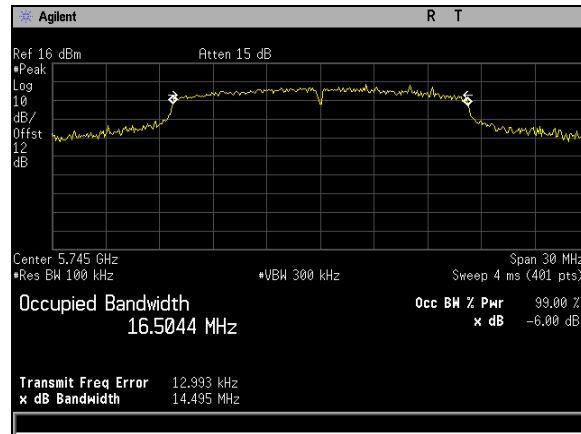
Plot 105. 6 dB Occupied Bandwidth, BW 20M, Ch 5745M, A Mode Port 1
