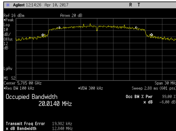
Plot 111. 6 dB Occupied Bandwidth, BW 20M, Ch 5785M, N Mode Port 1
