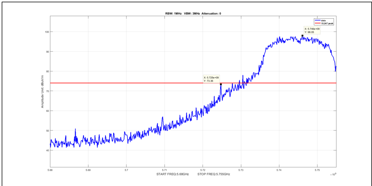
Plot 52. Undesirable Emissions, Peak Band Edge Spurious, BW 20M, Ch 5745M, N Mode
