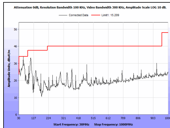
Plot 97. Undesirable Emissions, 30 MHz - 1 GHz 5785 MHz N Mode Port 1
