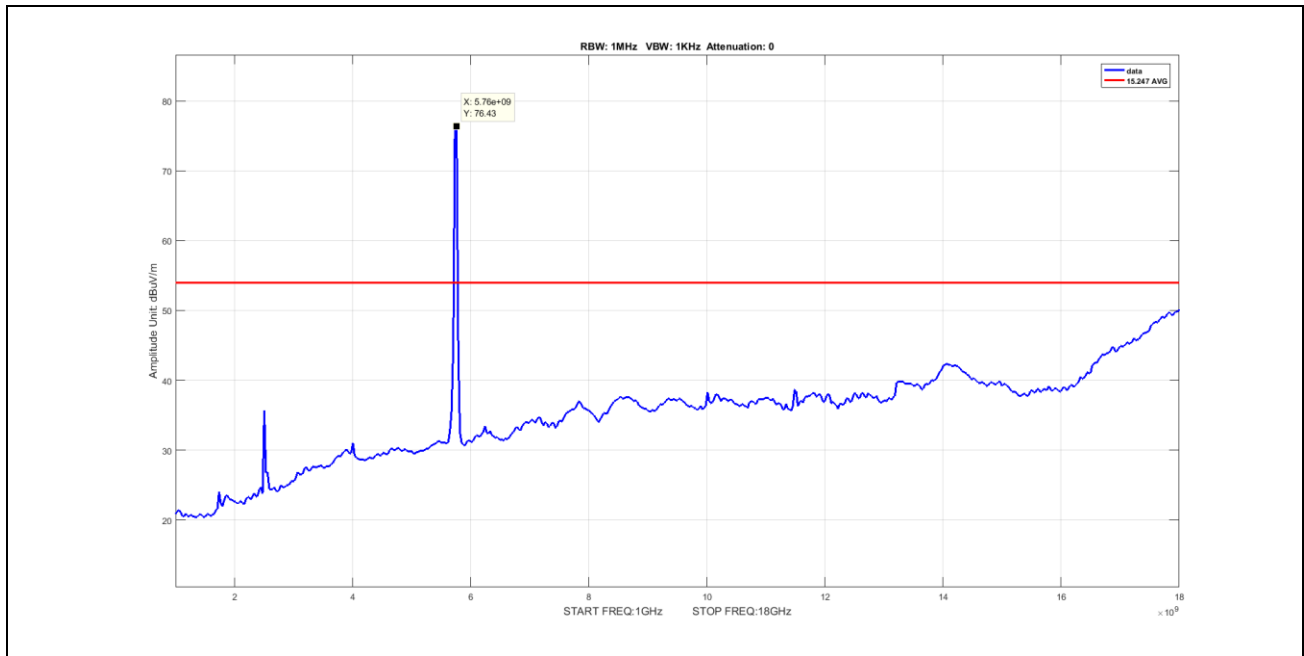
Plot 63. Undesirable Emissions, Average Spurious Emission 1-18GHz, BW 40M, Ch 5755M, N Mode
