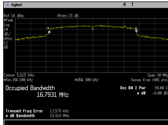
Plot 114. 6 dB Occupied Bandwidth, BW 20M, Ch 5825M, A Mode Port 2
