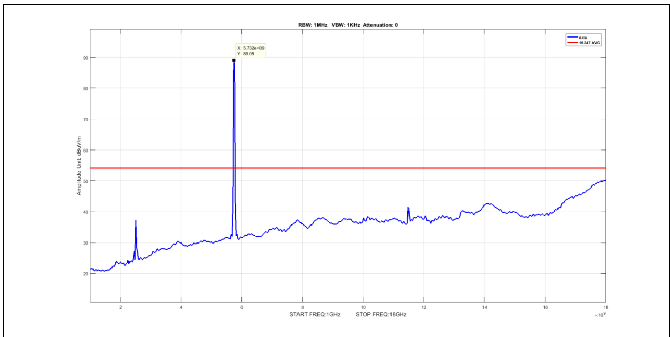
Plot 58. Undesirable Emissions, Average Spurious Emission 1-18GHz, BW 20M, Ch 5745M, N Mode
