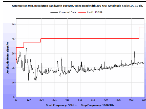
Plot 98. Undesirable Emissions, 30 MHz - 1 GHz 5785 MHz N Mode Port 2
