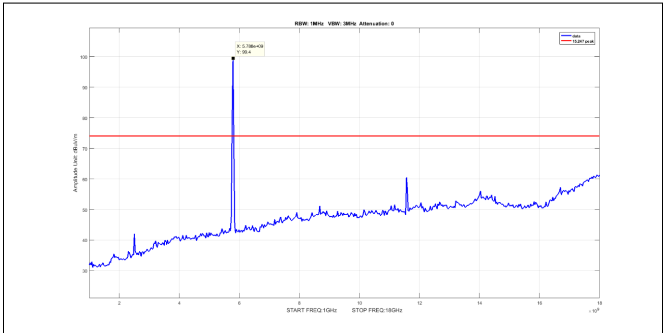
Plot 83. Undesirable Emissions, Peak Spurious Emission 1-18GHz, BW 20M, Ch 5785M, A Mode Port 2
