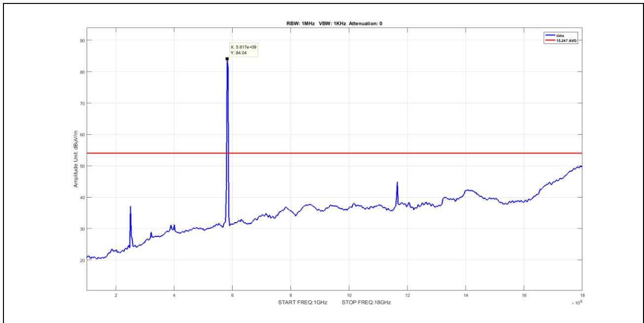
Plot 62. Undesirable Emissions, Average Spurious Emission 1-18GHz, BW 20M, Ch 5825M, N Mode
