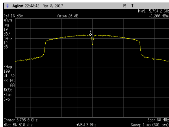
Plot 32. Power Spectral Density, BW 40M, Ch 5795M, N Mode Port 2
