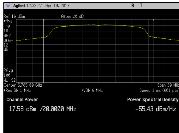
Plot 6. Maximum Conducted Output Power, BW 20M, Ch 5785M, A Mode Port 2
