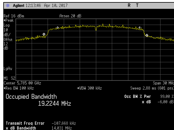
Plot 112. 6 dB Occupied Bandwidth, BW 20M, Ch 5785M, N Mode Port 2
