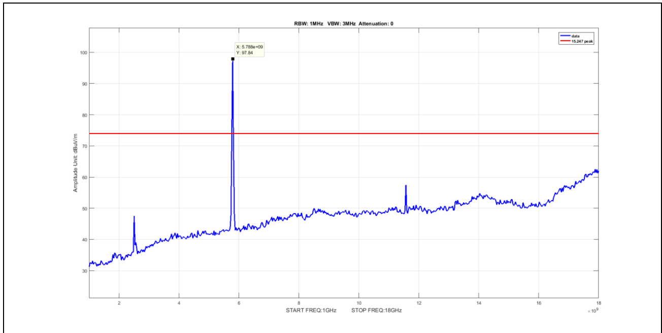
Plot 67. Undesirable Emissions, Peak Spurious Emission 1-18GHz, BW 20M, Ch 5785M, A Mode
