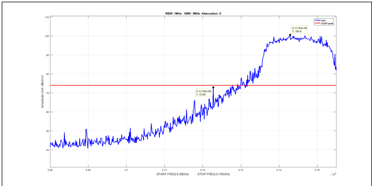
Plot 40. Undesirable Emissions, Peak Band Edge Spurious, BW 20M, Ch 5745M, N Mode Port 2
