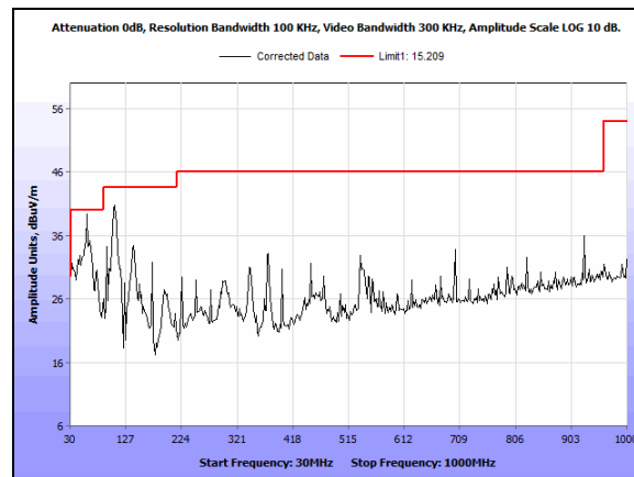
Plot 96. Undesirable Emissions, 30 MHz - 1 GHz 5785 MHz A Mode Port 2
