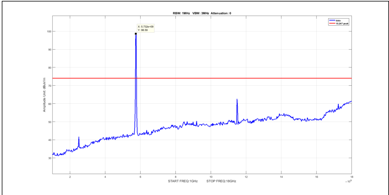
Plot 81. Undesirable Emissions, Peak Spurious Emission 1-18GHz, BW 20M, Ch 5745M, A Mode Port 2
