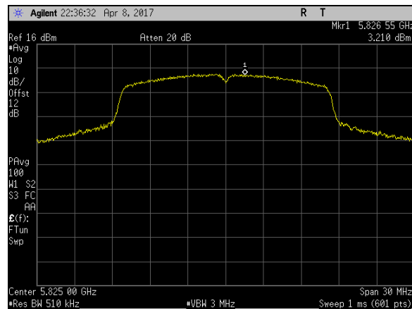
Plot 26. Power Spectral Density, BW 20M, Ch 5825M, A Mode Port 2
