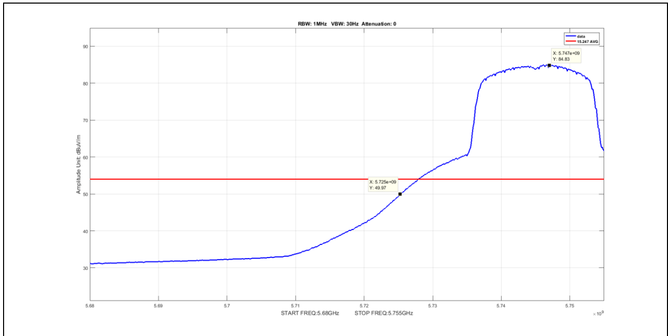
Plot 45. Undesirable Emissions, Average Band Edge Spurious, BW 20M, Ch 5745M, A Mode
