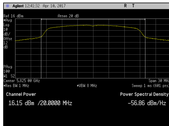
Plot 11. Maximum Conducted Output Power, BW 20M, Ch 5825M, N Mode Port 1
