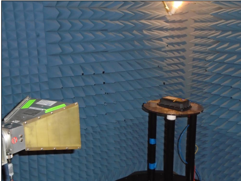
Photograph 1. Undesirable Emissions, Set up Above 1 GHz
