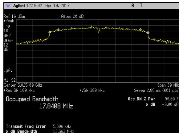
Plot 116. 6 dB Occupied Bandwidth, BW 20M, Ch 5825M, N Mode Port 2
