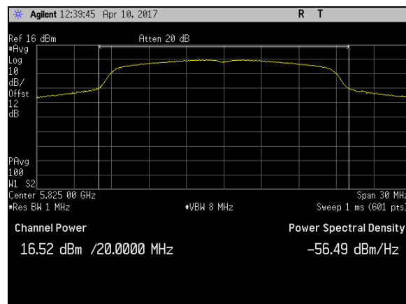
Plot 12. Maximum Conducted Output Power, BW 20M, Ch 5825M, N Mode Port 2
