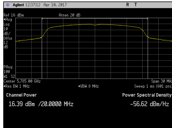
Plot 7. Maximum Conducted Output Power, BW 20M, Ch 5785M, N Mode Port 1
