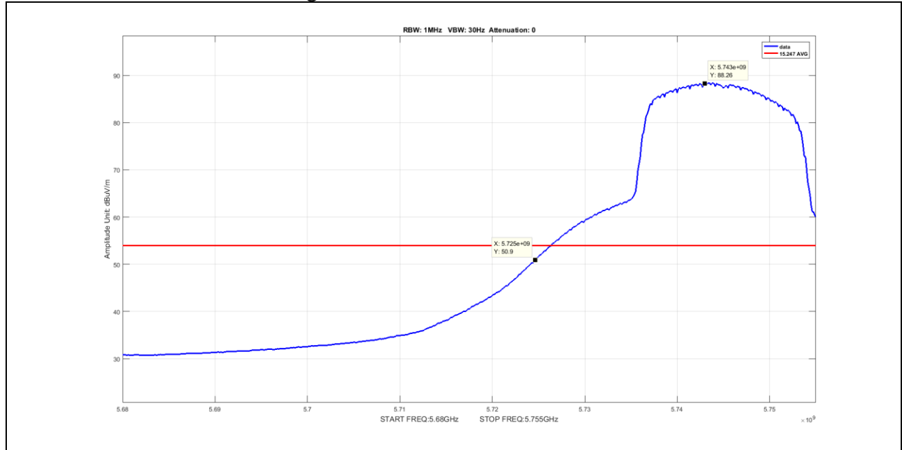
Plot 33. Undesirable Emissions, Average Band Edge Spurious, BW 20M, Ch 5745M, A Mode Port 2
