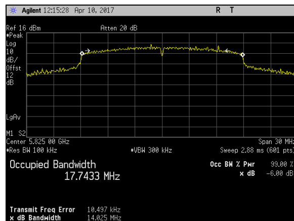
Plot 115. 6 dB Occupied Bandwidth, BW 20M, Ch 5825M, N Mode Port 1
