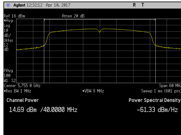
Plot 13. Maximum Conducted Output Power, BW 40M, Ch 5755M, N Mode Port 1
