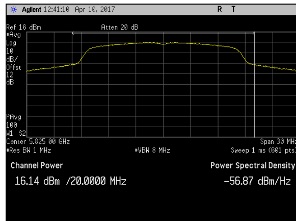
Plot 9. Maximum Conducted Output Power, BW 20M, Ch 5825M, A Mode Port 1
