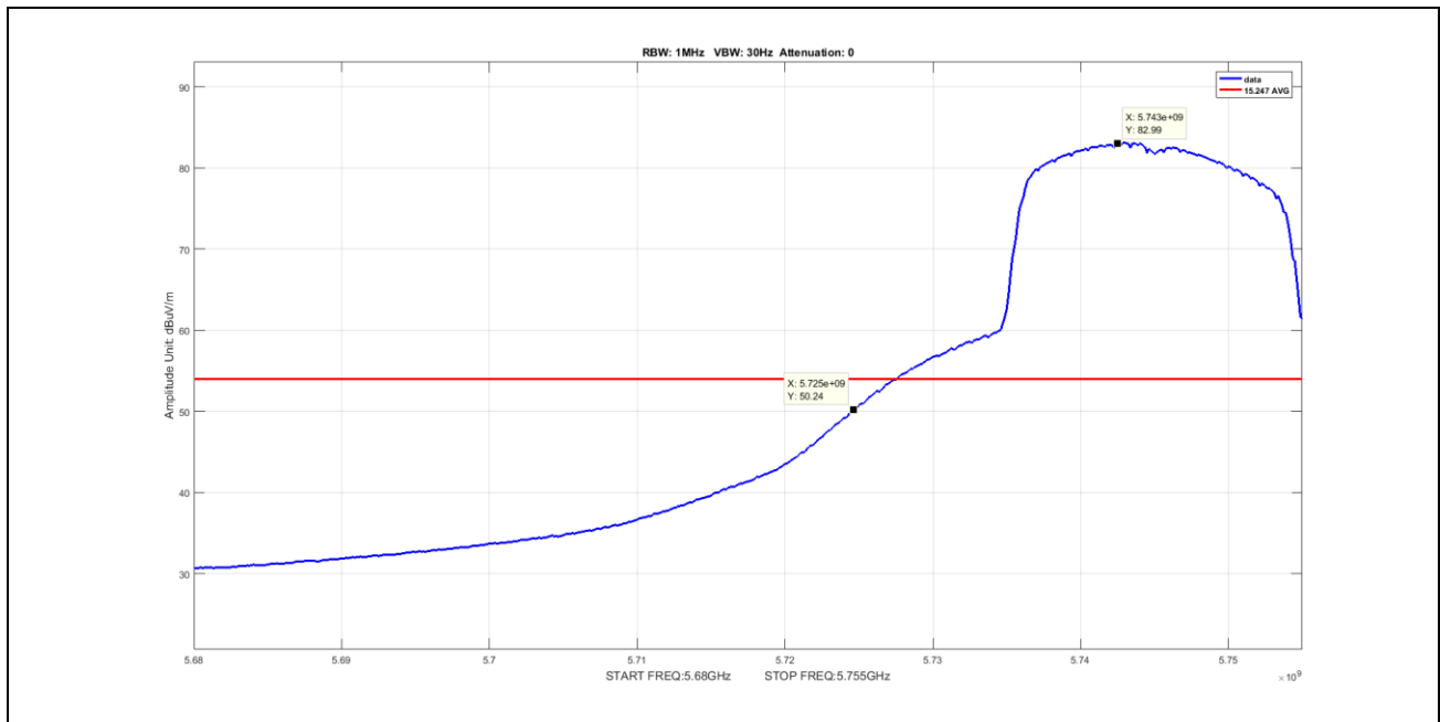
Plot 46. Undesirable Emissions, Average Band Edge Spurious, BW 20M, Ch 5745M, N Mode
