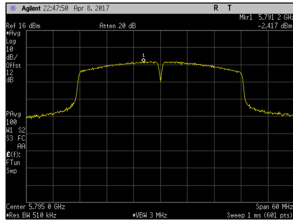
Plot 31. Power Spectral Density, BW 40M, Ch 5795M, N Mode Port 1
