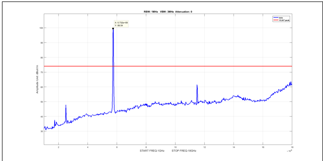
Plot 66. Undesirable Emissions, Peak Spurious Emission 1-18GHz, BW 20M, Ch 5745M, N Mode
