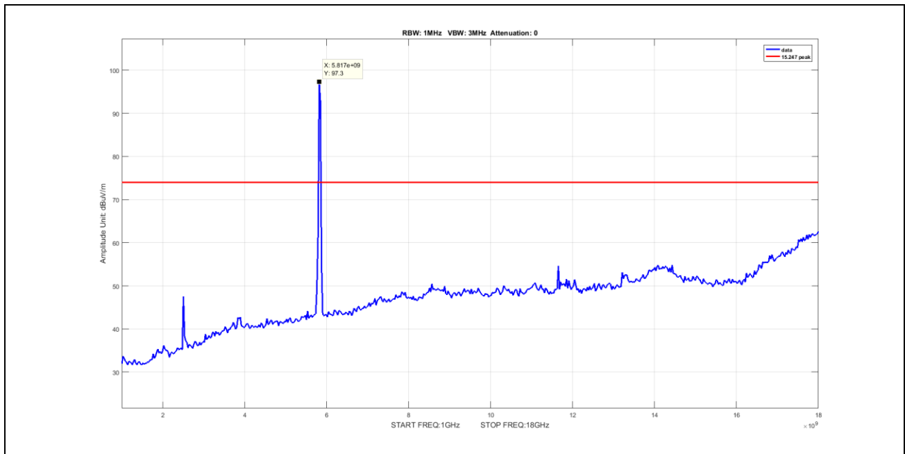
Plot 70. Undesirable Emissions, Peak Spurious Emission 1-18GHz, BW 20M, Ch 5825M, N Mode
