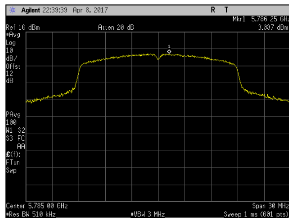
Plot 23. Power Spectral Density, BW 20M, Ch 5785M, N Mode Port 1
