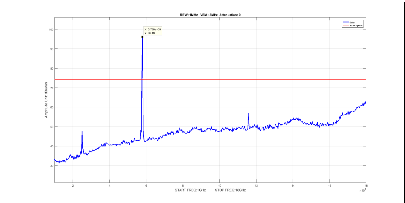
Plot 68. Undesirable Emissions, Peak Spurious Emission 1-18GHz, BW 20M, Ch 5785M, N Mode
