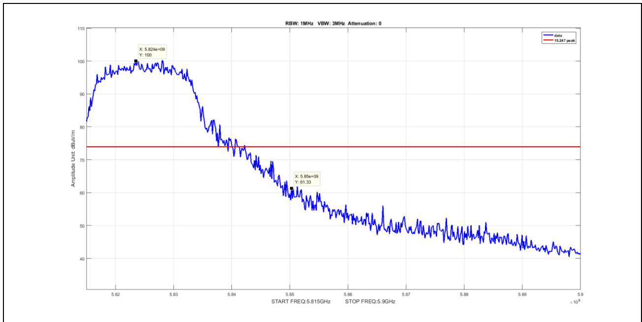
Plot 42. Undesirable Emissions, Peak Band Edge Spurious, BW 20M, Ch 5825M, N Mode Port 2
