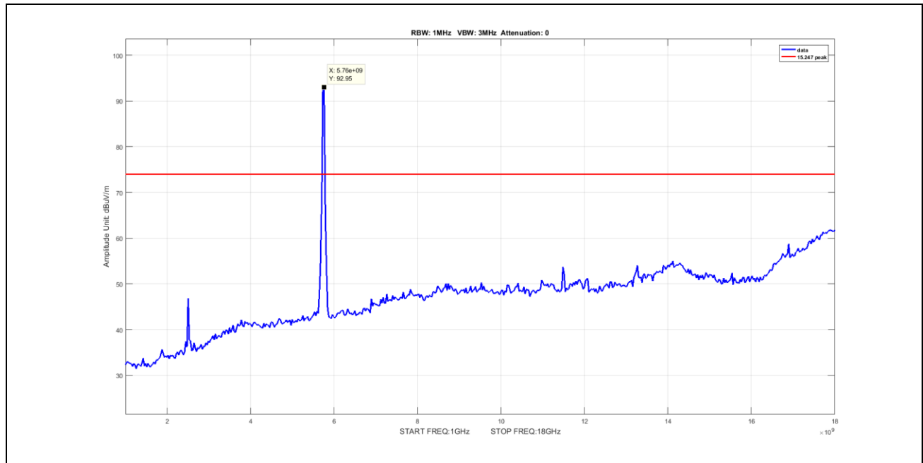
Plot 71. Undesirable Emissions, Peak Spurious Emission 1-18GHz, BW 40M, Ch 5755M, N Mode
