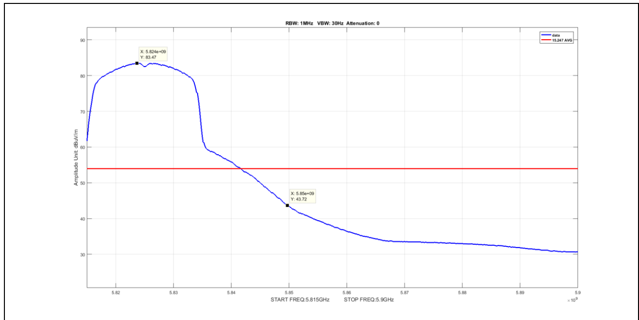
Plot 48. Undesirable Emissions, Average Band Edge Spurious, BW 20M, Ch 5825M, N Mode
