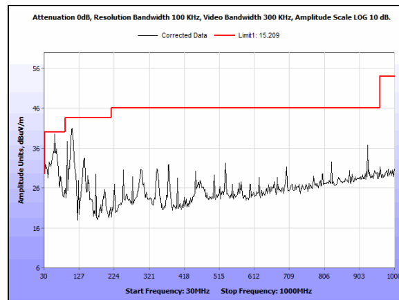
Plot 93. Undesirable Emissions, 30 MHz - 1 GHz 5755 MHz N Mode Port 1
