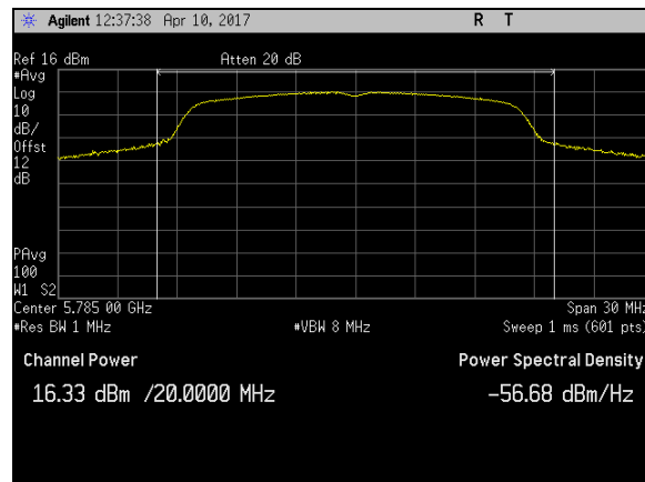
Plot 5. Maximum Conducted Output Power, BW 20M, Ch 5785M, A Mode Port 1
