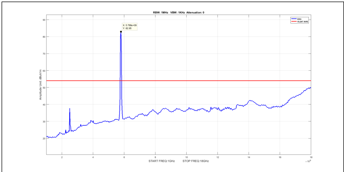
Plot 64. Undesirable Emissions, Average Spurious Emission 1-18GHz, BW 40M, Ch 5795M, N Mode
