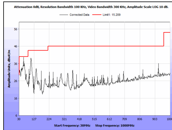
Plot 95. Undesirable Emissions, 30 MHz - 1 GHz 5785 MHz A Mode Port 1
