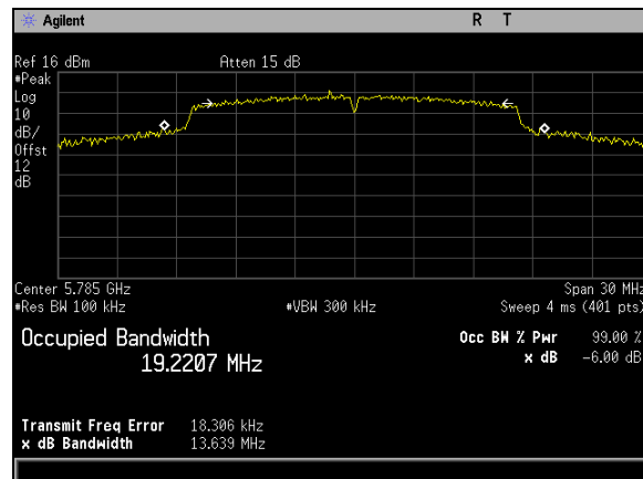
Plot 110. 6 dB Occupied Bandwidth, BW 20M, Ch 5785M, A Mode Port 2
