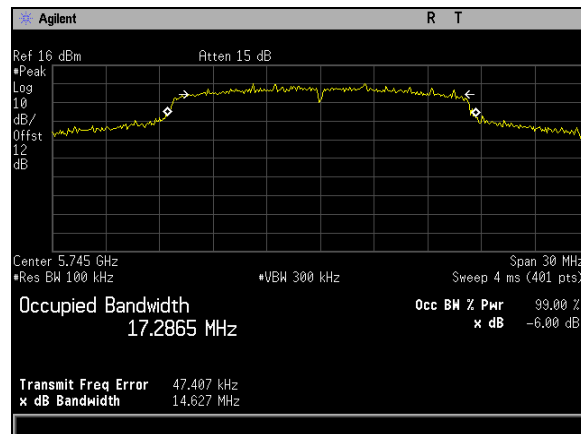
Plot 106. 6 dB Occupied Bandwidth, BW 20M, Ch 5745M, A Mode Port 2
