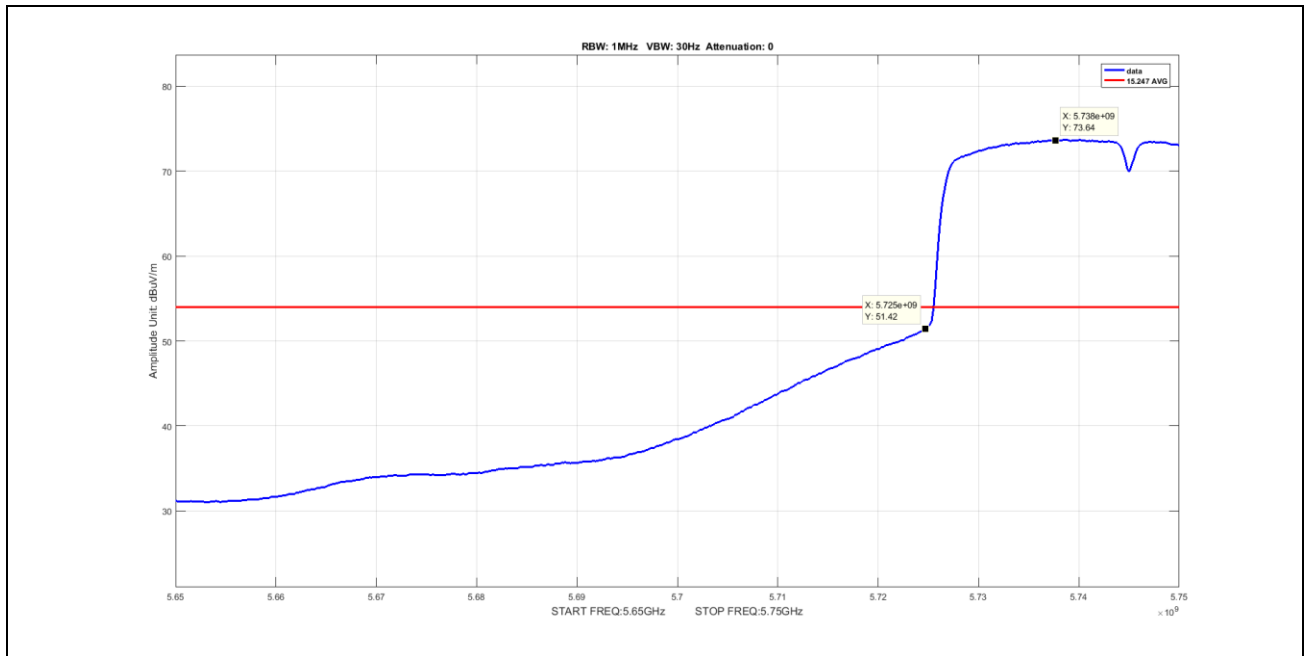
Plot 49. Undesirable Emissions, Average Band Edge Spurious, BW 40M, Ch 5755M, N Mode
