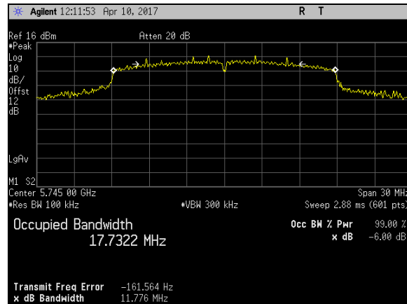
Plot 108. 6 dB Occupied Bandwidth, BW 20M, Ch 5745M, N Mode Port 2
