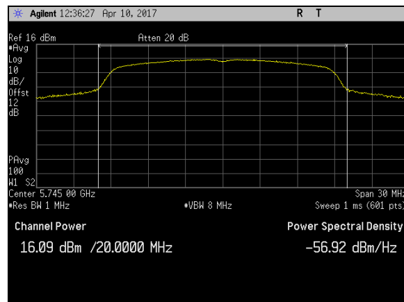
Plot 3. Maximum Conducted Output Power, BW 20M, Ch 5745M, N Mode Port 1
