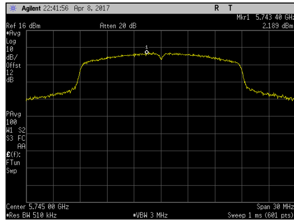
Plot 19. Power Spectral Density, BW 20M, Ch 5745M, N Mode Port 1
