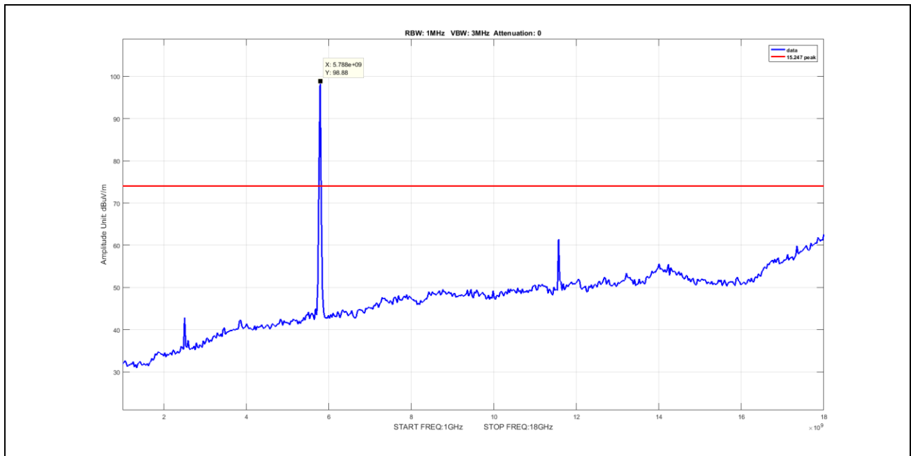
Plot 84. Undesirable Emissions, Peak Spurious Emission 1-18GHz, BW 20M, Ch 5785M, N Mode Port 2
