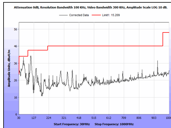
Plot 99. Undesirable Emissions, 30 MHz - 1 GHz 5795 MHz N Mode Port 1
