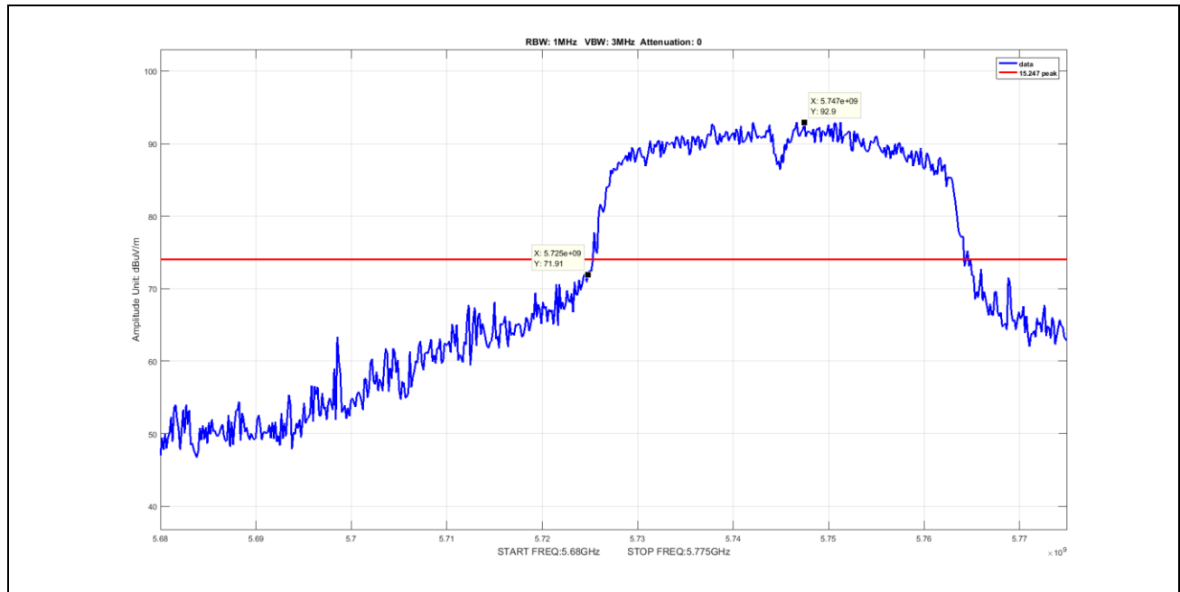
Plot 55. Undesirable Emissions, Peak Band Edge Spurious, BW 40M, Ch 5755M, N Mode
