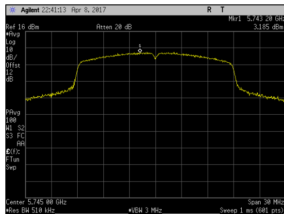
Plot 20. Power Spectral Density, BW 20M, Ch 5745M, N Mode Port 2
