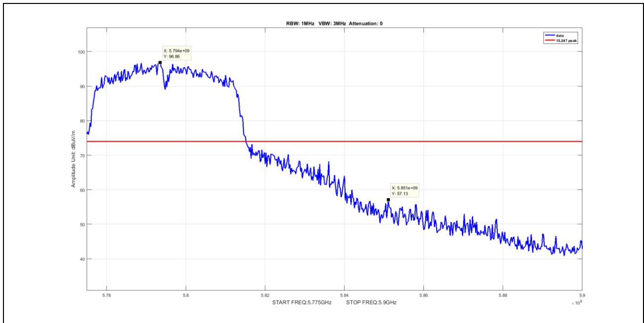
Plot 44. Undesirable Emissions, Peak Band Edge Spurious, BW 40M, Ch 5795M, N Mode Port 2
