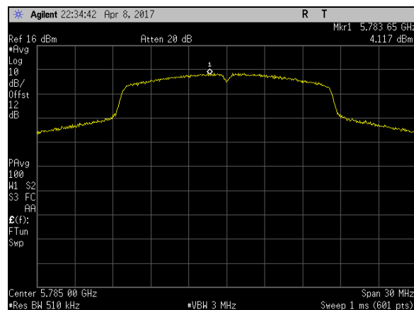
Plot 21. Power Spectral Density, BW 20M, Ch 5785M, A Mode Port 1
