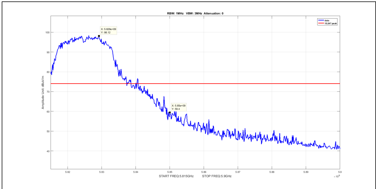
Plot 53. Undesirable Emissions, Peak Band Edge Spurious, BW 20M, Ch 5825M, A Mode
