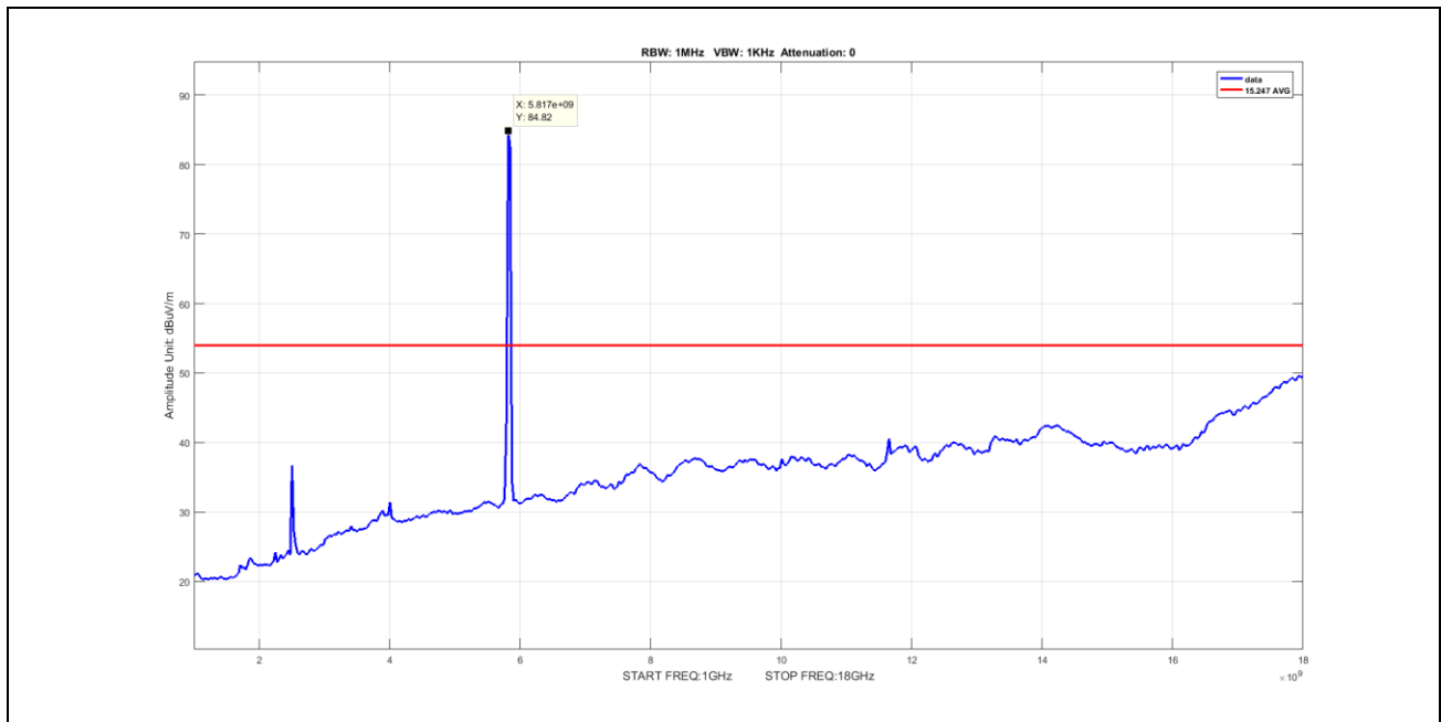
Plot 78. Undesirable Emissions, Average Spurious Emission 1-18GHz, BW 20M, Ch 5825M, N Mode Port 2
