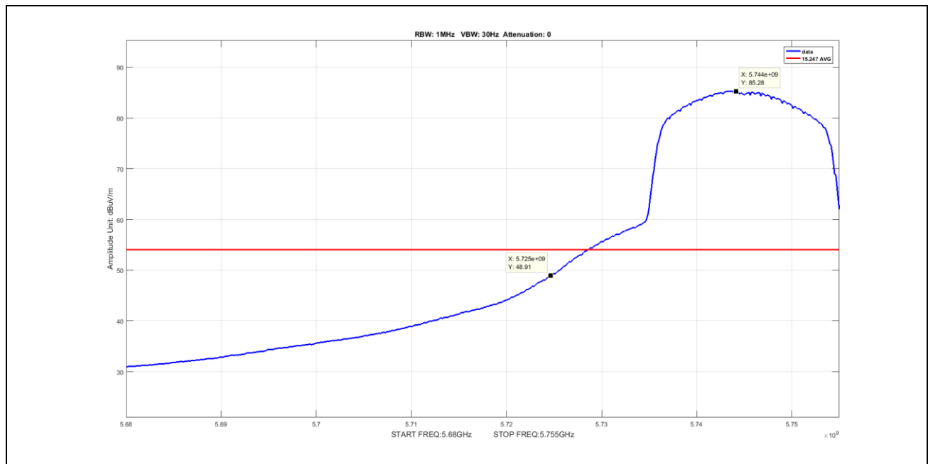
Plot 34. Undesirable Emissions, Average Band Edge Spurious, BW 20M, Ch 5745M, N Mode Port 2
