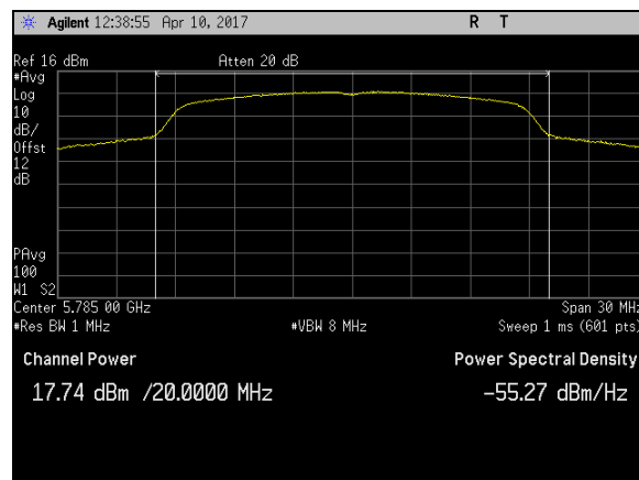
Plot 8. Maximum Conducted Output Power, BW 20M, Ch 5785M, N Mode Port 2
