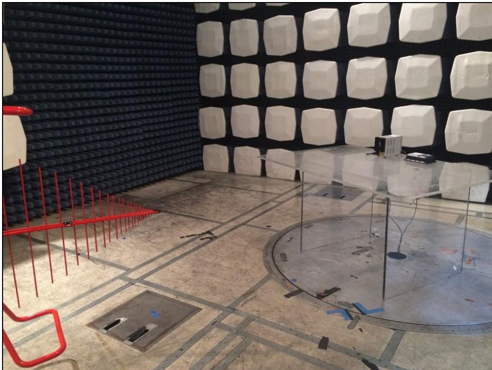
Photograph 2. Undesirable Emissions, Set up Below 1 GHz
