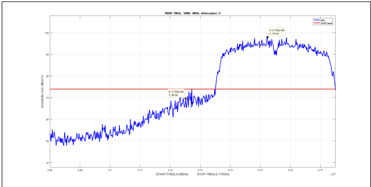
Plot 43. Undesirable Emissions, Peak Band Edge Spurious, BW 40M, Ch 5755M, N Mode Port 2
