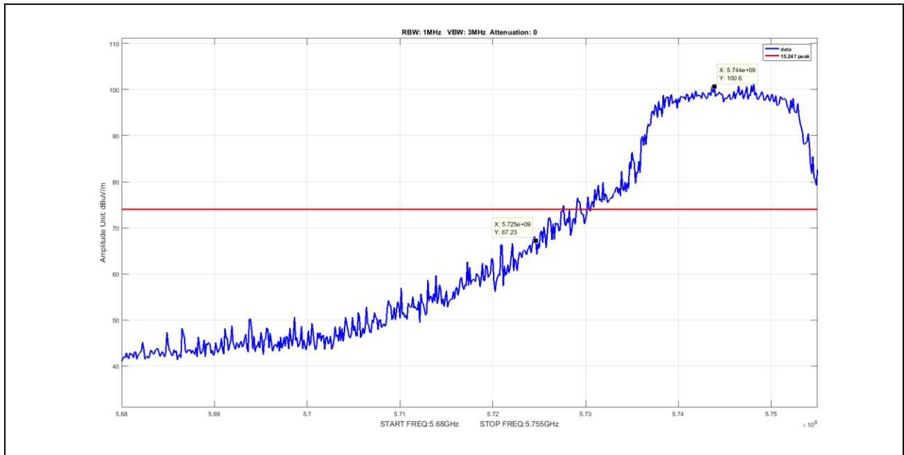
Plot 39. Undesirable Emissions, Peak Band Edge Spurious, BW 20M, Ch 5745M, A Mode Port 2
