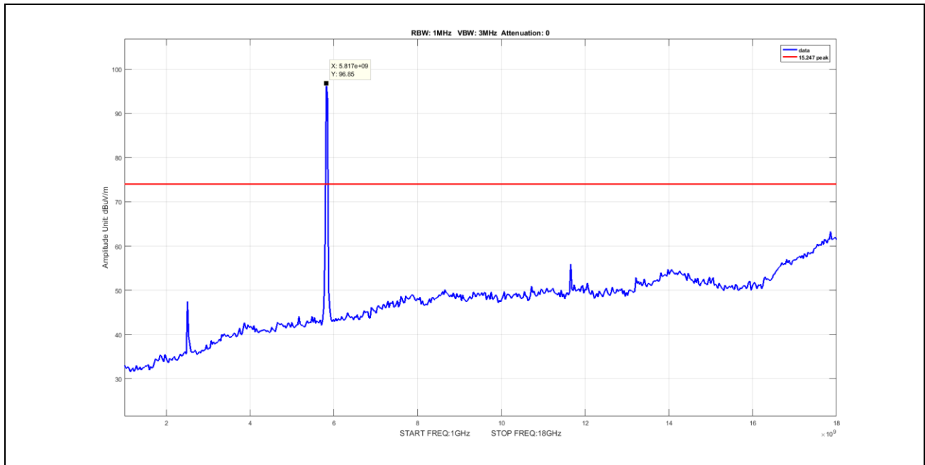
Plot 69. Undesirable Emissions, Peak Spurious Emission 1-18GHz, BW 20M, Ch 5825M, A Mode
