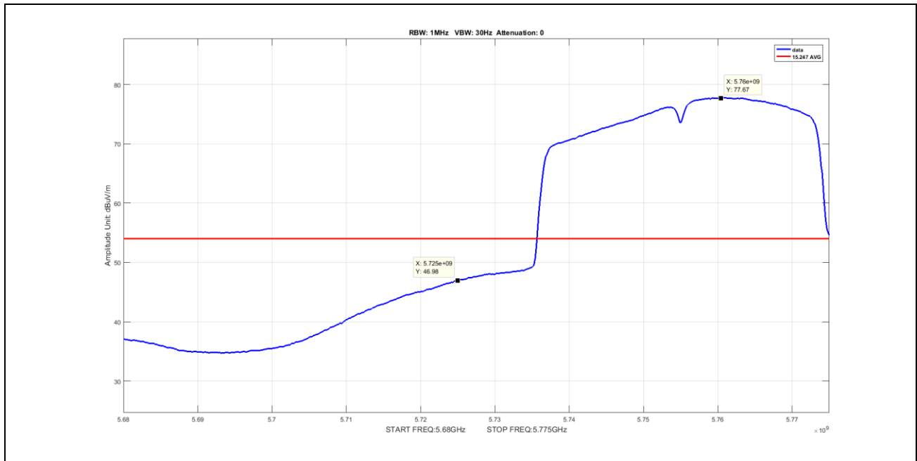
Plot 37. Undesirable Emissions, Average Band Edge Spurious, BW 40M, Ch 5755M, N Mode Port 2
