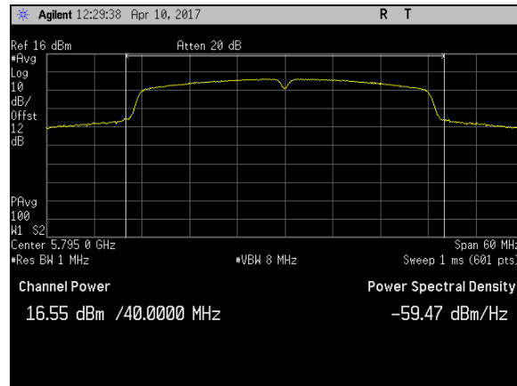
Plot 16. Maximum Conducted Output Power, BW 40M, Ch 5795M, N Mode Port 2
