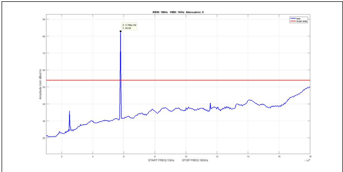
Plot 59. Undesirable Emissions, Average Spurious Emission 1-18GHz, BW 20M, Ch 5785M, A Mode
