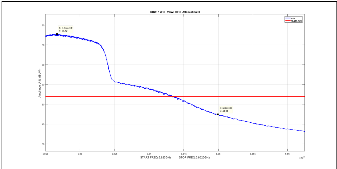
Plot 35. Undesirable Emissions, Average Band Edge Spurious, BW 20M, Ch 5825M, A Mode Port 2
