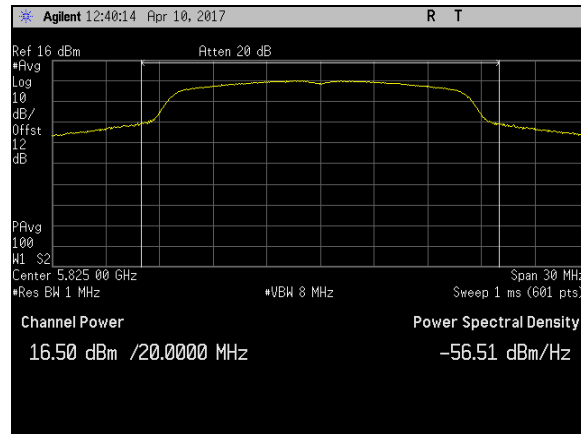
Plot 10. Maximum Conducted Output Power, BW 20M, Ch 5825M, A Mode Port 2
