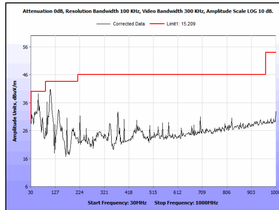
Plot 92. Undesirable Emissions, 30 MHz - 1 GHz 5745 MHz N Mode Port 2
