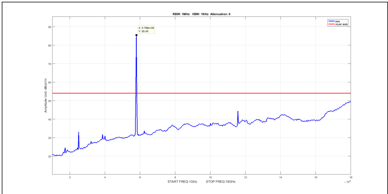
Plot 76. Undesirable Emissions, Average Spurious Emission 1-18GHz, BW 20M, Ch 5785M, N Mode Port 2
