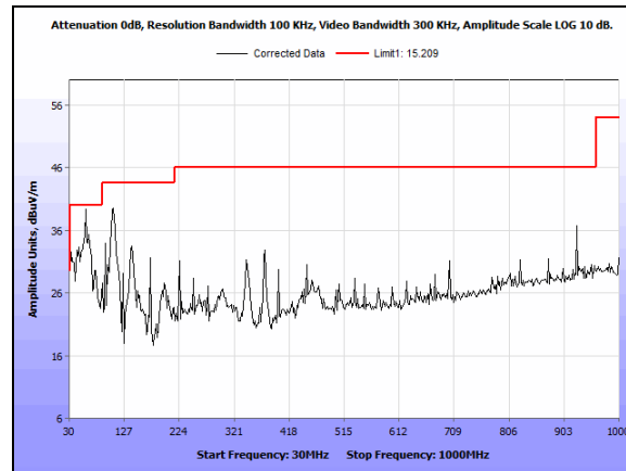
Plot 101. Undesirable Emissions, 30 MHz - 1 GHz 5825 MHz A Mode Port 1
