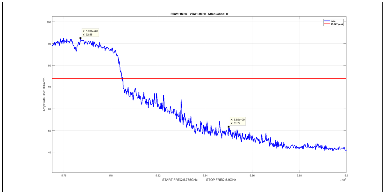
Plot 56. Undesirable Emissions, Peak Band Edge Spurious, BW 40M, Ch 5795M, N Mode
