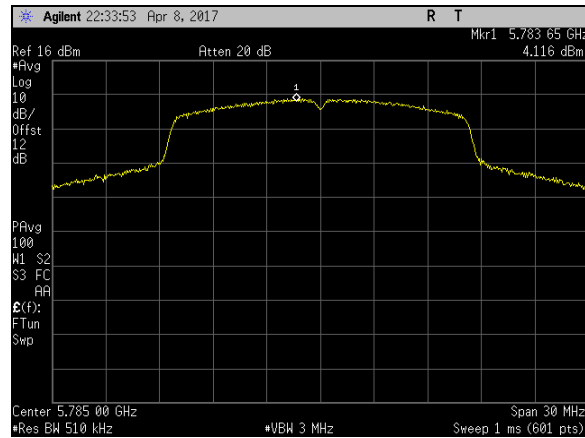
Plot 22. Power Spectral Density, BW 20M, Ch 5785M, A Mode Port 2
