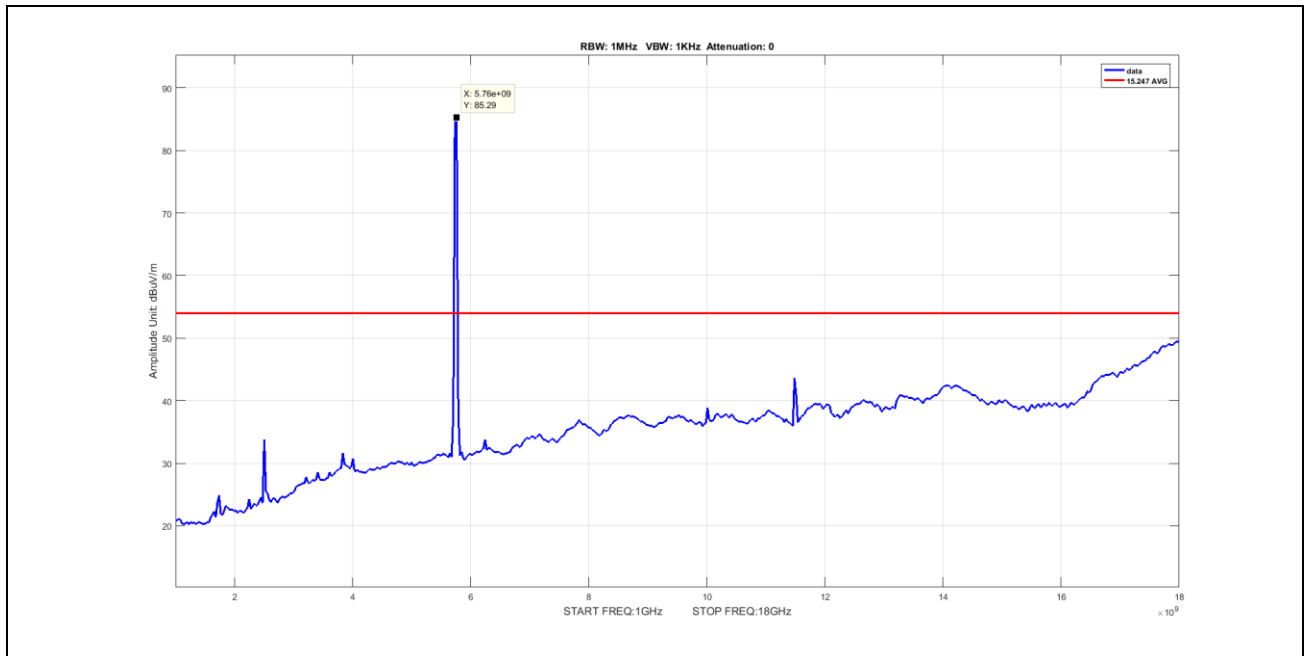
Plot 73. Undesirable Emissions, Average Spurious Emission 1-18GHz, BW 20M, Ch 5745M, A Mode Port 2
