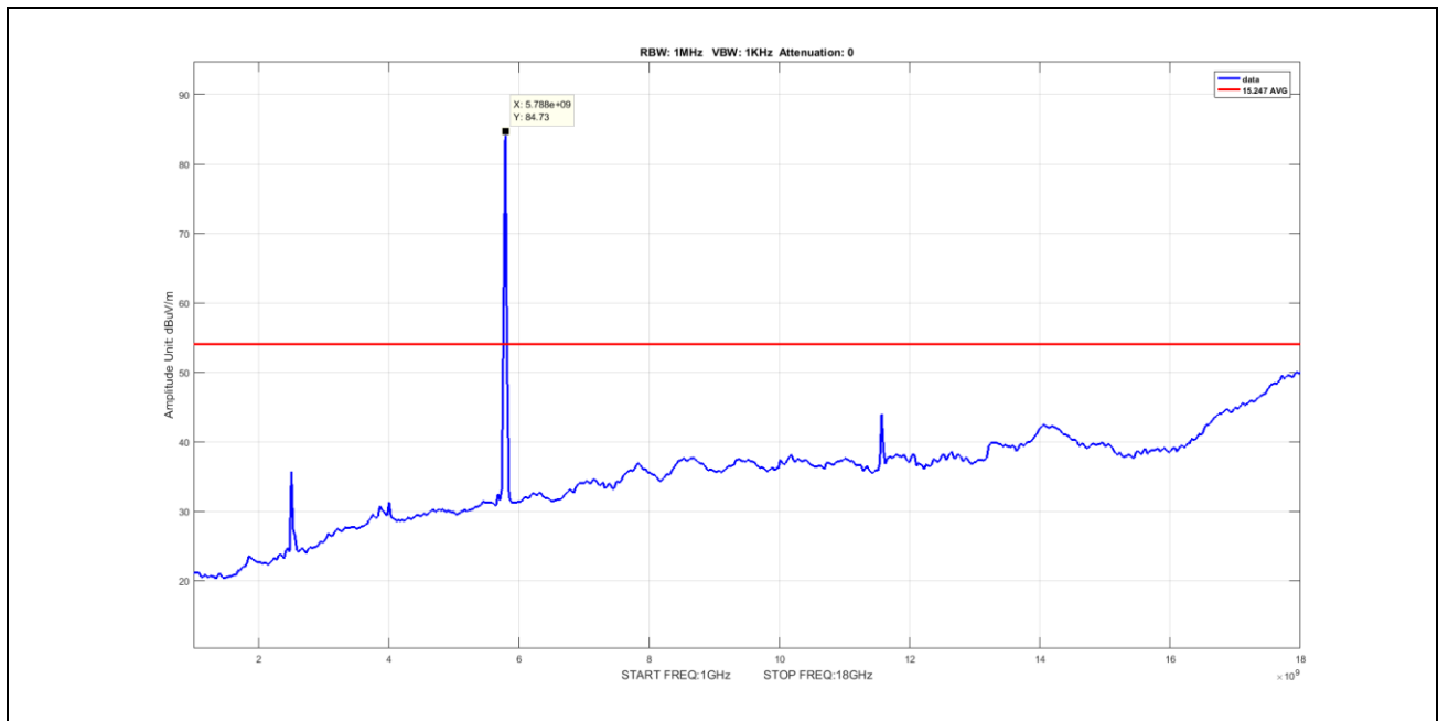
Plot 60. Undesirable Emissions, Average Spurious Emission 1-18GHz, BW 20M, Ch 5785M, N Mode
