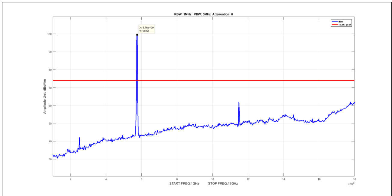
Plot 82. Undesirable Emissions, Peak Spurious Emission 1-18GHz, BW 20M, Ch 5745M, N Mode Port 2
