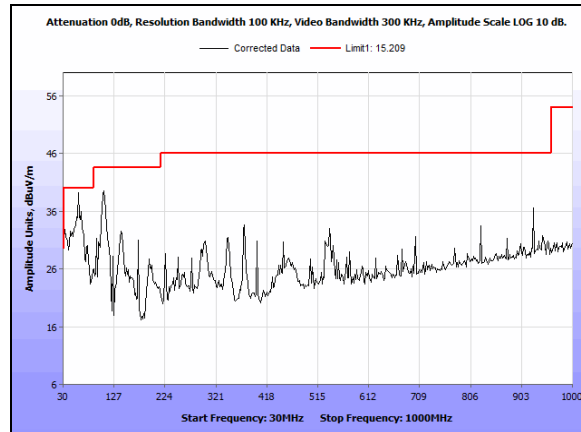
Plot 89. Undesirable Emissions, 30 MHz - 1 GHz 5745 MHz A Mode Port 1
