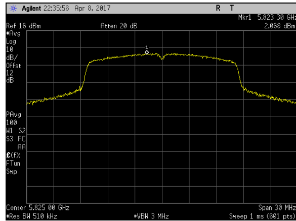
Plot 25. Power Spectral Density, BW 20M, Ch 5825M, A Mode Port 1
