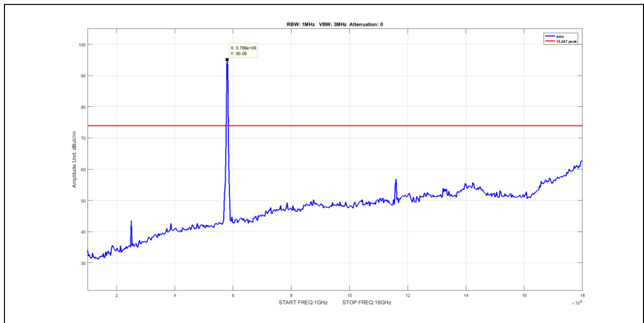
Plot 88. Undesirable Emissions, Peak Spurious Emission 1-18GHz, BW 40M, Ch 5795M, N Mode Port 2
