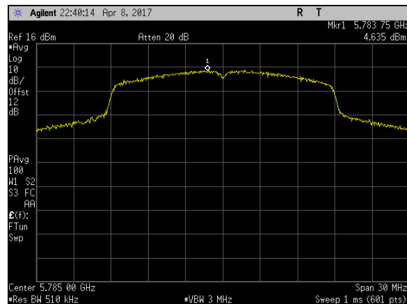
Plot 24. Power Spectral Density, BW 20M, Ch 5785M, N Mode Port 2
