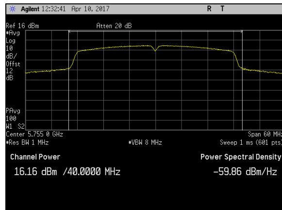
Plot 14. Maximum Conducted Output Power, BW 40M, Ch 5755M, N Mode Port 2
