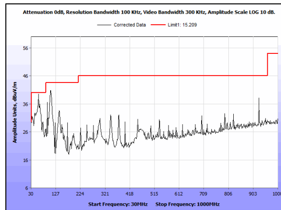
Plot 100. Undesirable Emissions, 30 MHz - 1 GHz 5795 MHz N Mode Port 2
