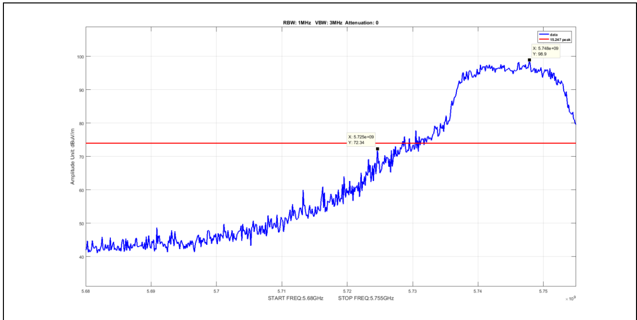
Plot 51. Undesirable Emissions, Peak Band Edge Spurious, BW 20M, Ch 5745M, A Mode
