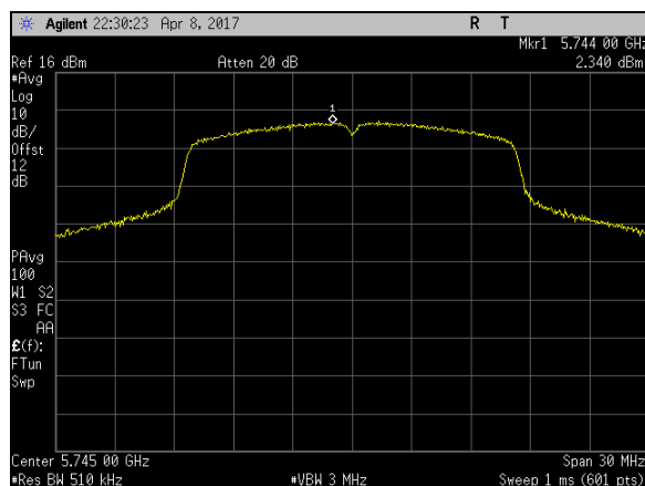
Plot 17. Power Spectral Density, BW 20M, Ch 5745M, A Mode Port 1
