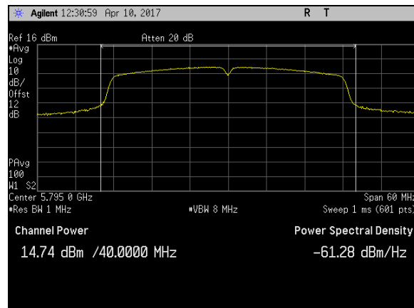
Plot 15. Maximum Conducted Output Power, BW 40M, Ch 5795M, N Mode Port 1
