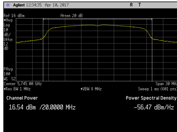
Plot 4. Maximum Conducted Output Power, BW 20M, Ch 5745M, N Mode Port 2
