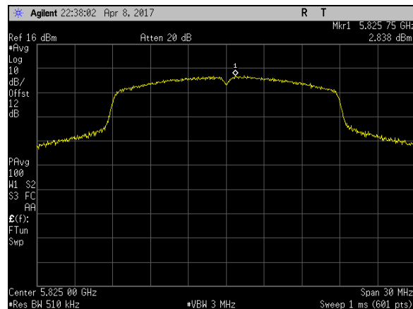
Plot 27. Power Spectral Density, BW 20M, Ch 5825M, N Mode Port 1
