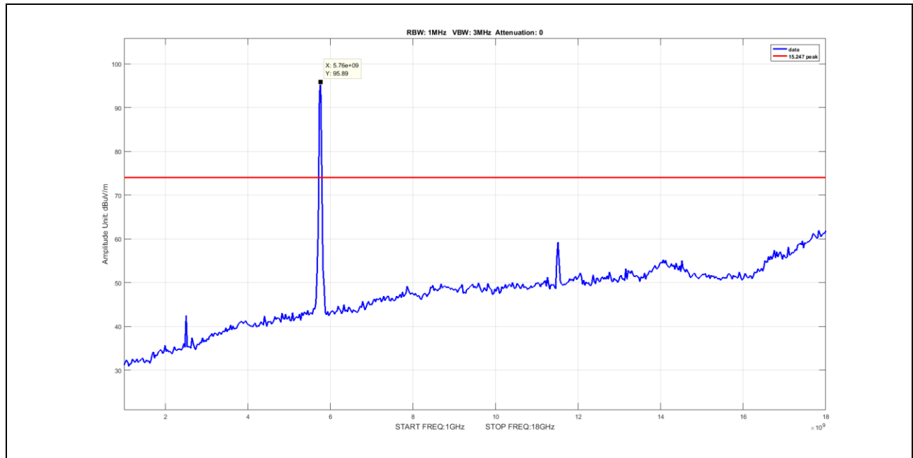
Plot 87. Undesirable Emissions, Peak Spurious Emission 1-18GHz, BW 40M, Ch 5755M, N Mode Port 2
