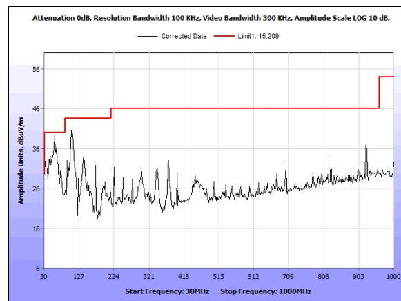
Plot 90. Undesirable Emissions, 30 MHz - 1 GHz 5745 MHz A Mode Port 2
