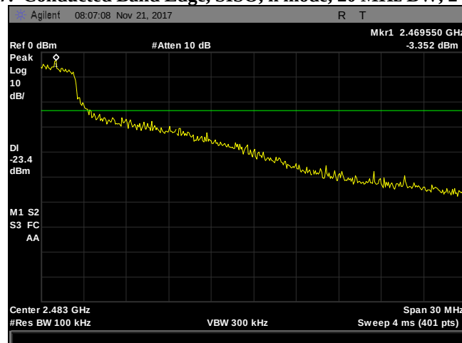
Plot 138. Conducted Band Edge, SISO, n mode, 20 MHz BW, 2462 MHz
