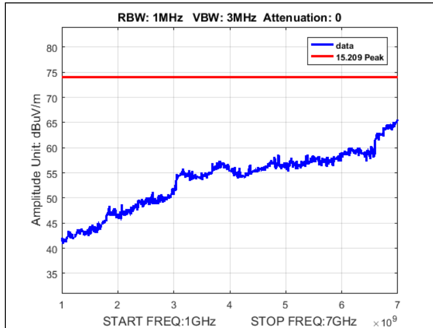
Plot 65. Spurious Radiated Emissions, SISO, Peak Spurious Emission 1-7GHz, BW 20M, Ch 2437M, B Mode
