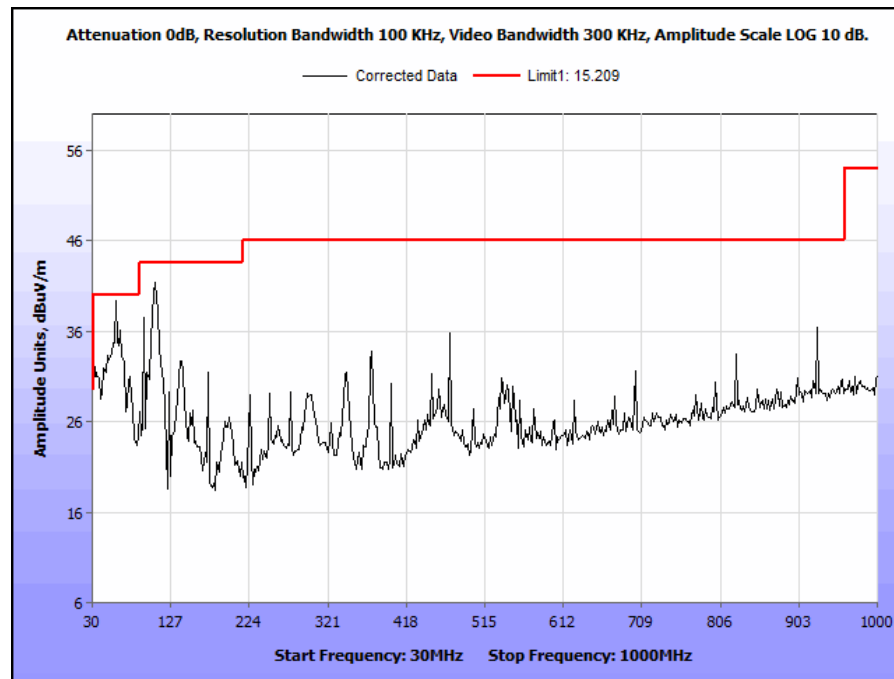
Plot 37. Spurious Radiated Emissions, SISO, 30 MHz - 1 GHz, n mode, 40MHzBW, mid
