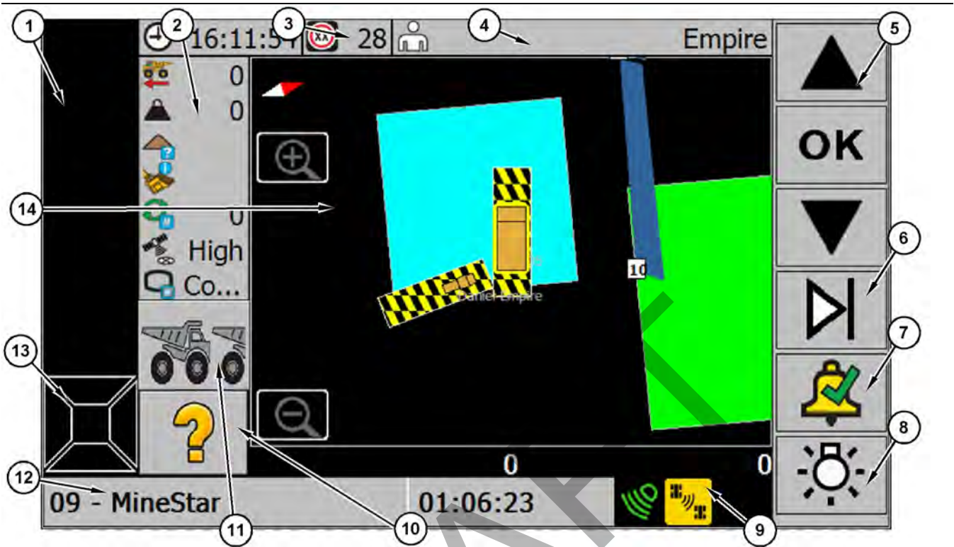
Illustration 6 (1) Object Detection Proximity Bar (2) System Information (3) Speed Limit (4) Operator Name (5) Soft Button Panel including Up and Down Arrows, and OK buttons (6) Soft Panel Next Screen button (7) Soft Panel Alarm Acknowledge button (8) Soft Panel Brightness button (9) System Status and Warning (10) Tool Bar Button Menu (11) Truck State (12) Status Window (13) Object Detection Quadrant Detection (14) Map View
