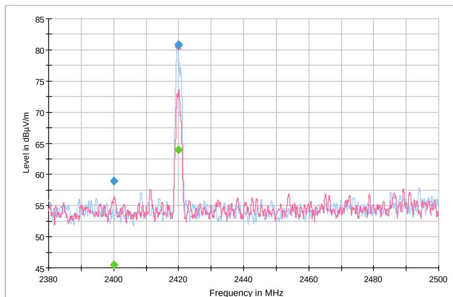
Lower bandedge (Rotor)
