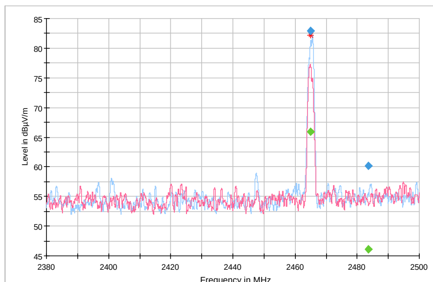
Higher bandedge (Rotor)
