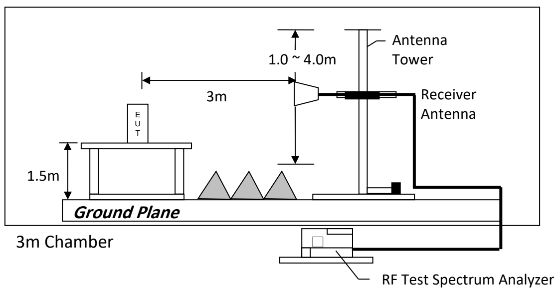
Test setup of radiated emissions above 1GHz
