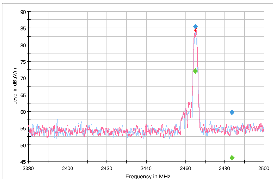
Higher bandedge (Stator)
