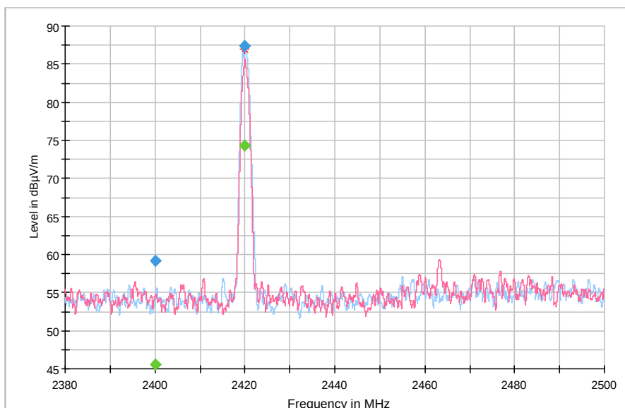
Lower bandedge (Stator)
