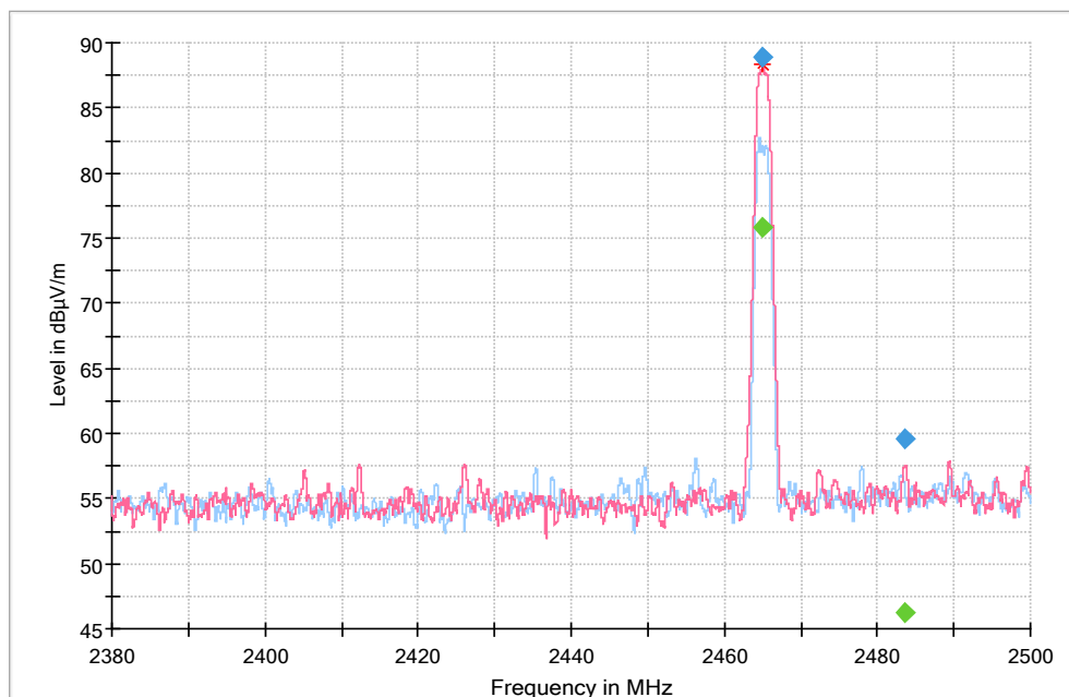
Higher bandedge (Stator)
