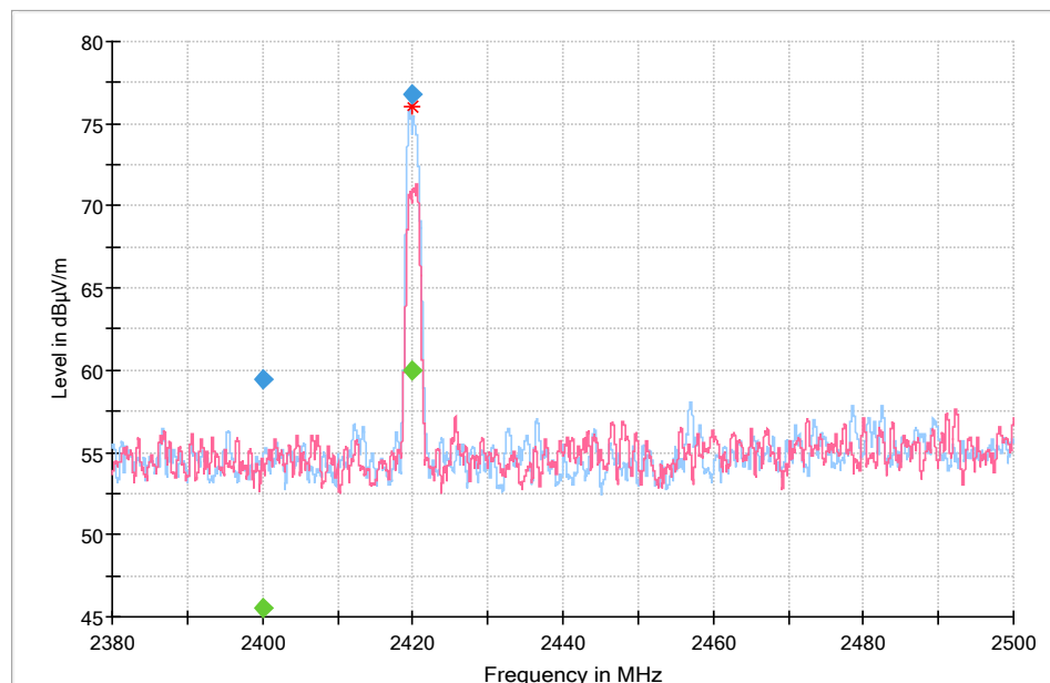
Lower bandedge (Rotor)
