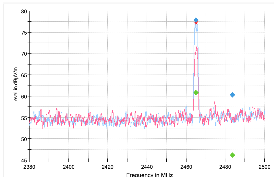
Higher bandedge (Rotor)
