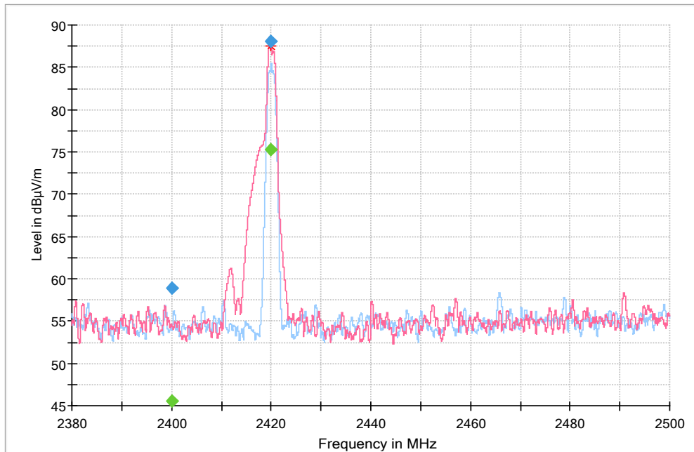
Lower bandedge (Stator)
