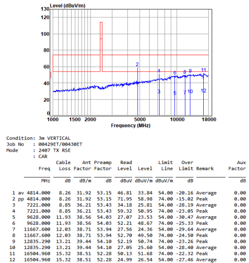
2.4G_SRD_LOW_TX_Vertical
