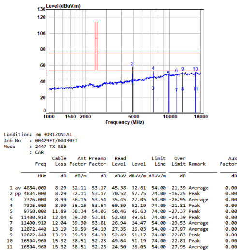
2.4G_SRD_MID_TX_Horizontal
