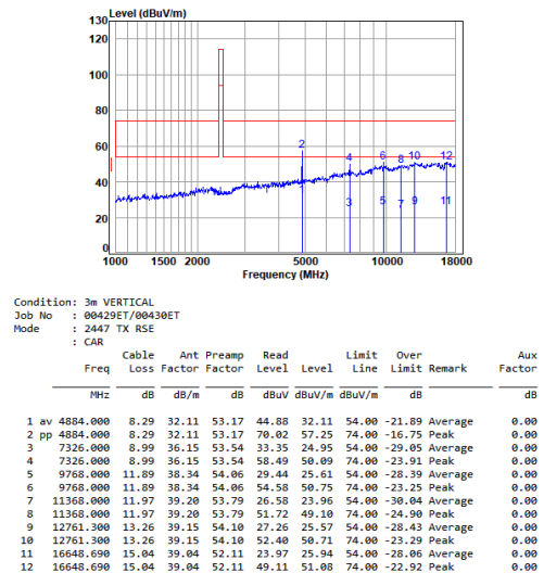
2.4G_SRD_MID_TX_Vertical
