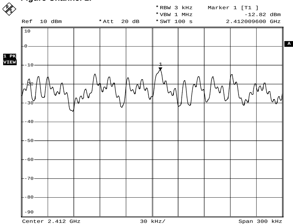
Figure Channel 1:
