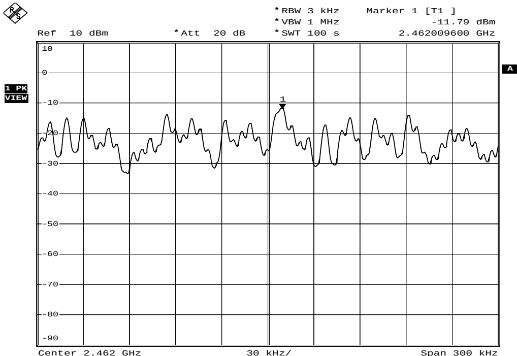
Figure Channel 11:
