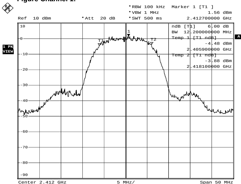
Figure Channel 1:
