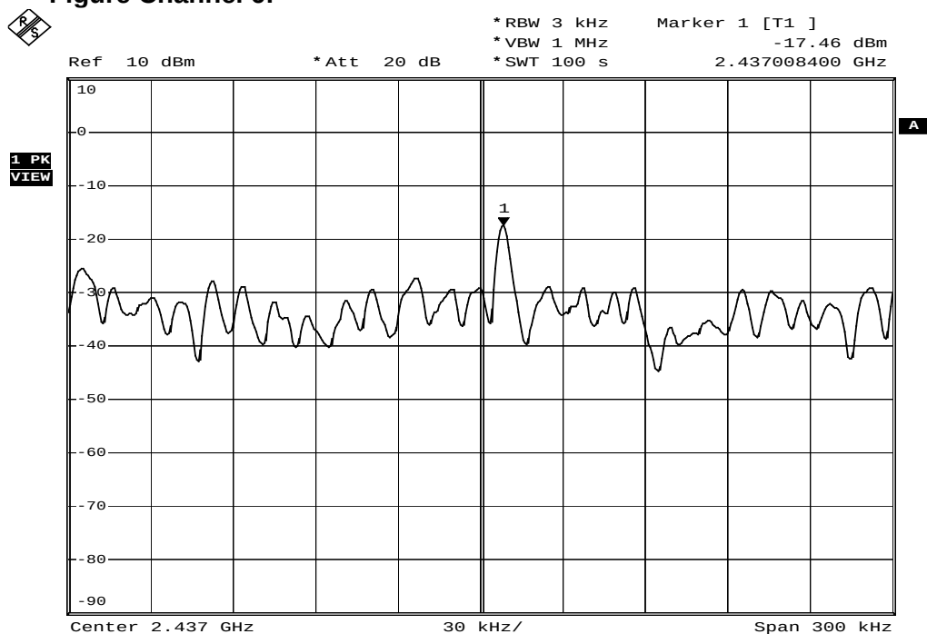
Figure Channel 6:
