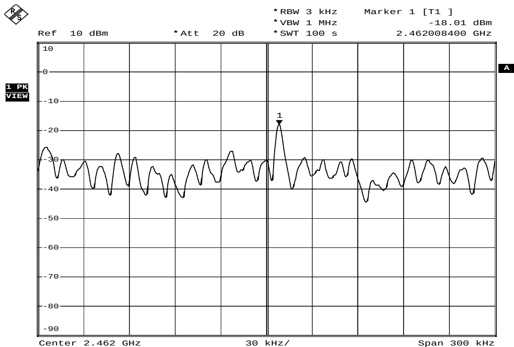
Figure Channel 11:
