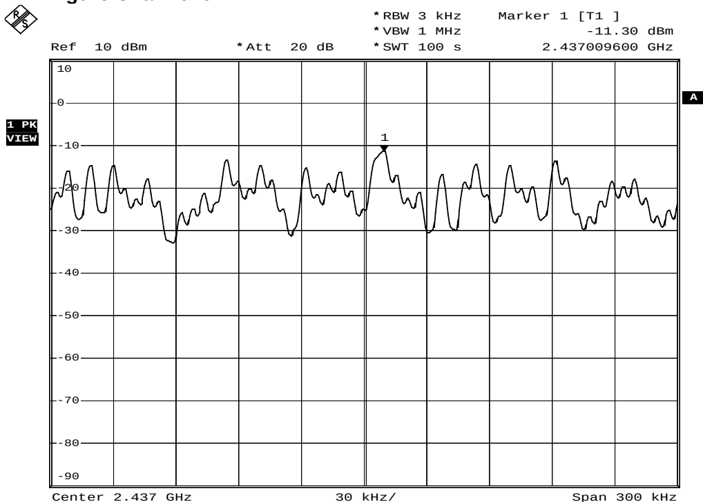
Figure Channel 6:
