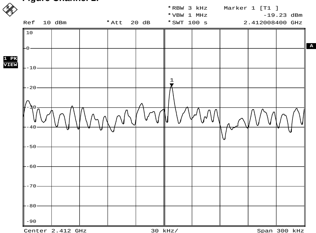
Figure Channel 1:
