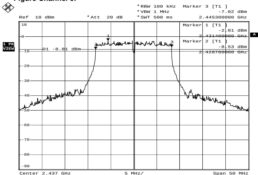
Figure Channel 6:
