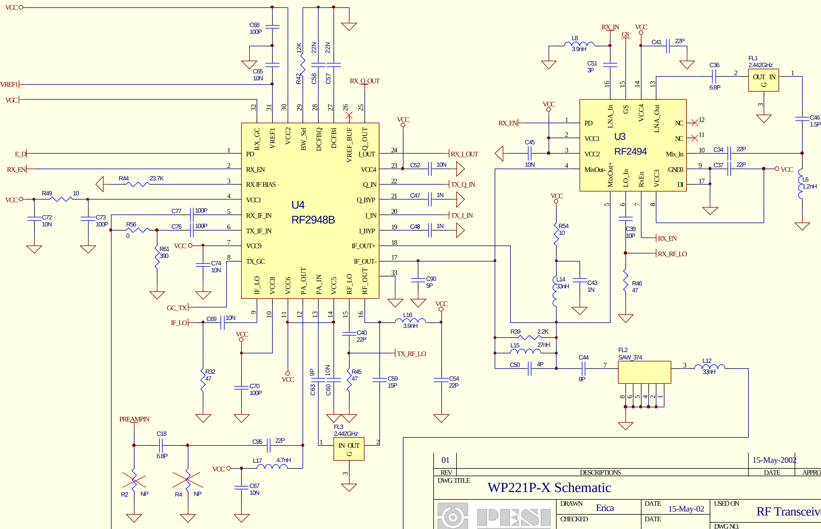
RF Transeiver Stage
