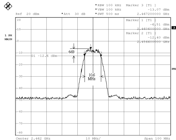
Channel 11:
