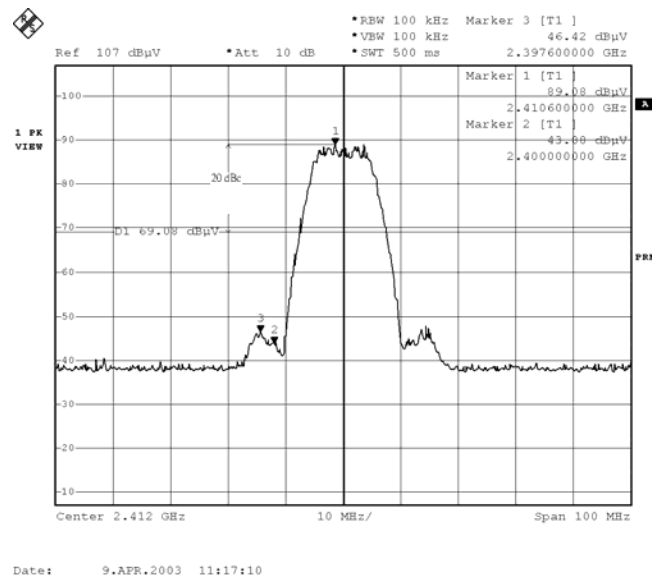
Figure Channel 1: (Vertical)
