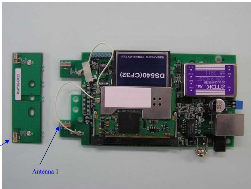
Wireless LAN Mini PCI Car with the main board
