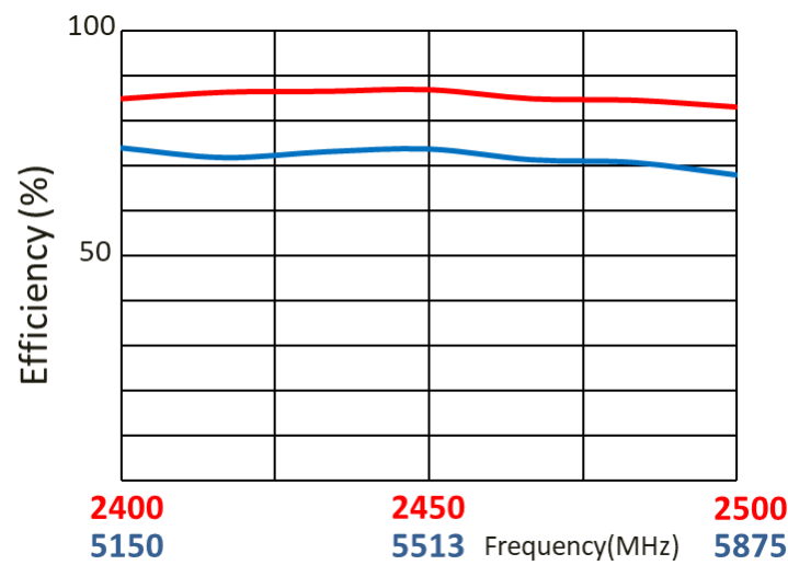
Efficiency
